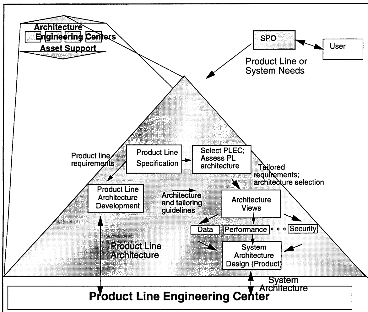
Figure 3: Architecture Tasks
