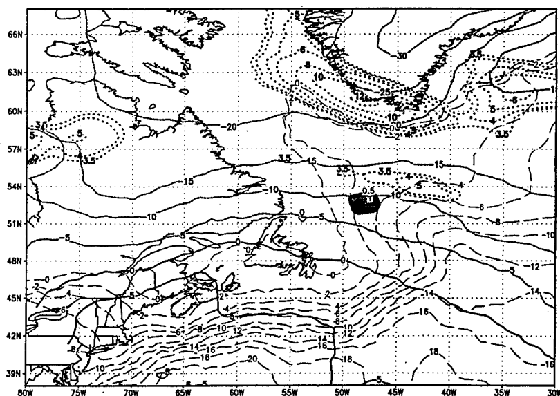
Figure 4.24: Initial 760\text{ hPa} temperature (heavy solid contours, ^{\circ}\text{C} ) and sea-surface temperature (long dashed contours, ^{\circ}\text{C} ) at 00UTC 20 January 1995. Shaded region near 53^{\circ}\text{N} , 48^{\circ}\text{W} indicates area of 1^{\circ}\text{C} initial temperature perturbation P1 used in MAMS1 forecasts shown in Figs. 4.25-4.28. Dotted contours correspond to initial cyclonic vorticity ( 10^{-5}\text{ s}^{-1} ) at 760\text{ hPa} .
