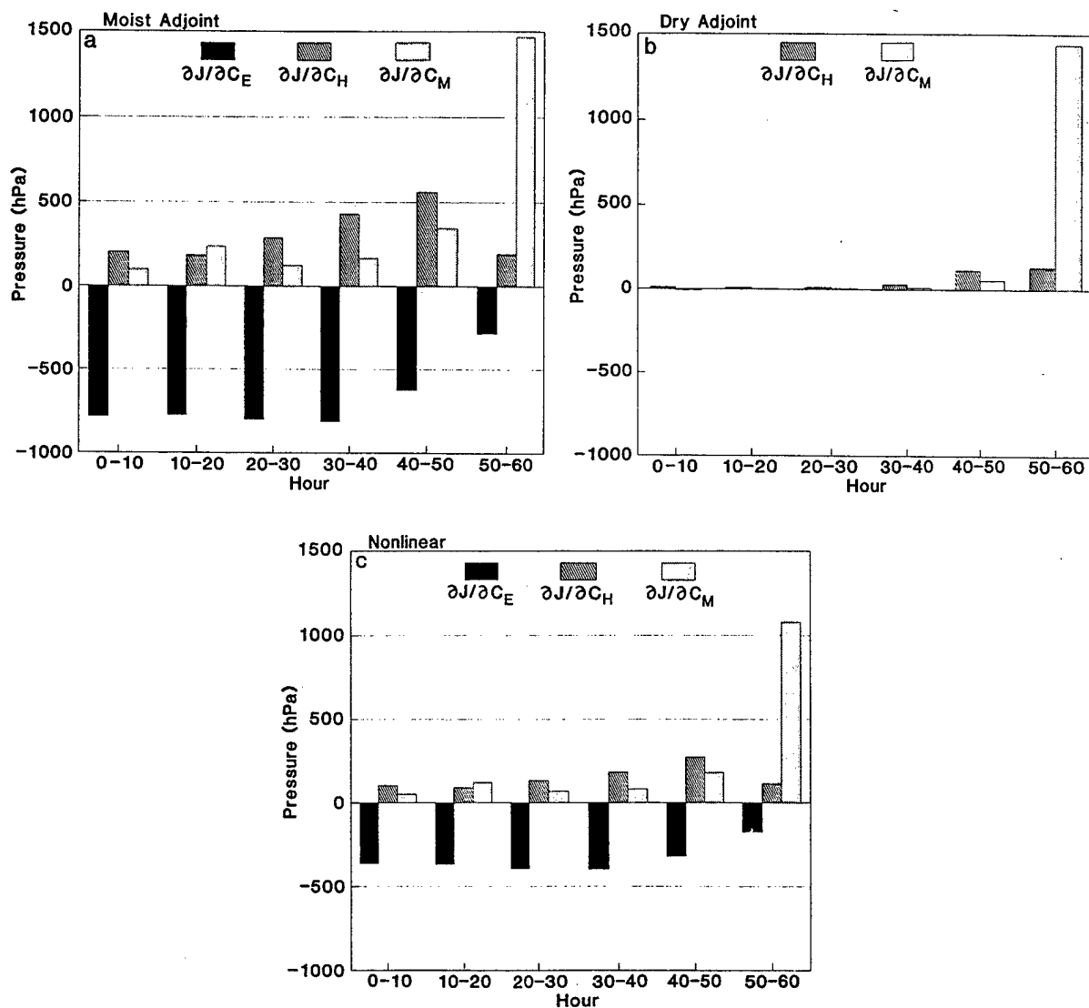
Figure 3.32: Histograms of (a) accumulated adjoint sensitivity for perturbations of surface transfer coefficients, \partial J/\partial C_E (latent heat flux), \partial J/\partial C_H (sensible heat flux), and \partial J/\partial C_M (momentum stress) over entire model domain; (b), as in (a), using dry adjoint model. Effect on 60 h cyclone central pressure ( J ) is a dot product of a perturbation of C_E , C_H , or C_M and this sensitivity; (c) Nonlinear sensitivity obtained from difference between non-perturbed integrations and nonlinear integrations with surface transfer coefficients increased by 0.5 \times 10^{-3} over entire model domain. Moist simulations (a, c) include convective and nonconvective precipitation. Forecast aspect J is pressure at center of 60 h cyclone.
