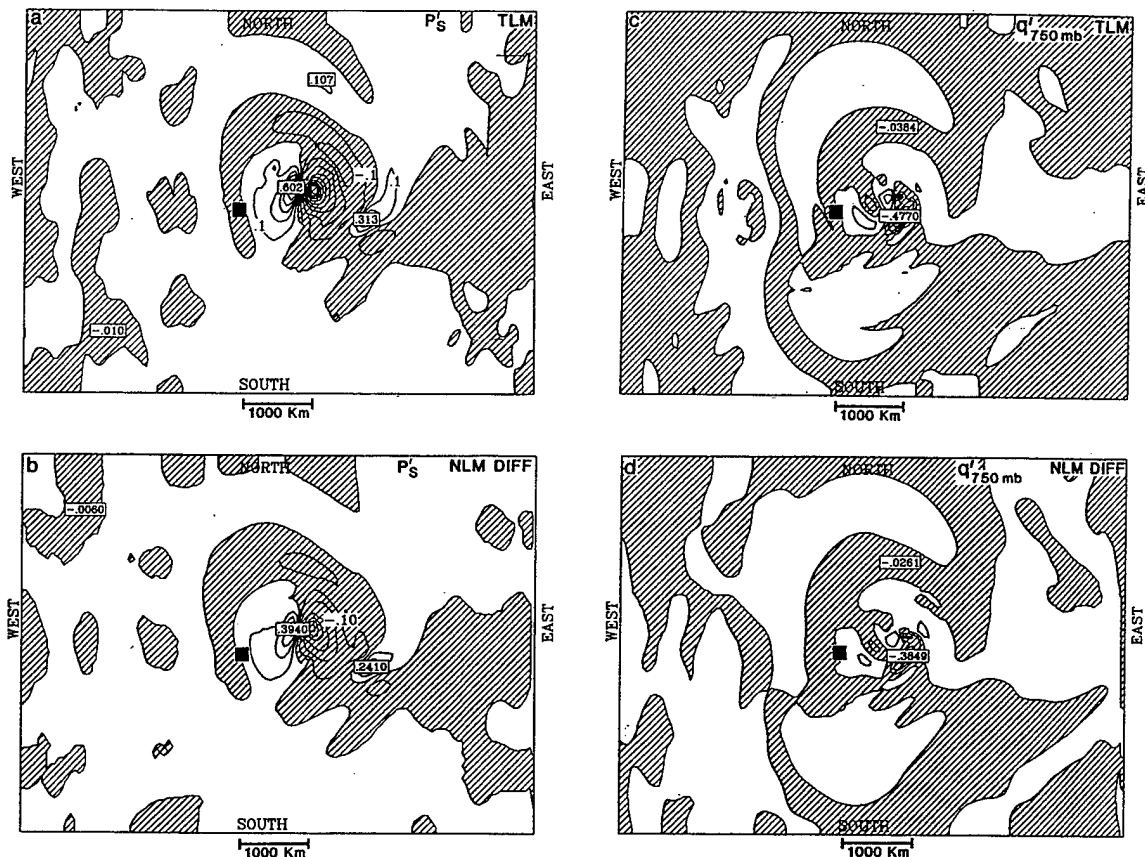
Figure 3.24: (a) 20 h forecast of TLM surface pressure perturbations (contour = 0.1 hPa) resulting from perturbation of mixing ratio (+ 1 g kg -1 ) at nine grid points on model level near 760 hPa at 40 h. (b) As in (a), except difference between perturbed and non-perturbed nonlinear integrations. (c) 20 hour forecast of TLM mixing ratio perturbations (contour = 0.1 g kg -1 ) near 760 hPa resulting from initial perturbation as in (a). (d) As in (c), except difference between perturbed and non-perturbed nonlinear integrations. Simulations include convective and nonconvective precipitation. Negative values are shaded. Solid square indicates location of perturbation at 40 h.
