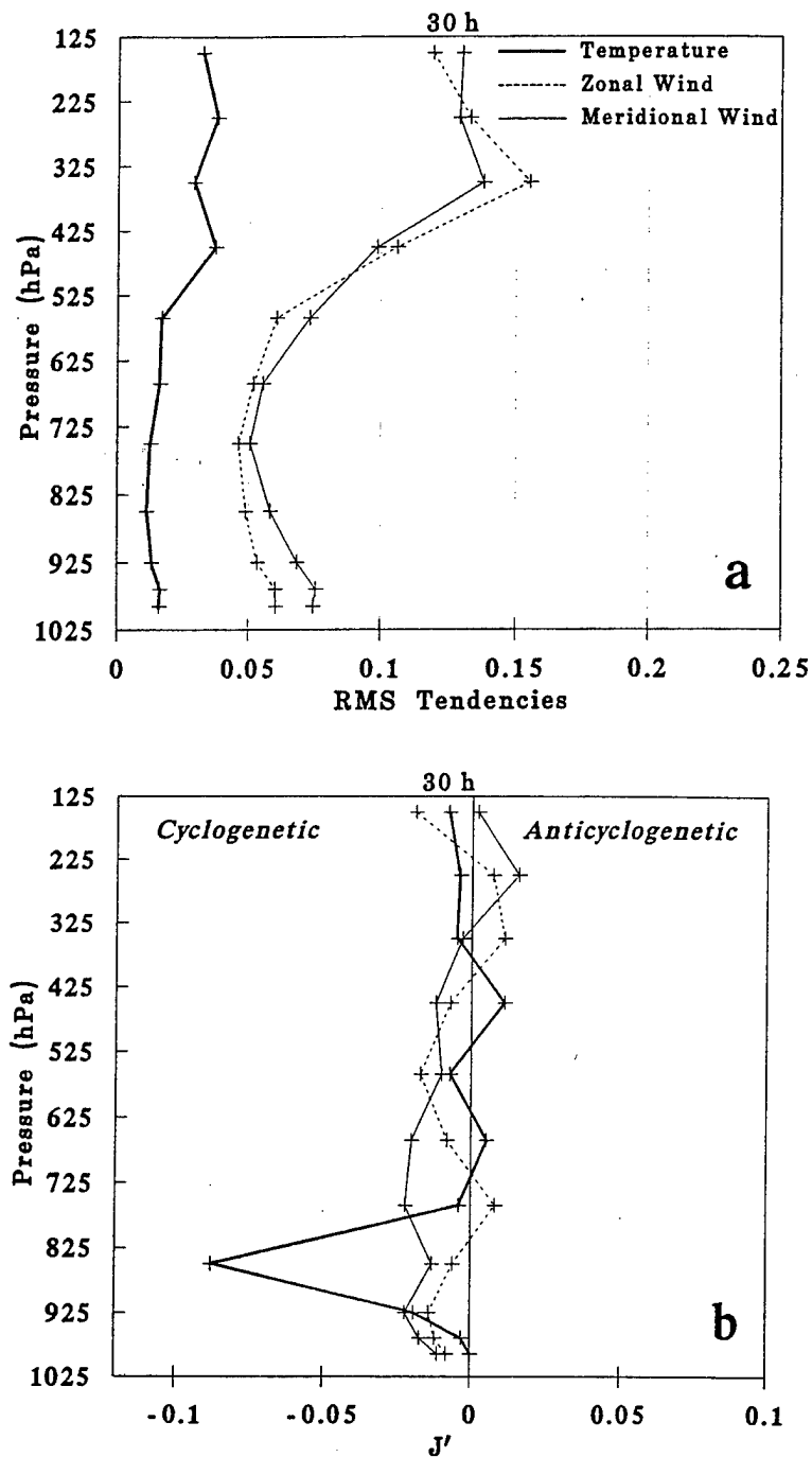
Figure 3.11: (a) Root mean square (on sigma levels) of nonlinear model tendencies of zonal and meridional wind ( \text{m s}^{-1} \text{h}^{-1} ) and temperature ( \text{K h}^{-1} ) obtained as a two-hour difference centered at 30 h; (b) Dot product of perturbations (one-hour wind or temperature adjustment) and 30 h adjoint sensitivity, summed on sigma levels. Units of J' are hPa, negative values indicate an increase in nonlinear tendency produces a negative pressure perturbation ( J' ) at center of 90 h cyclone. Crosses correspond to model levels.
