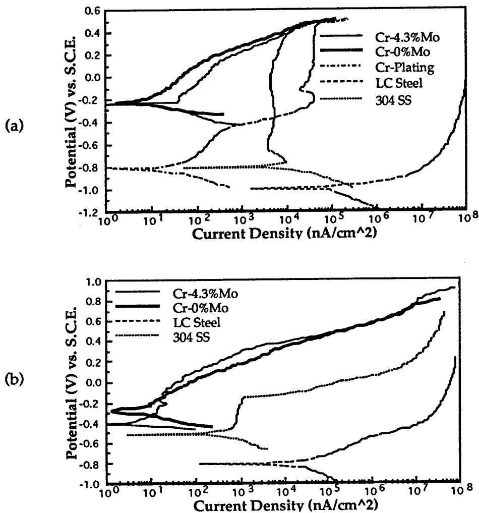
Fig. 13. Results of the corrosion tests for the IBED treated samples and a number of substrates substrates in (a): sulfuric acid (b): sodium chloride.
