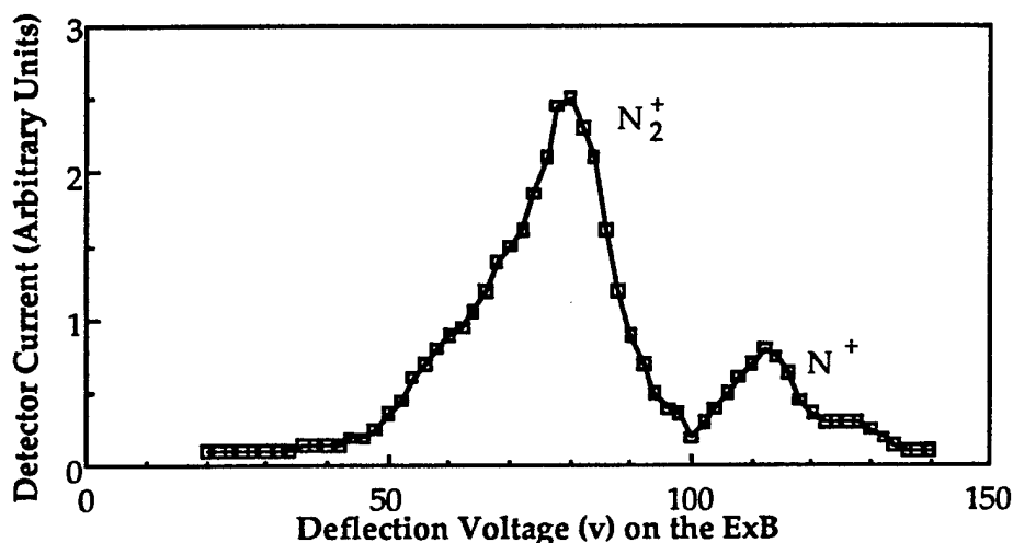
Fig. 4. Ion mass spectra in a nitrogen plasma under certain processing conditions: N_2^+=75.7\% and N^+=24.2\% have been measured in this case.
