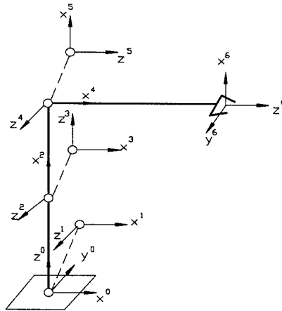
Figure 2.4 Coordinate frames of a linkage robot
