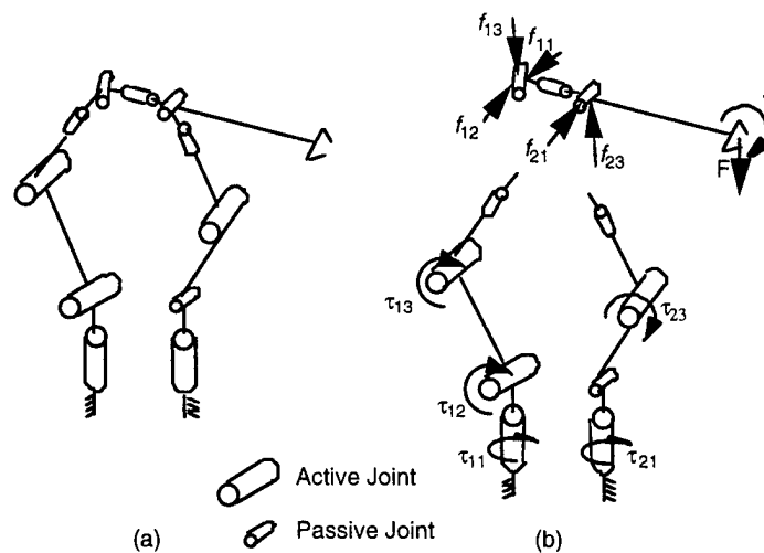
Figure 4.3 The free body diagram of a linkage robot
