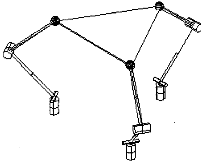
Figure 2.5 A three articulated-arm platform robot
