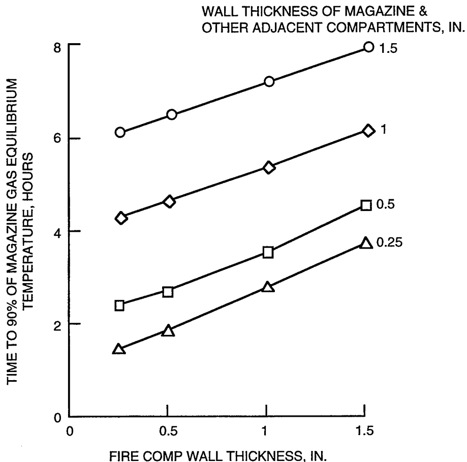
FIGURE 11. Time Response of Magazine Gas Versus Wall Thickness.
