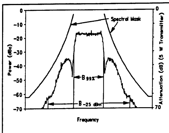
Figure A-7. 1000 kbps RNRZ PCM/FM signal and spectral mask (frequency span = 5 MHz).
