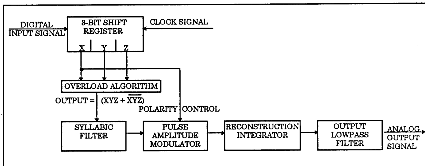
Figure F-1b. Typical CVSD decoder.
