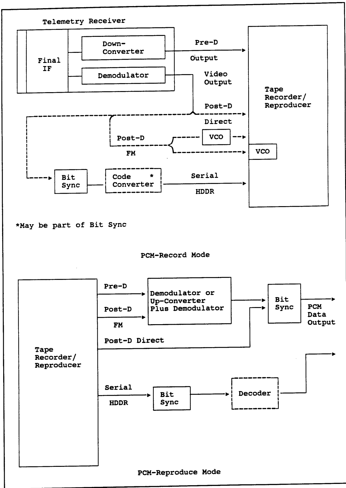
Figure 6-4. PCM record and reproduce configuration.
