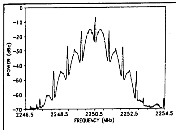
Figure A-4. Biφ PCM/PM signal.
