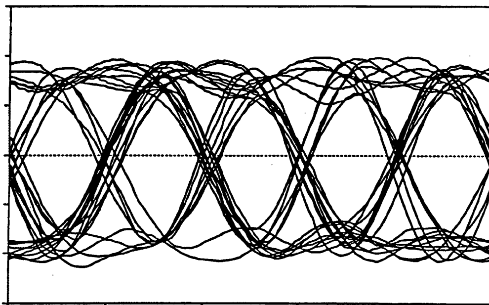
b. RNRZ-L at bit packing density of 25 kb/in.
