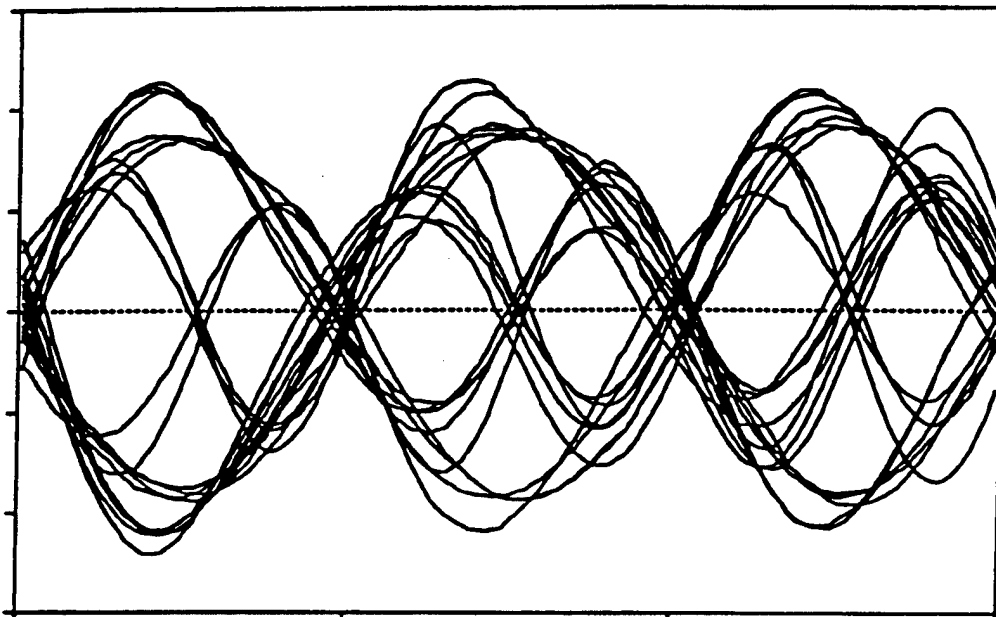
a. Biφ-L at bit packing density of 15 kb/in.
