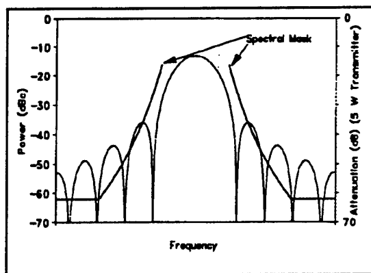
Figure A-9. 1000 kbps OQPSK signal (sinusoidal weighting) and spectral mask.
