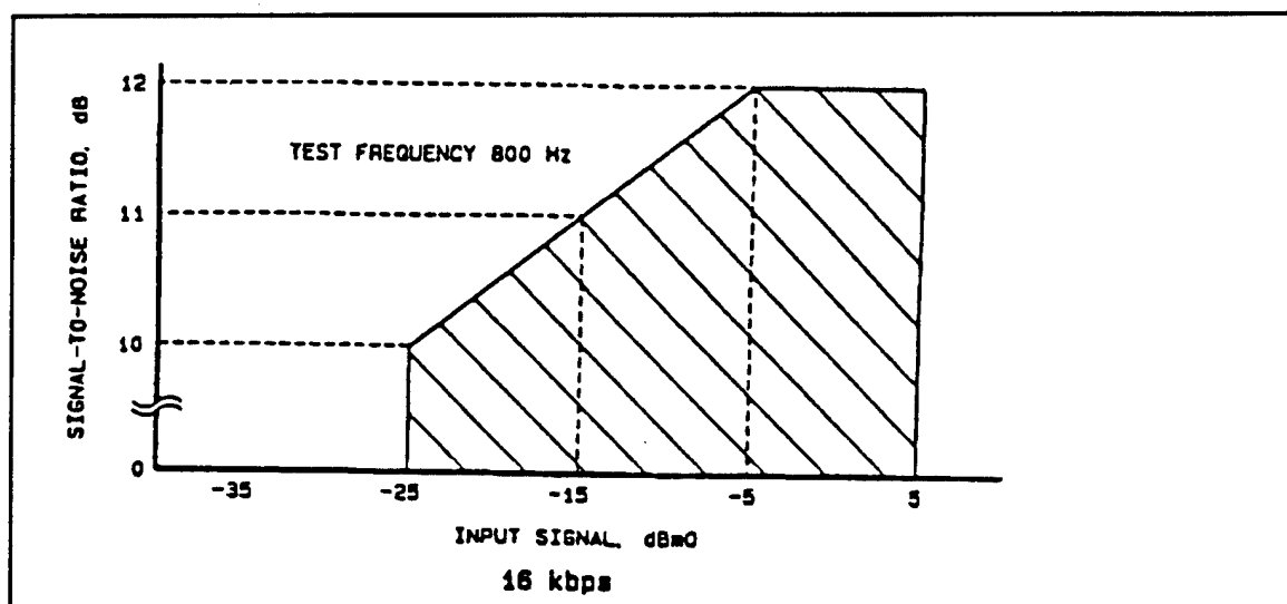
Figure F-6a. Signal to quantizing noise ratio versus input level for CVSD.
