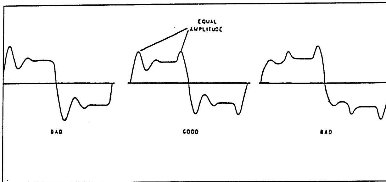
Figure D-7. Square wave responses.
