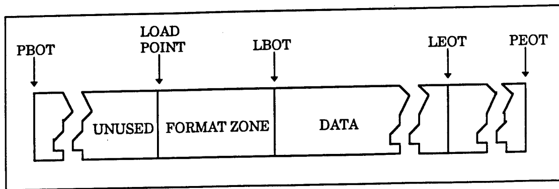
Figure 6-13. Tape cartridge layout.
