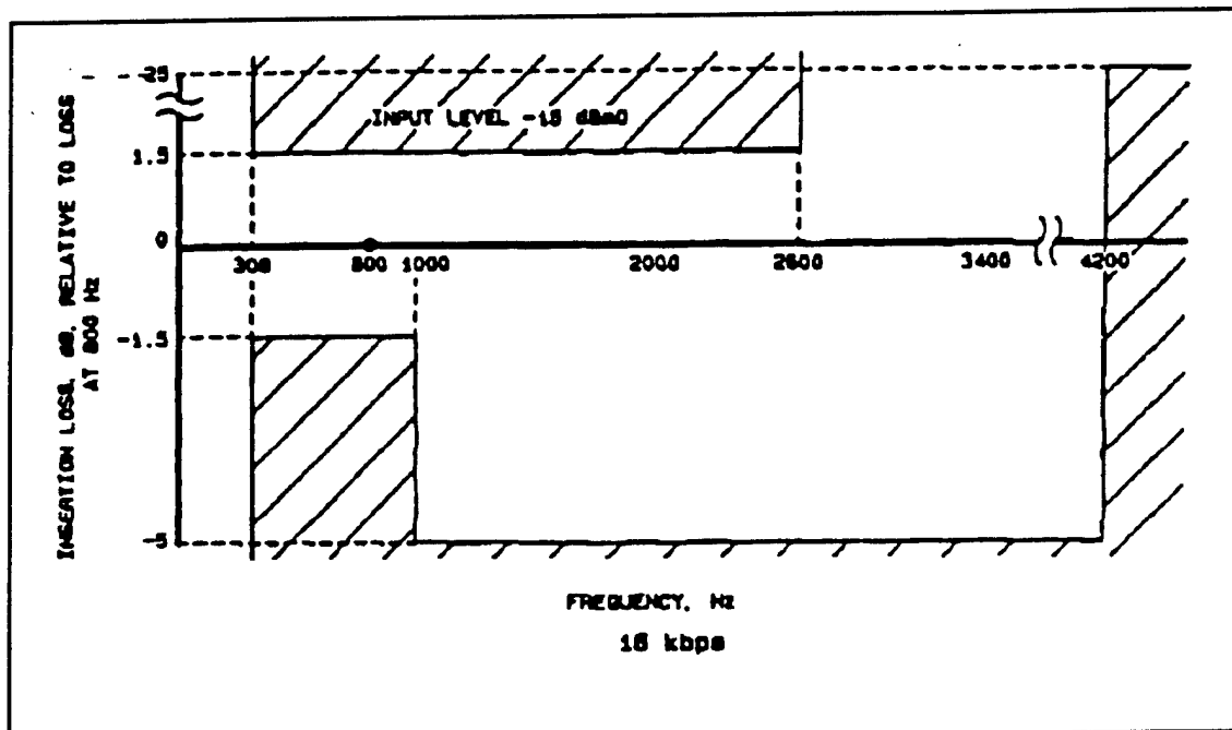
Figure F-4a. Insertion loss versus frequency for CVSD.
