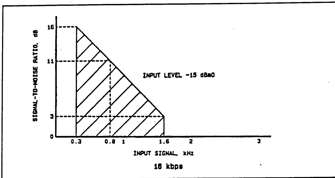
Figure F-7a. Signal to quantizing noise ratio versus frequency for CVSD.
