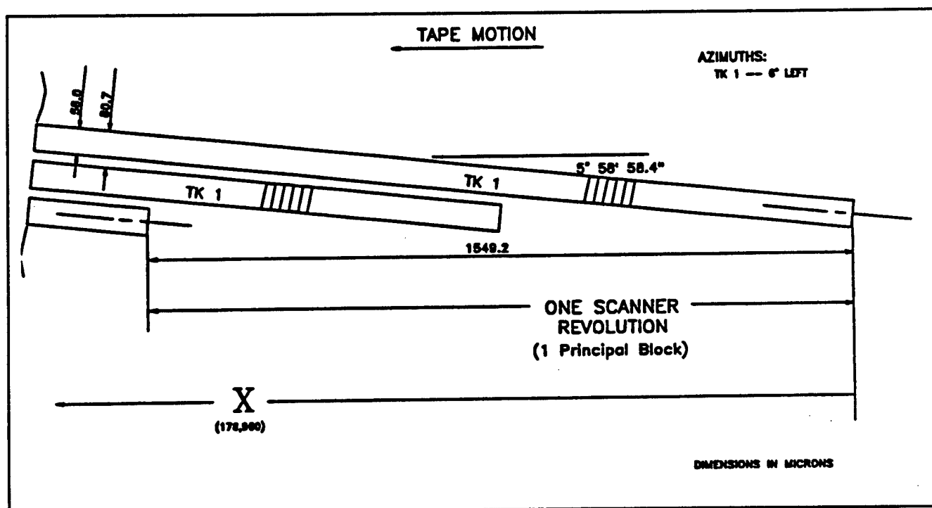
Figure 6-11. Helical track dimensions, E format.
