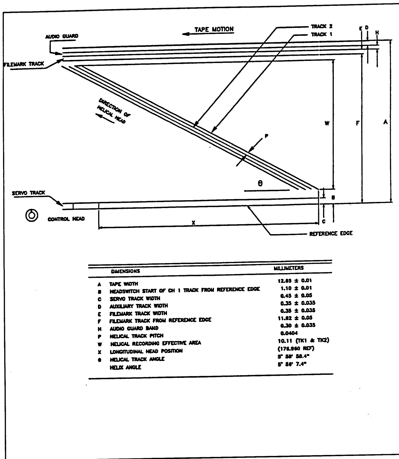
Figure 6-12. Recorded tracks on tape, B format.
