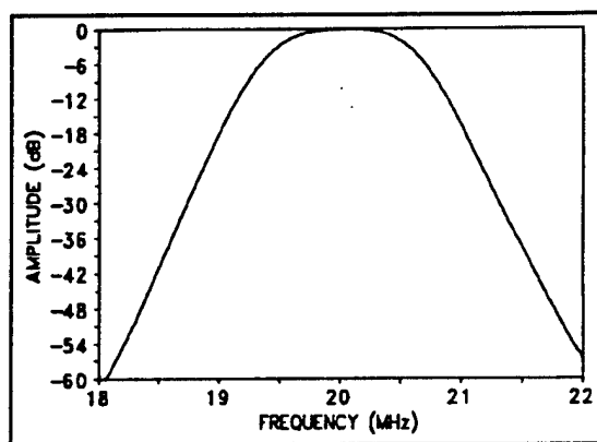
Figure A-6. Typical receiver IF filter response (-3 dB bandwidth = 1 MHz).
