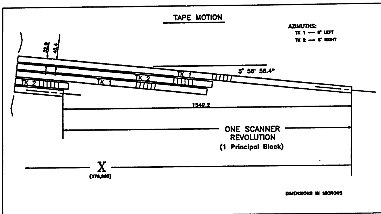
Figure 6-10. Helical track dimensions, B format.
