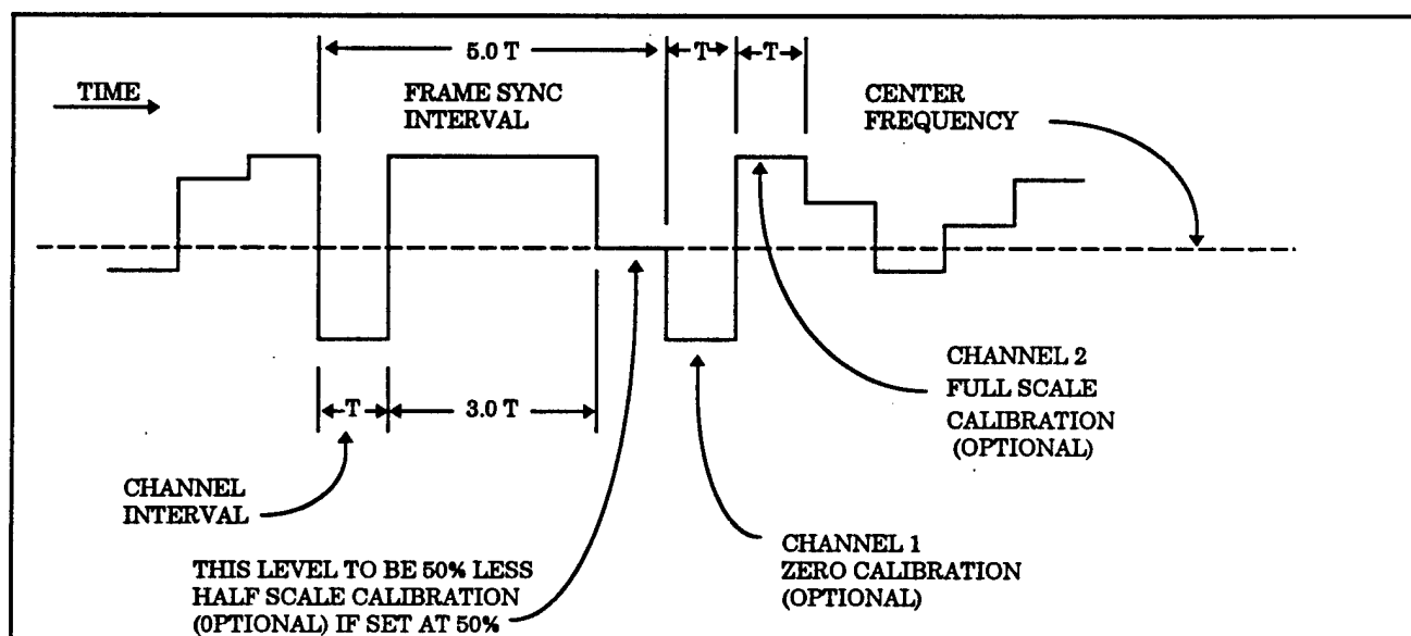
Figure K-2. 100-percent duty cycle PAM with amplitude synchronization.
