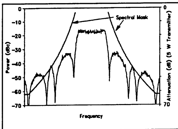
Figure A-8. Unfiltered 1000 kbps RNRZ PCM/FM signal and spectral mask.
