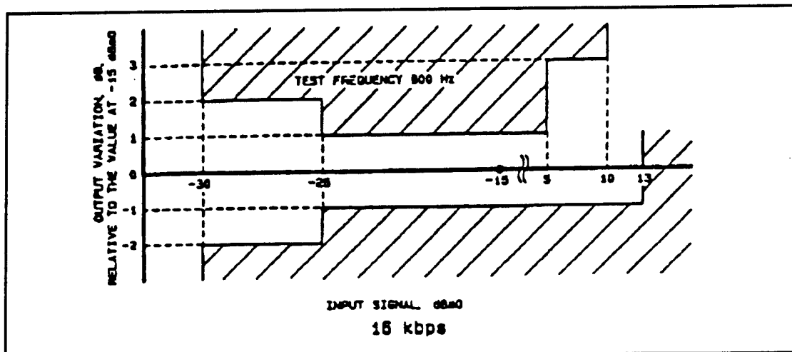
Figure F-5a. Variation of gain with input level for CVSD.
