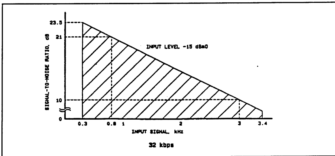
Figure F-7b. Signal to quantizing noise ratio versus frequency for CVSD.
