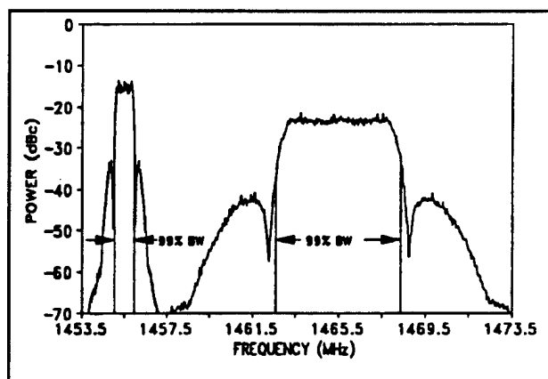
Figure A-1. 800 kbps and 5 Mbps RNRZ PCM/FM signals.
