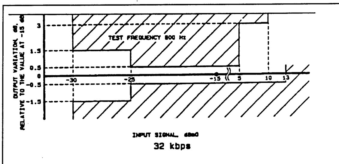
Figure F-5b. Variation of gain with input level for CVSD.
