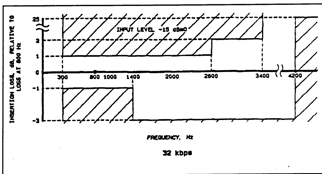
Figure F-4b. Insertion loss versus frequency for CVSD.
