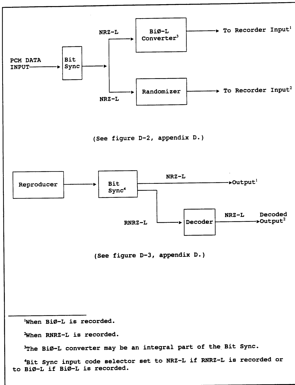
Figure 6-5. Serial high density digital record and reproduce.
