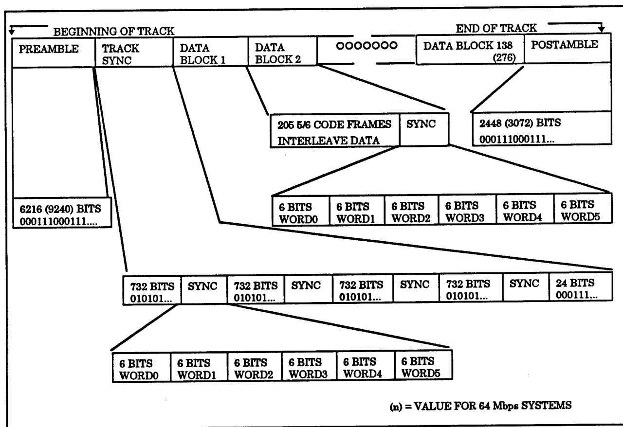
Figure 6-14. Helical track format.
