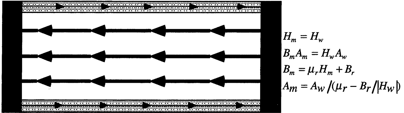
Figure 2: Configuration of Supply Magnet and Pole Pieces in the Workspace
