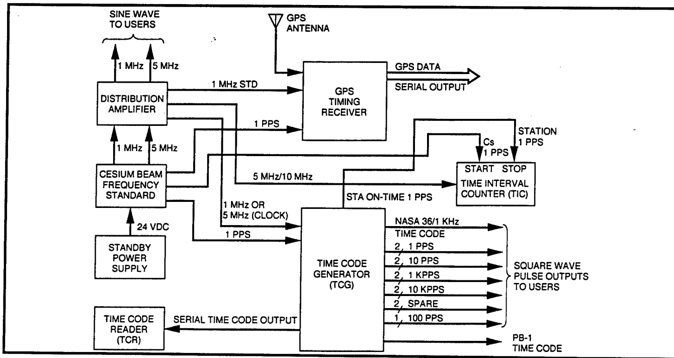
Figure 16-1. Timing equipment.
