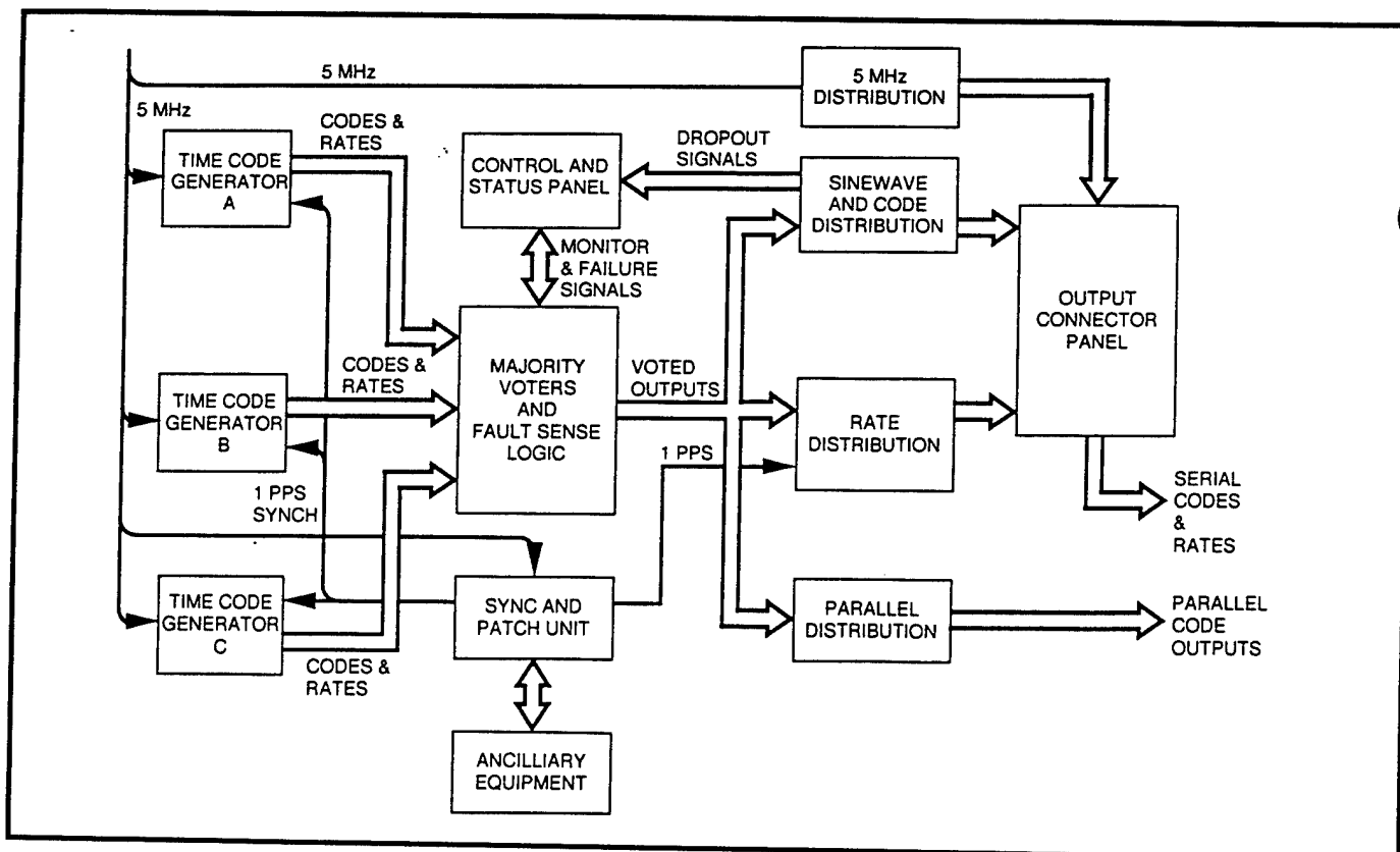
Figure 16-4. TRAK 8407 triple redundant clock.
