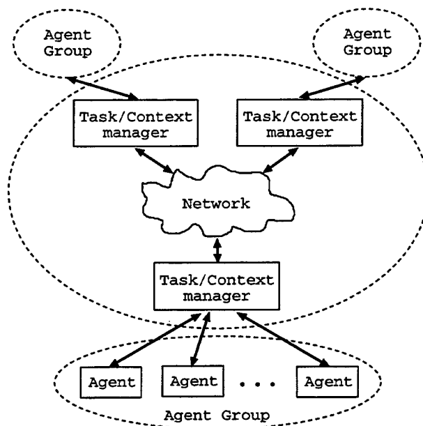
Figure 3: Interconnected network of TCMs.
