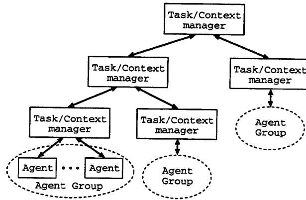
Figure 2: Hierarchical network of TCMs.
