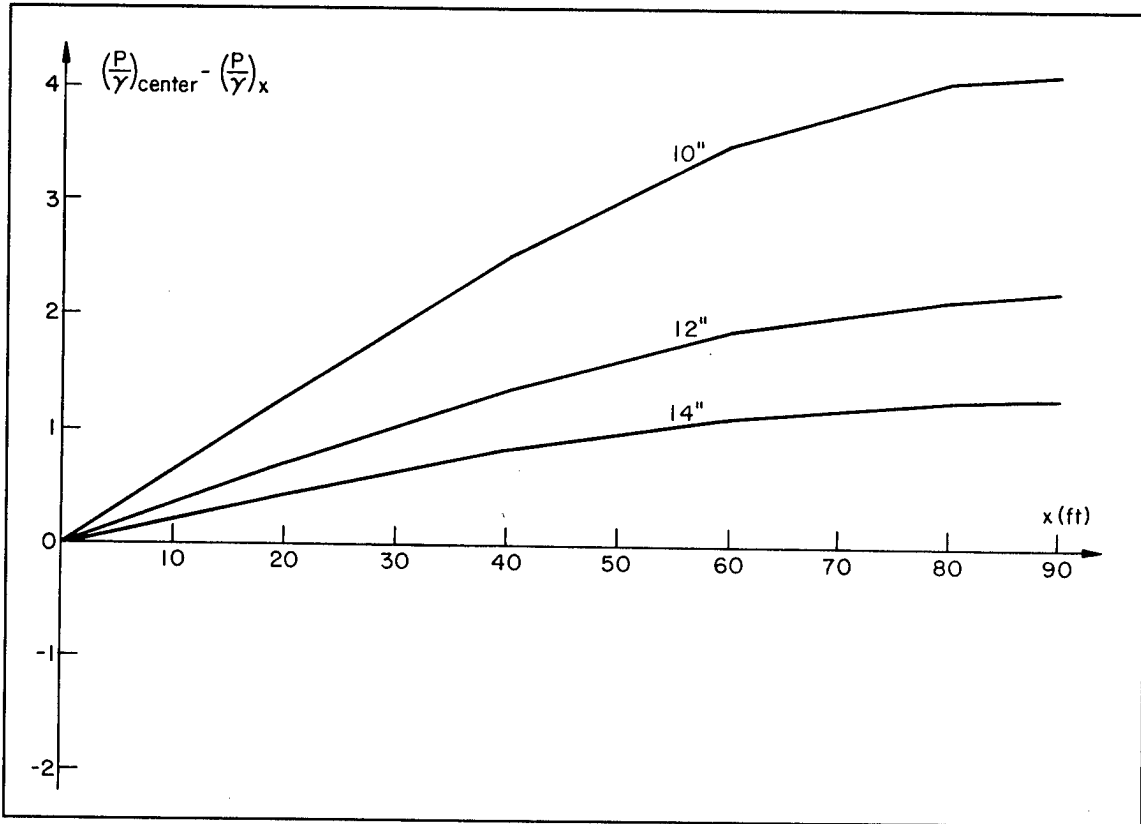
Figure A3. Variation of pressure head from center-feed pressure head inside and along fluidization pipe, Example 2
