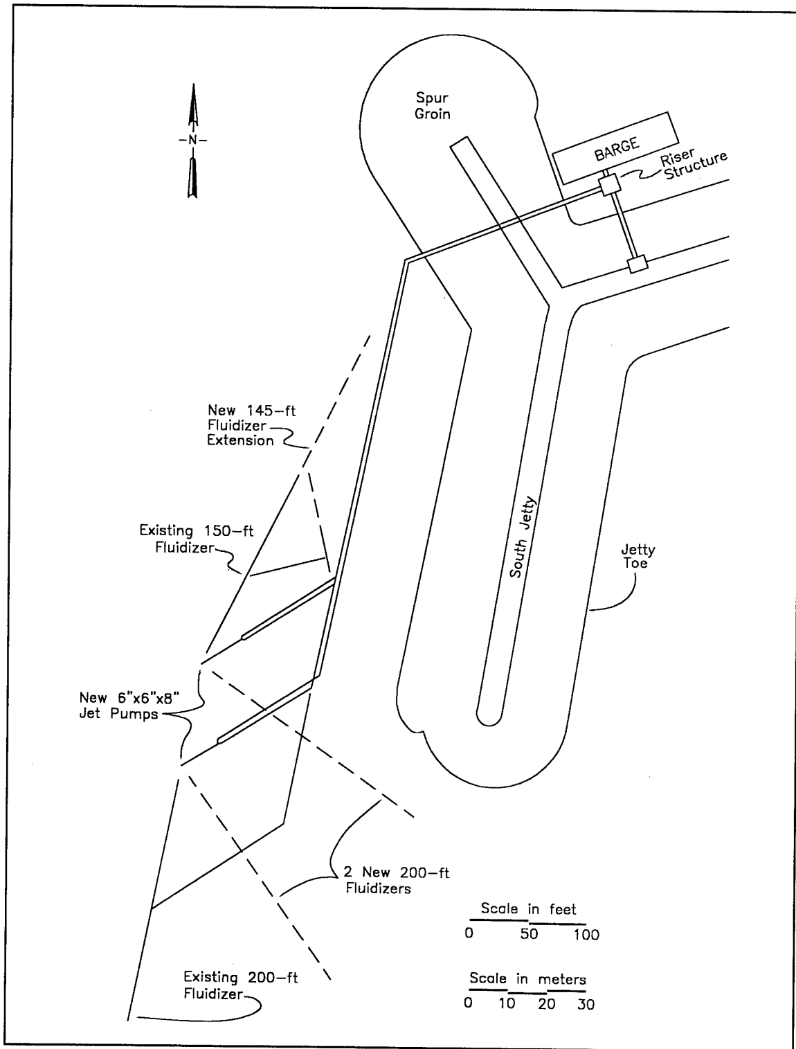
Figure B11. Planned modifications for Phase III of the Oceanside Sand Bypass System (after Moffatt and Nichol Engineers (1994))
