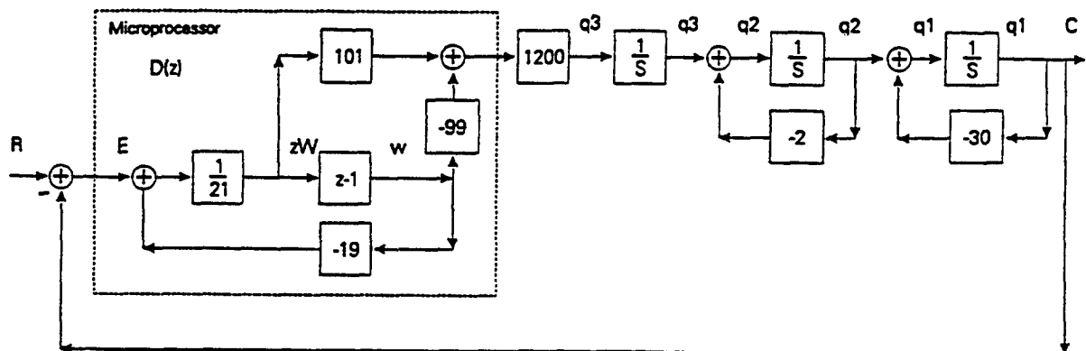
Figure 2-11. Discrete-time closed-loop control system with a gain of 1200.
