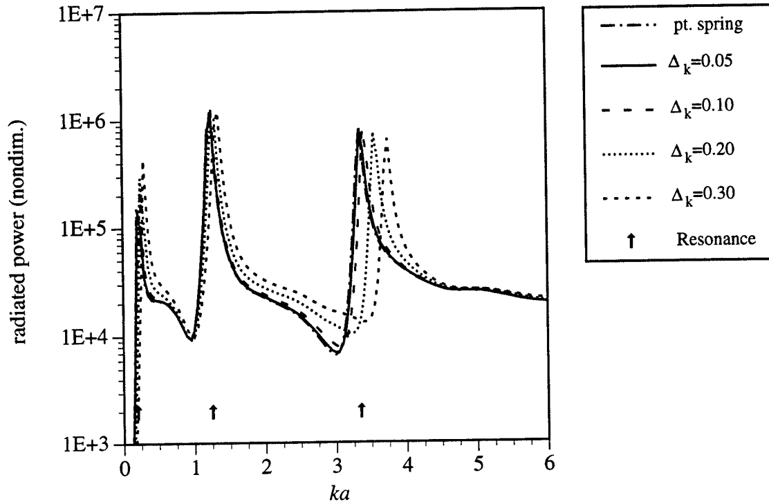
Figure 11. Radiated acoustic power for a lumped element and various distribution widths, \Delta_k \cdot k_{rat} = 2860 .
