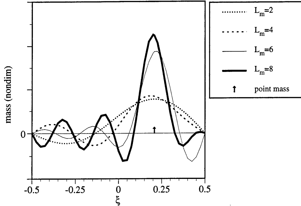
Figure 4. Example mass distribution for finite series. One mass of 0.25 at \xi = 0.2071 .
