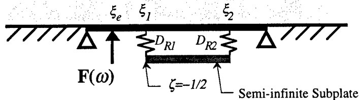
Figure 14. Coupling Scales: Semi-infinite wave-bearing subplate suspended by line springs
