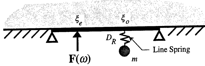
Figure 10. Elastic Scales: Semi-infinite plate with Line mass suspended by line spring.
