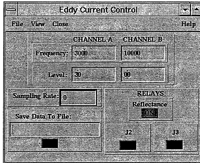
FIGURE 17. EDDY-CURRENT INSTRUMENT INTERFACE
