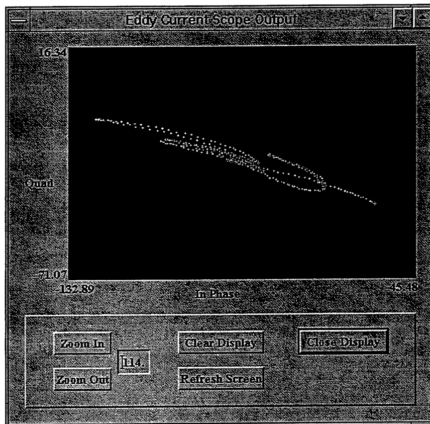
FIGURE 19. EDDY-CURRENT IMPEDANCE PLANE DISPLAY
