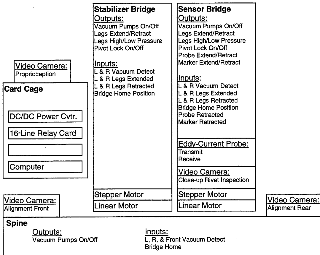
FIGURE 8. ONBOARD COMPUTER AND ROBOT ELECTRONICS
