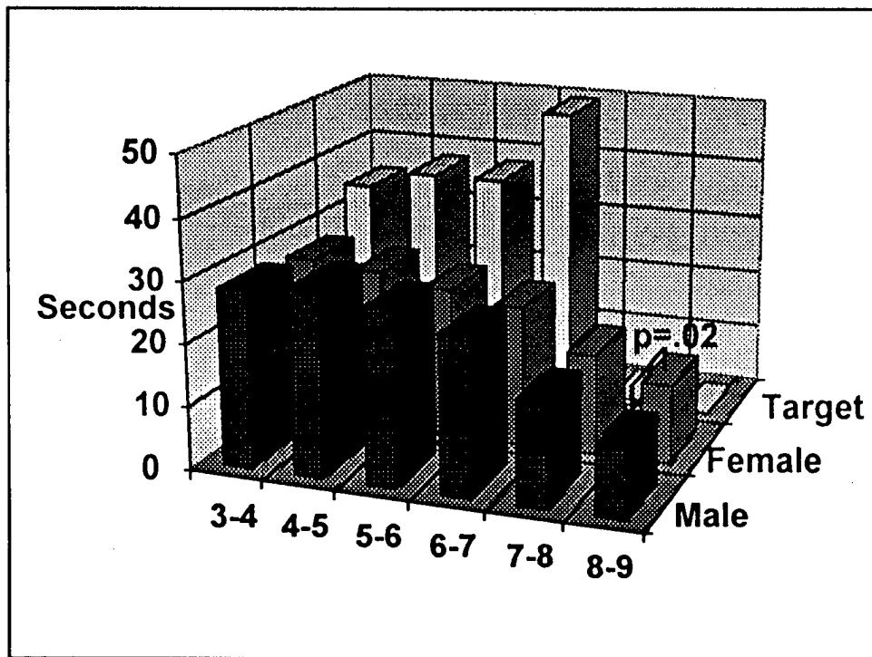
Figure 8. G Distribution
