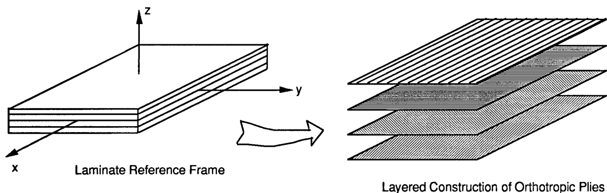
Figure 7—Laminate Constructed from Thin, Arbitrarily-Oriented, Orthotropic Plies
