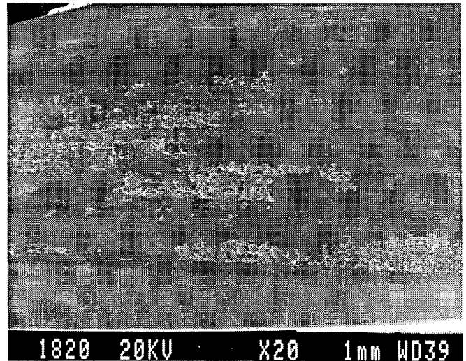
Figure 10.—Pitting damage typically found during testing. (set "J").
