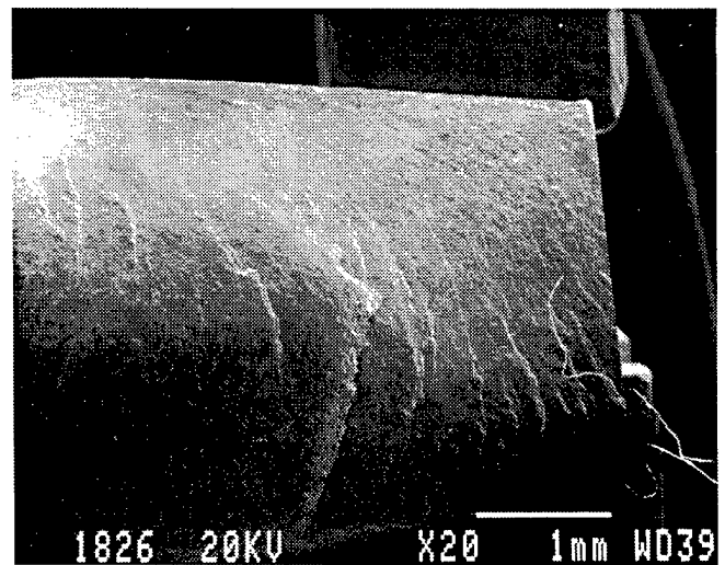
Figure 11.—Photograph of bending failed tooth fracture surface. (set "J").
