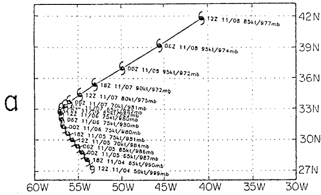
Track of hurricane Florence starting on 4 November at 1200 UTC.
