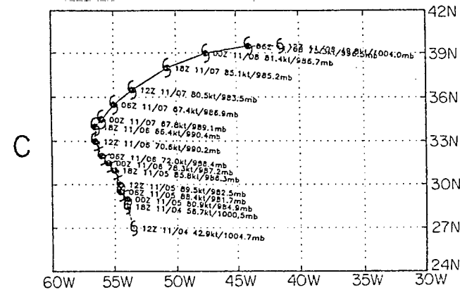
Track of physically initialized forecast for hurricane Florence starting on 4 November at 1200 UTC.
