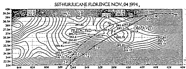
Reynolds weekly OI SST for the week of 4 November 94 with the observed and physically initialized tracks from hours 48 to 96.
