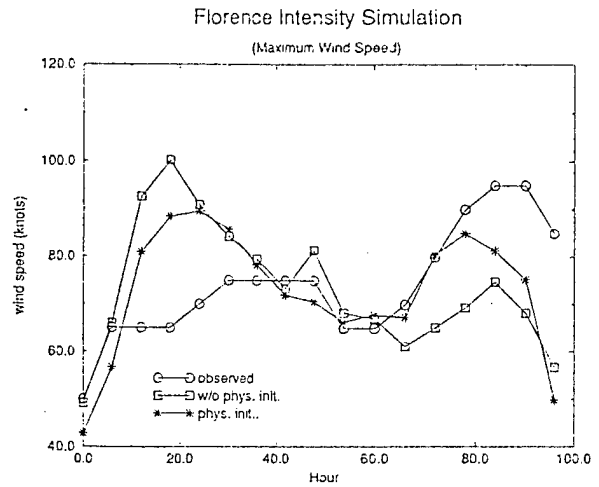
Intensity simulation of hurricane Florence illustrating maximum wind speeds for 96 hr. forecast for observed winds, control experiment and physically initialized experiment.
