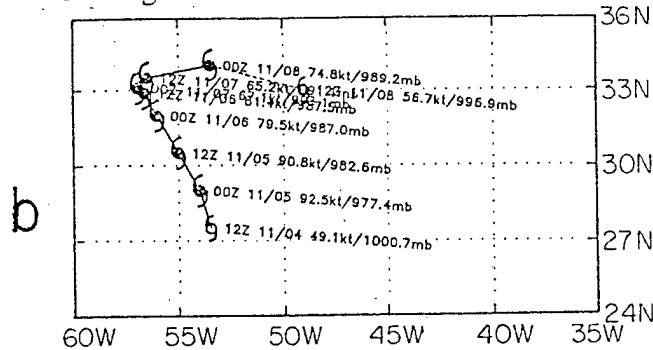
Track of control forecast for hurricane Florence starting on 4 November at 1200 UTC.
