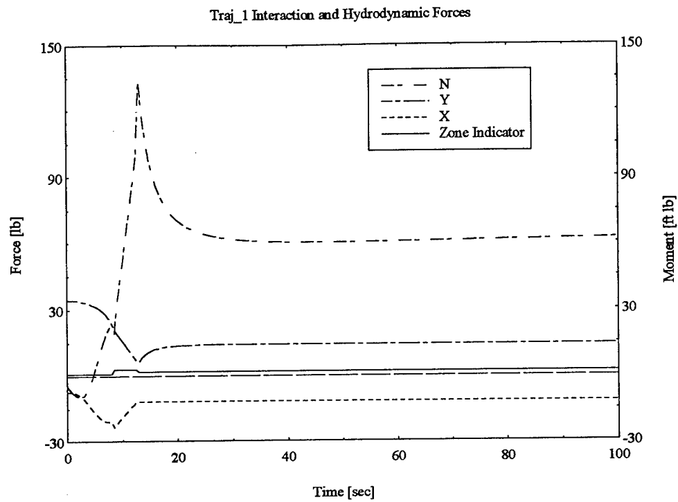
Figure 4.5 Hydrodynamic Forces Including Vehicle Interactions
