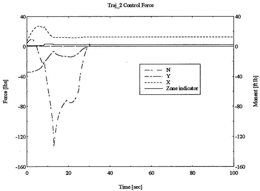
Figure 4.14 Control Force
