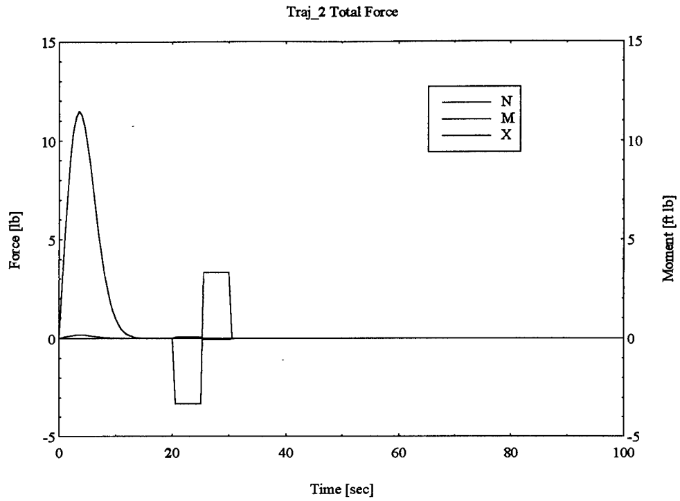
Figure 4.13 Total Force
