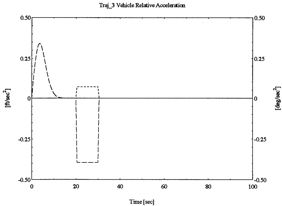
Figure 4.17 Acceleration Profile
