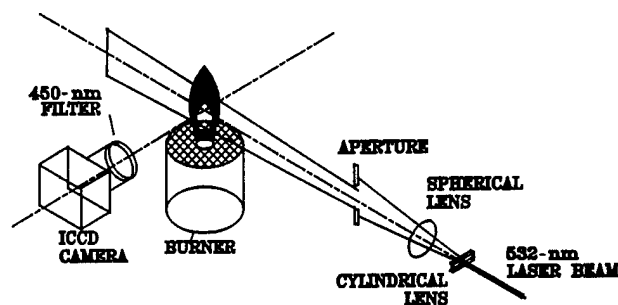
Fig. 1. Experimental setup for 2-D LII imaging.
