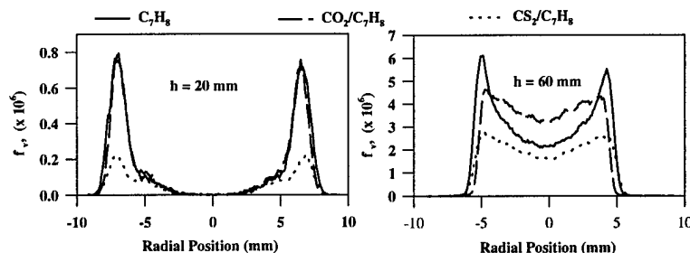
Figure 14. Soot volume fraction profiles with CS_2 addition to quadricyclane / methane mixture flames for measurement heights, h , of 20 mm and 60 mm.
