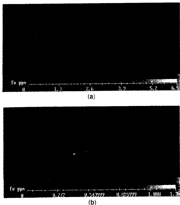
Fig. 11. Soot volume fraction ( f_v ) images of turbulent ethene diffusion flames: (a) Reynolds number 4000, (b) Reynolds number 8000.
