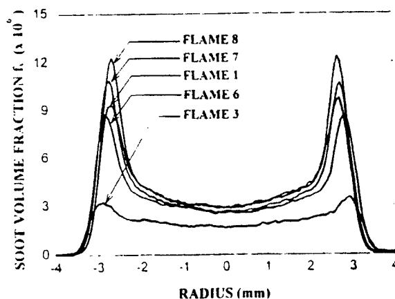
FIG. 4. Comparison of soot volume fraction profiles of the pure ethene flame (flame 1) and the flames mixed with 14.2 C% methane (flame 3), 20 C% ethanol (flame 6), 14.2 C% 1-propanol (flame 7), and 14.2 C% 2-propanol (flame 8) at the 40-mm height.
