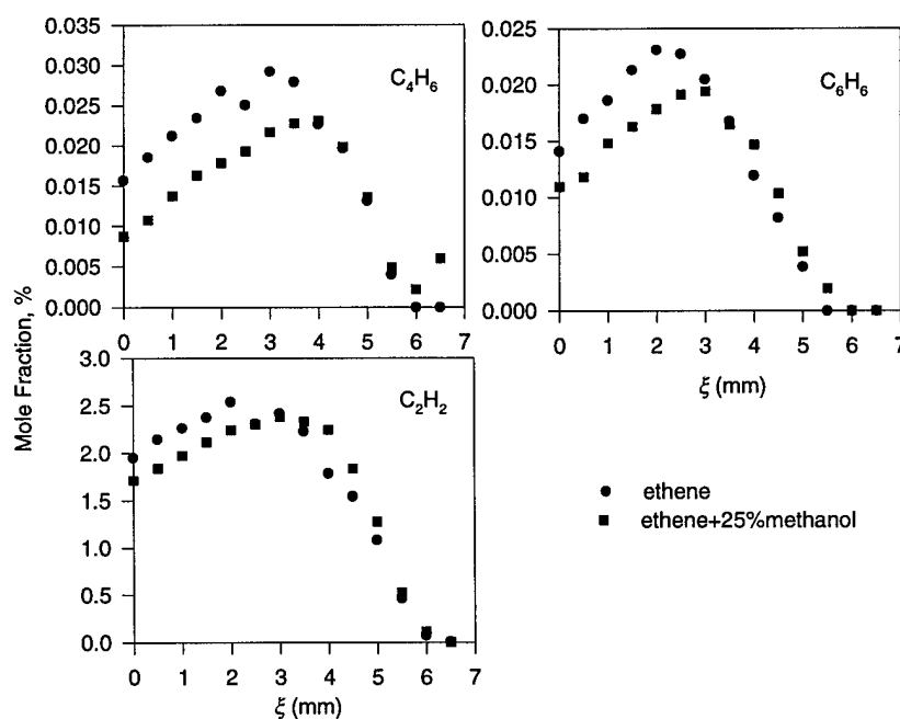
Figure 10. Stable species profiles in C_2H_4 and C_2H_4 + 25\% CH_3OH flames at an axial height of 10 mm.
