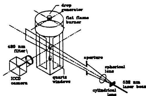
Fig. 1 Experimental setup for 2D-LII imaging
