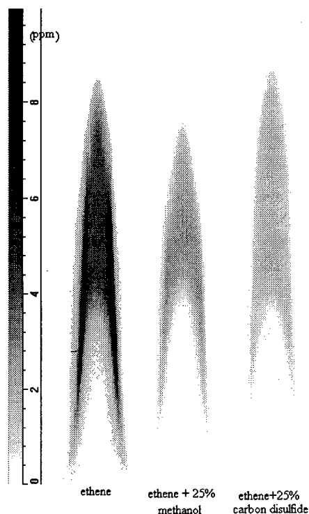
Figure 5. Planar images of soot volume fraction in \text{C}_2\text{H}_4 , \text{C}_2\text{H}_4 + 25\% \text{CH}_3\text{OH} , and \text{C}_2\text{H}_4 + 25\% \text{CS}_2 flames.
