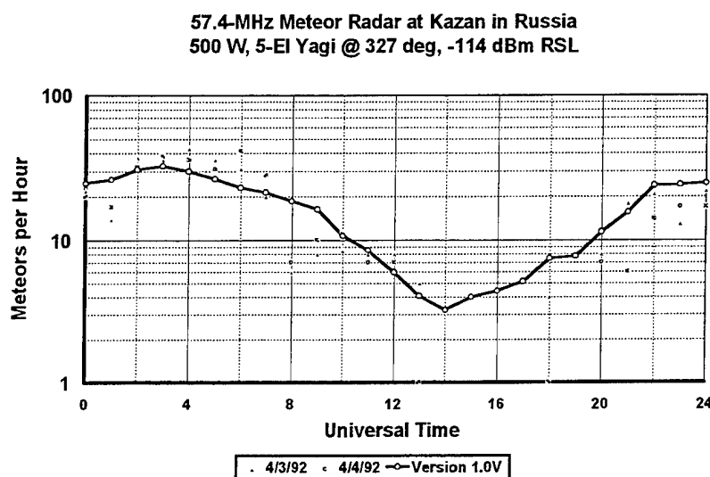
Figure 3.2 Kazan radar (backscatter) measurements
