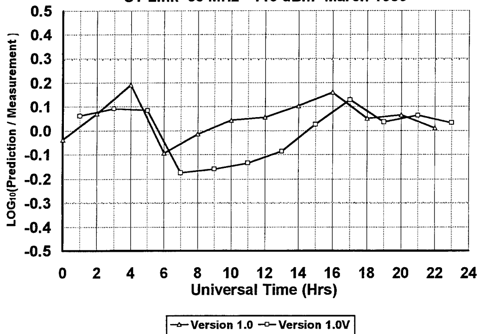
Comparison of %UMR Prediction Accuracy ST Link 65 MHz -110 dBm March 1989
