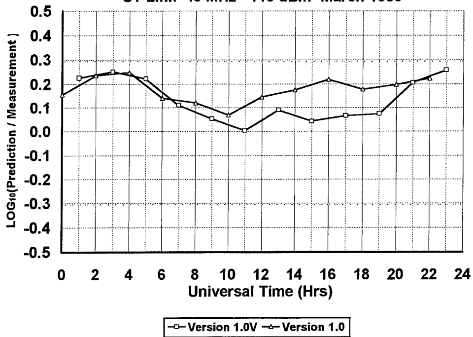
Comparison of %UMR Prediction Accuracy ST Link 45 MHz -110 dBm March 1989
