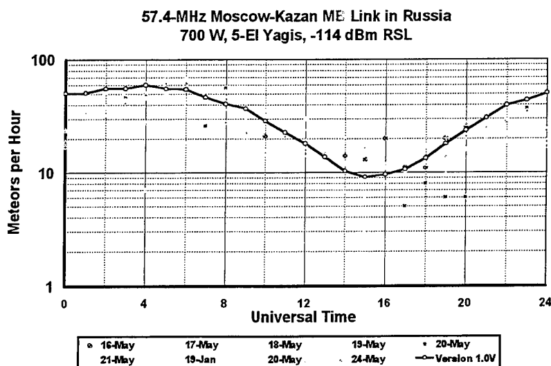
Figure 3.3 Moscow-Kazan forward-scatter MB link
