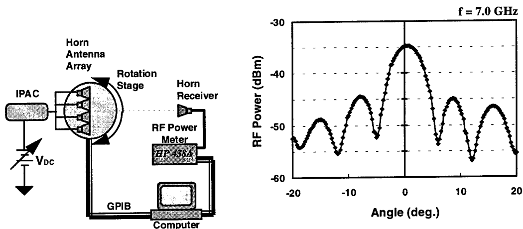
Figure 4.4-3. Antenna Array Pattern Measurement System and Four Element Horn Antenna Array Pattern
