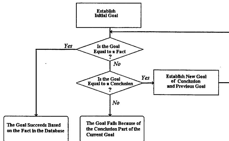
Figure 7. Backward Chaining
