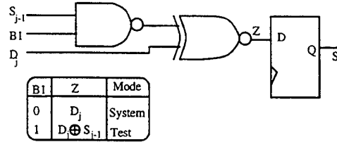
Figure 9.5: CBIST register cell
