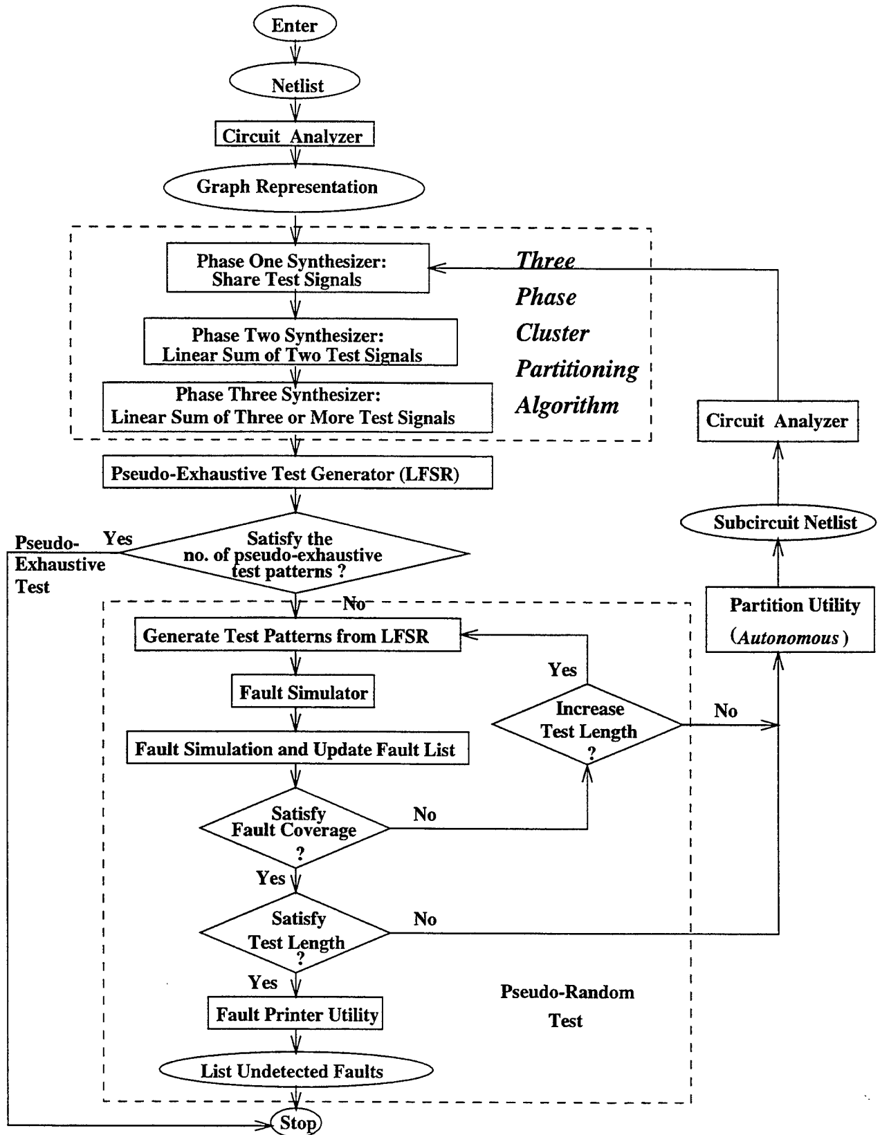
Figure 7.19: BISTSYN System
