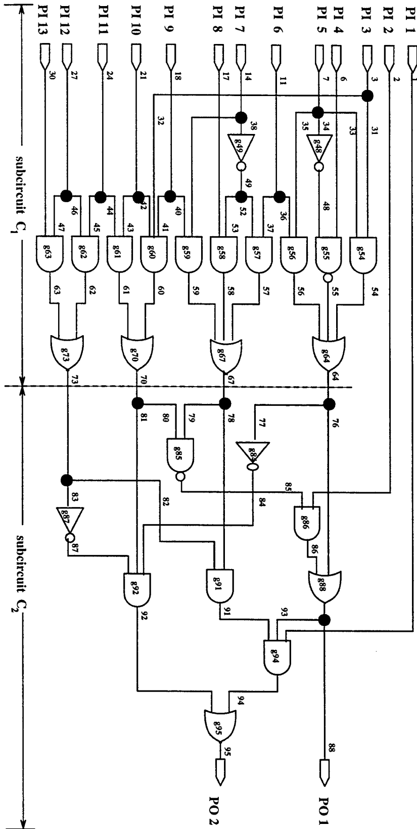
Figure 8.2: Example circuit
