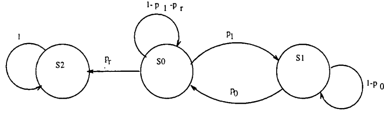
Figure 10.3: Markov model for detecting stuck-at-1 faults
