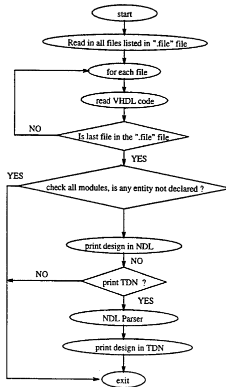
Figure 3.10: Flow chart of the VHDL parser
