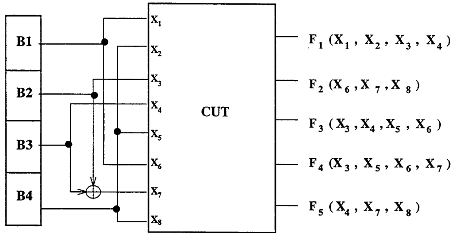
Figure 7.11: Second test scheme of example 1
