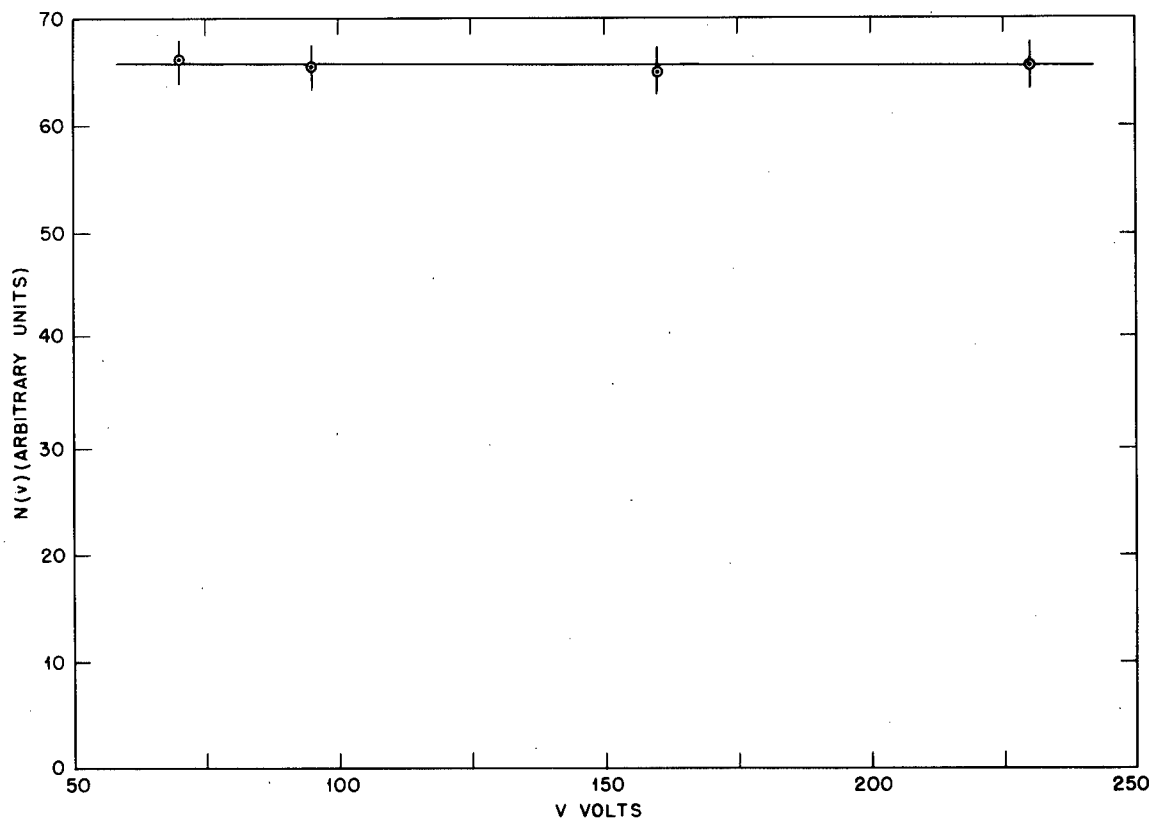
Figure 15. Apparent yield per \mu c vs. positive target voltage, deuteron energy = 80 kev.
