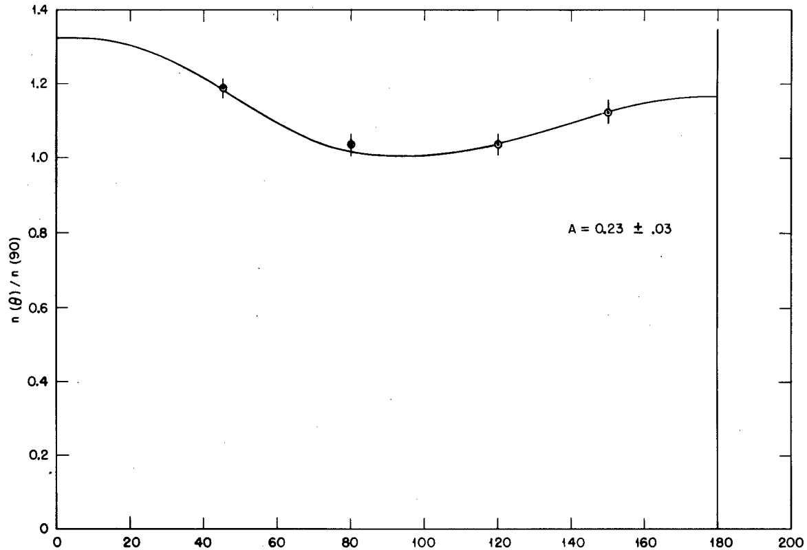
Figure 16. Angular distribution D + D 20 kev. Laboratory system.
