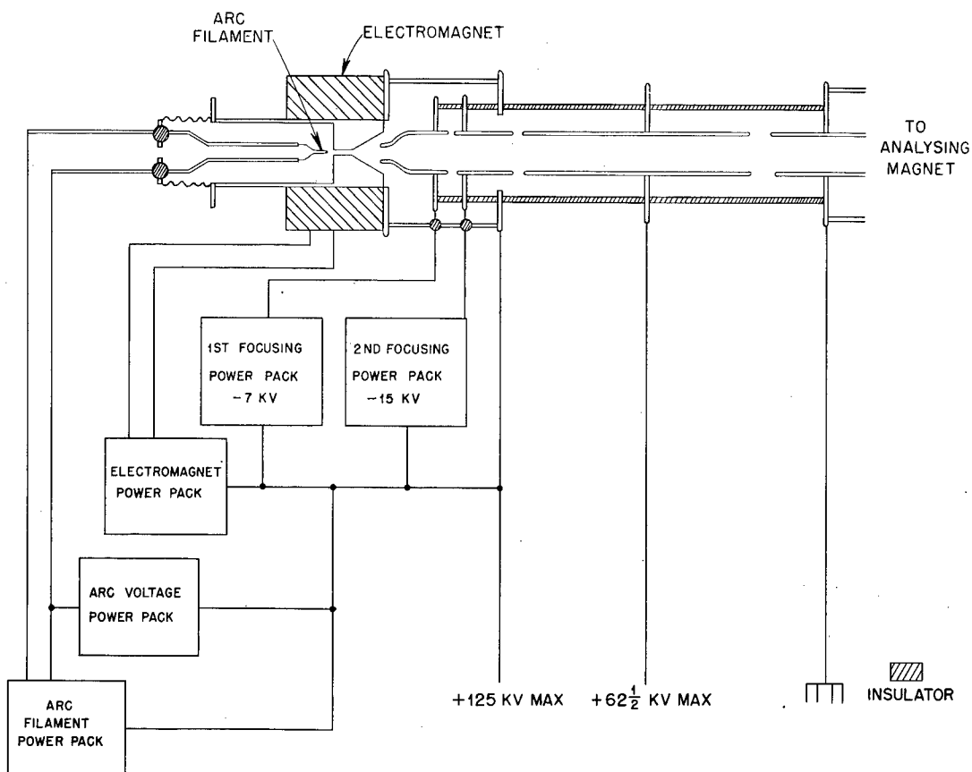
Figure 4. Ion source and accelerating system (125 kv set).
