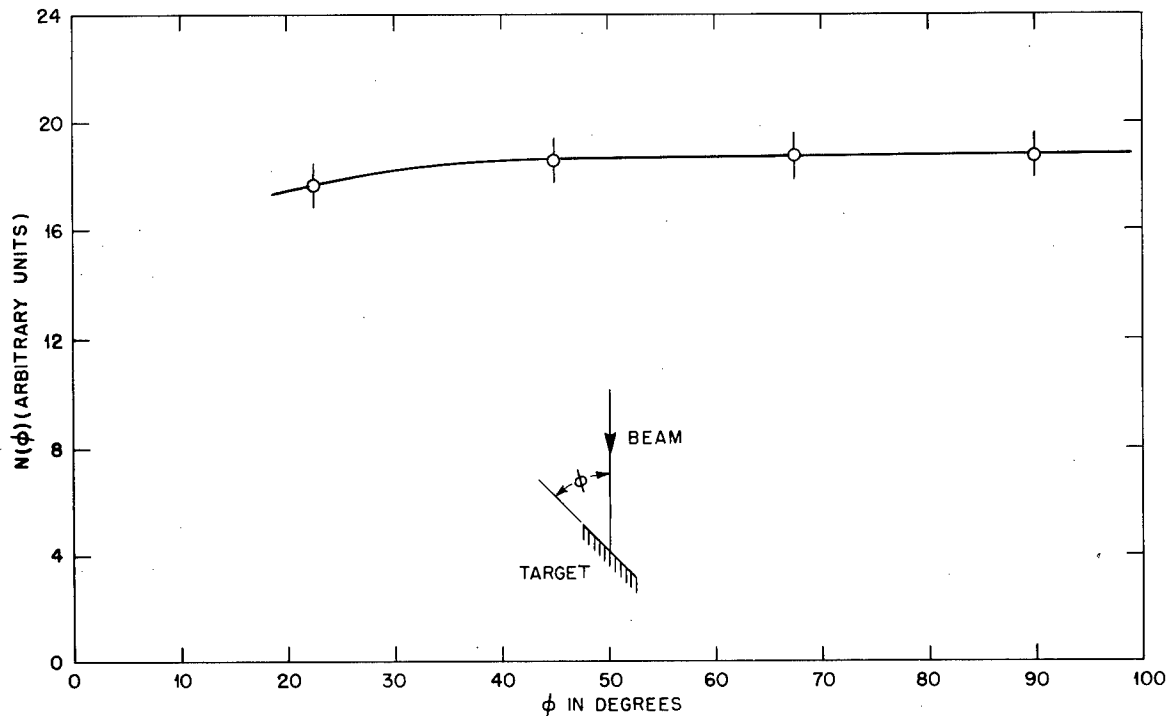
Figure 14. Apparent yield per \mu c vs. target setting, deuteron energy = 40 kev.
