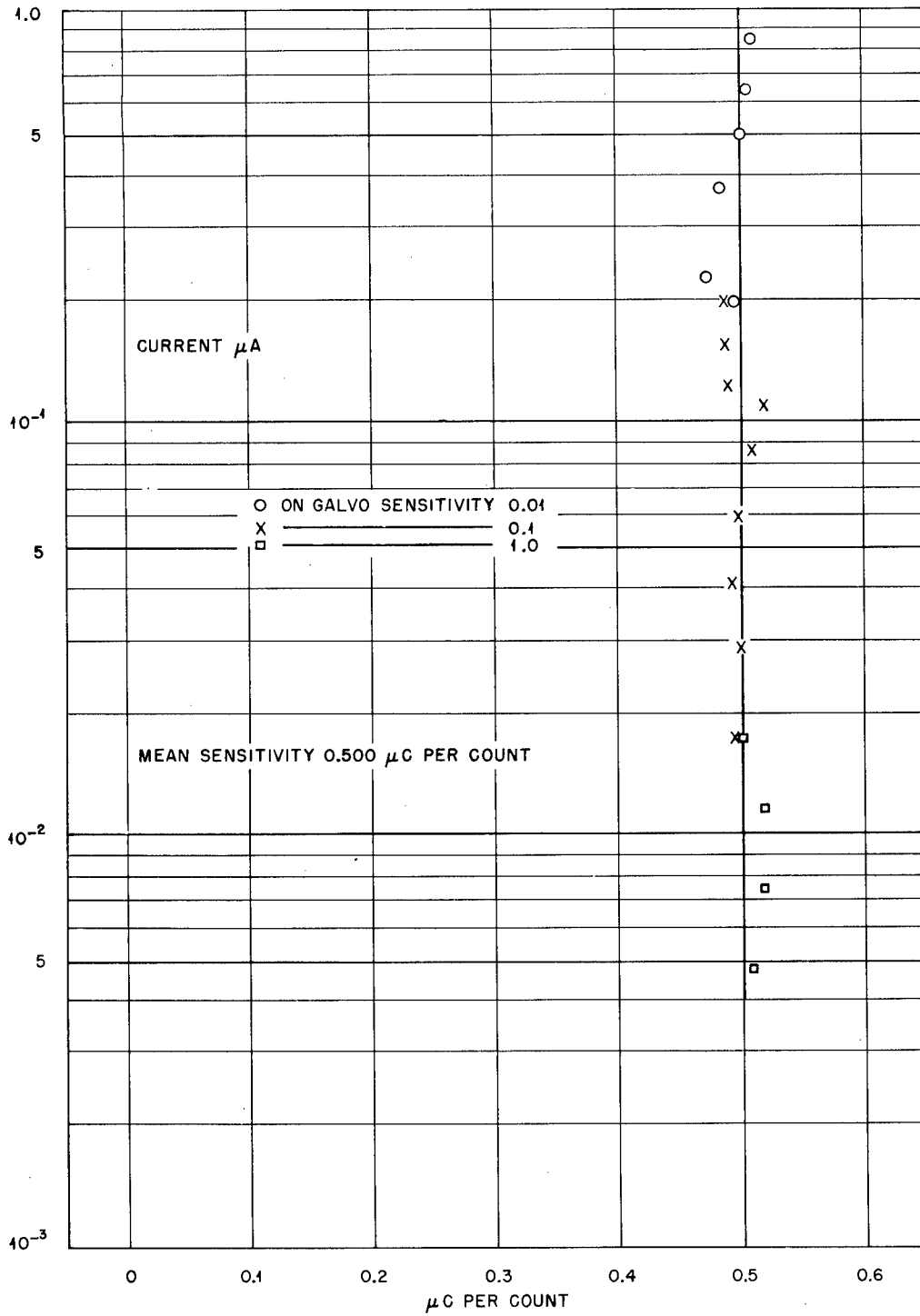
Figure 11. Current integrator sensitivity.
