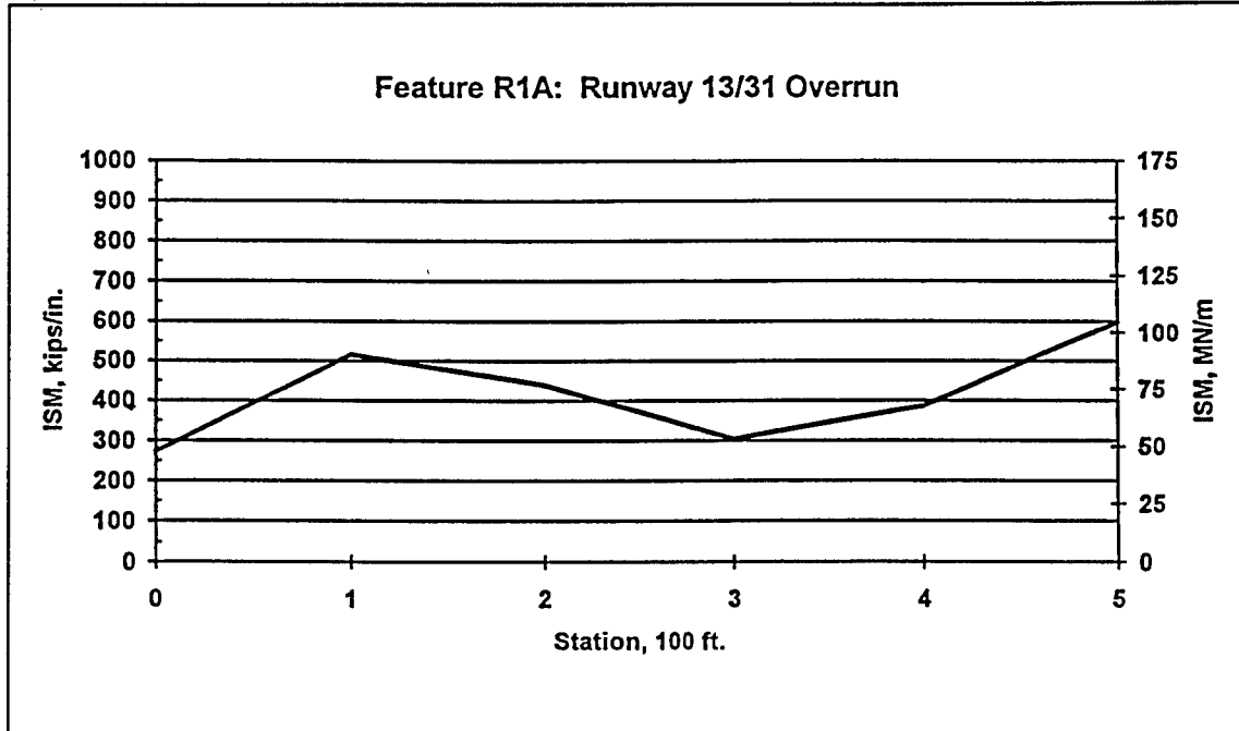
Figure B3. ISM profile for Runway 13-31 Overrun, feature R1A
