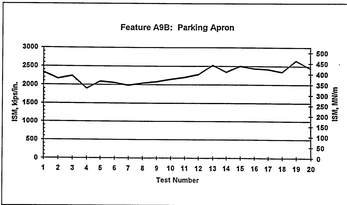
Figure B25. ISM profile for the Parking Apron, feature A9B
