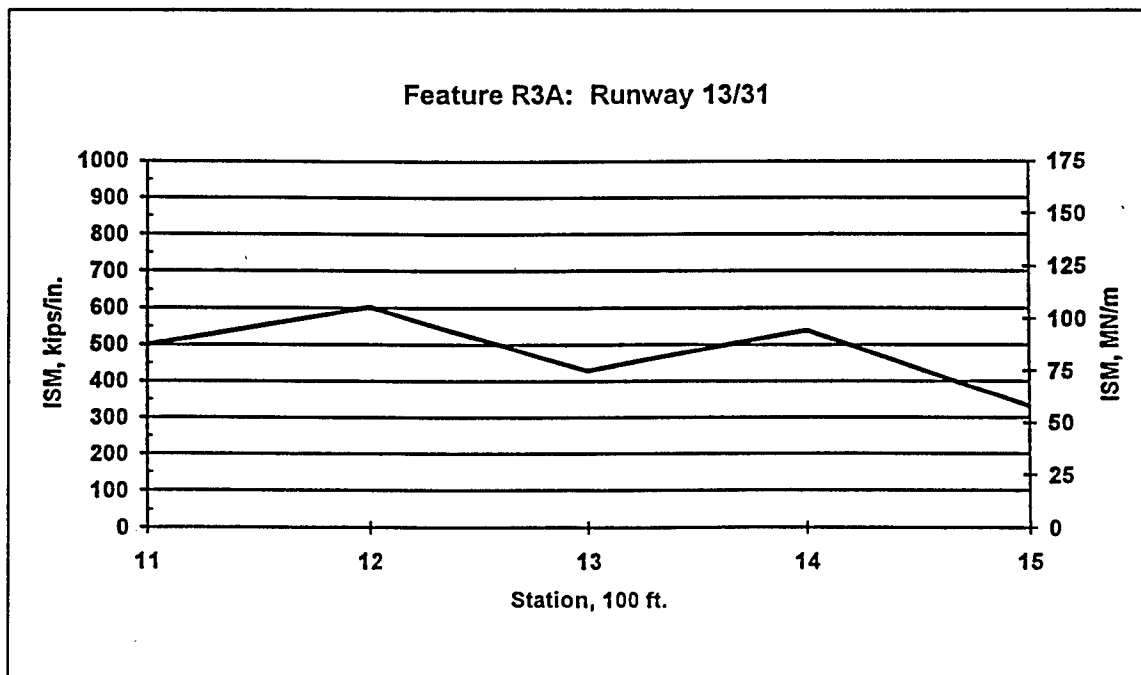
Figure B5. ISM profile for Runway 13-31, feature R3A
