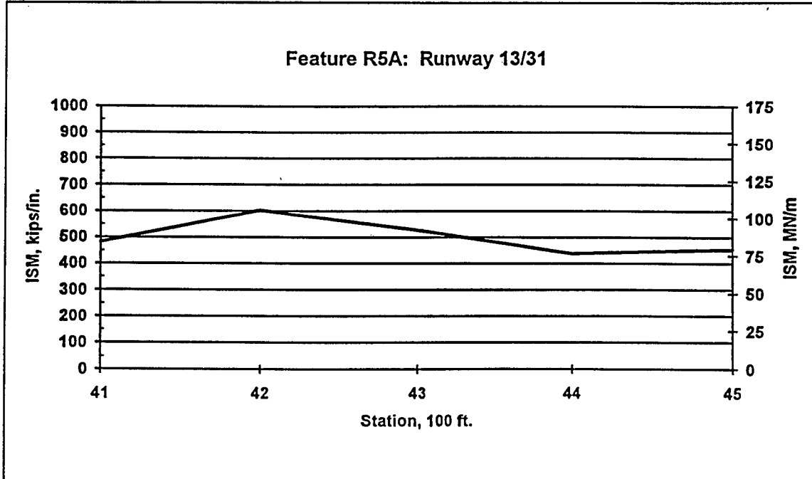
Figure B7. ISM profile for Runway 13-31, feature R5A
