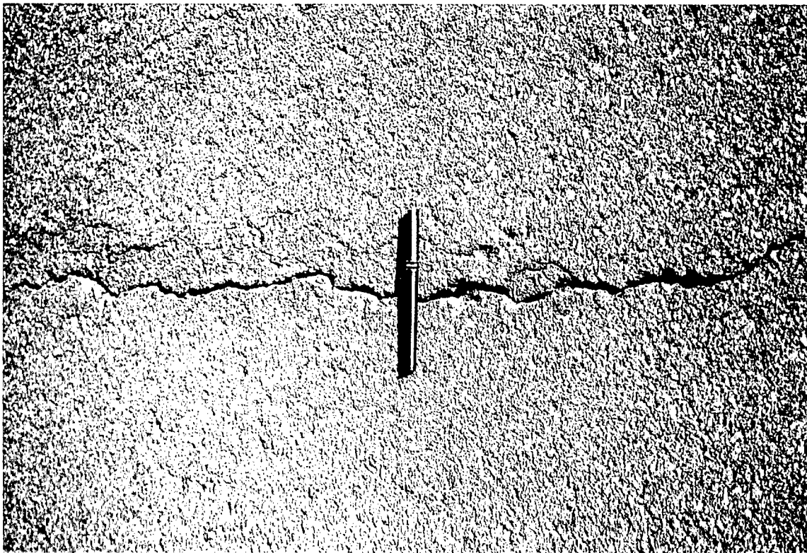
Photo C4. Medium-severity longitudinal and transverse crack
