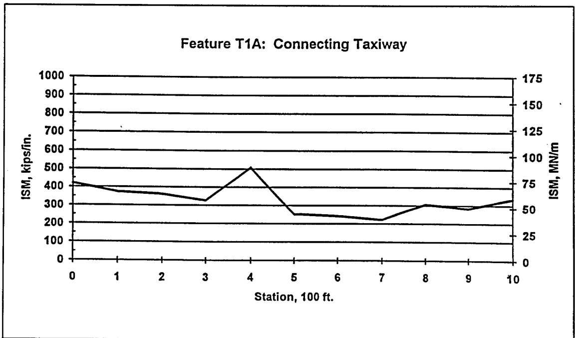
Figure B9. ISM profile for Connecting Taxiway, feature T1A
