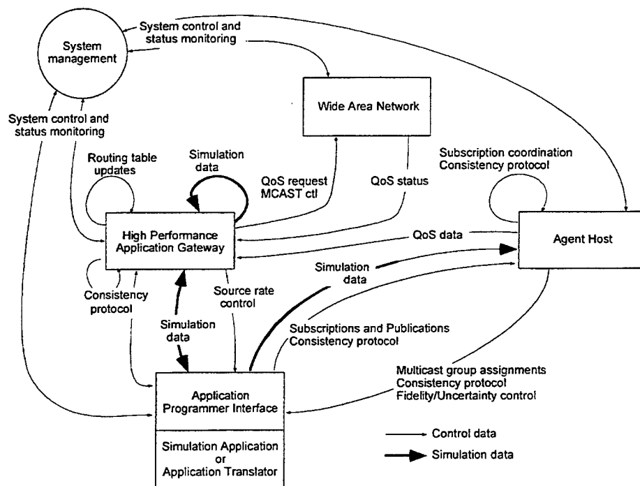
Figure 3. The data flow of the RITN system components.
