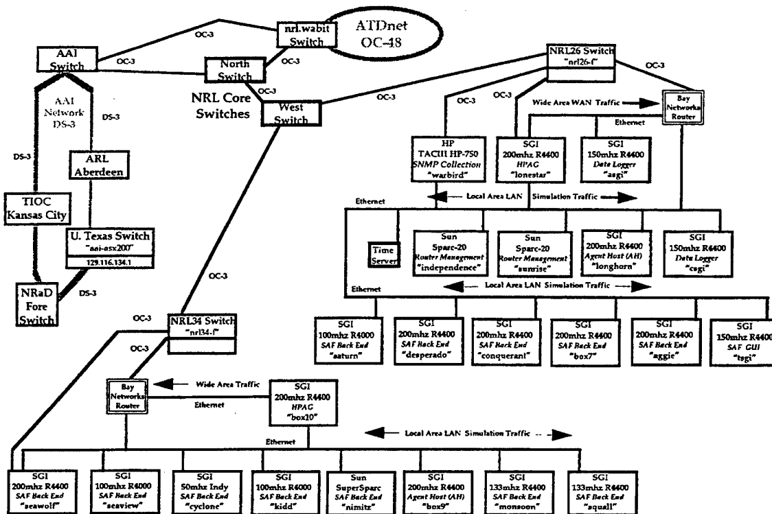
Figure 9. Node site configurations at NRL34 and NRL26.
