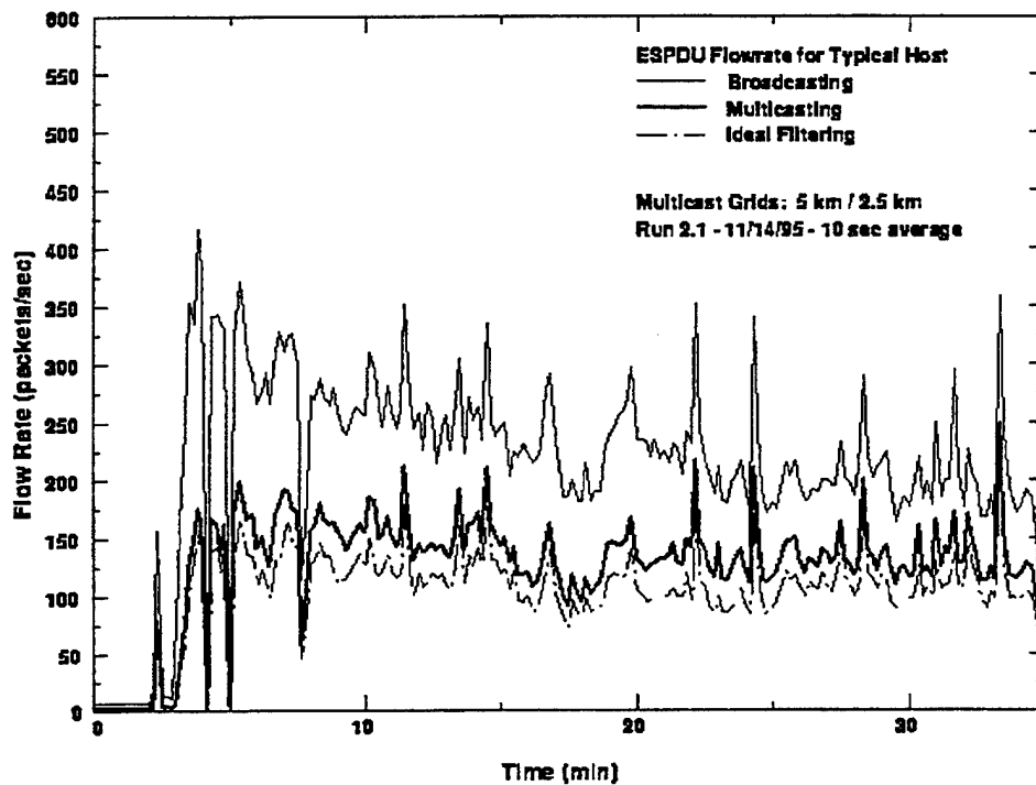
Figure 14. Application-level ESPDU flow multicasting Test Event 2. Note the thick curve is ESPDU flow multicast to 5-km low-rate and 2.5-km high-rate grid.
