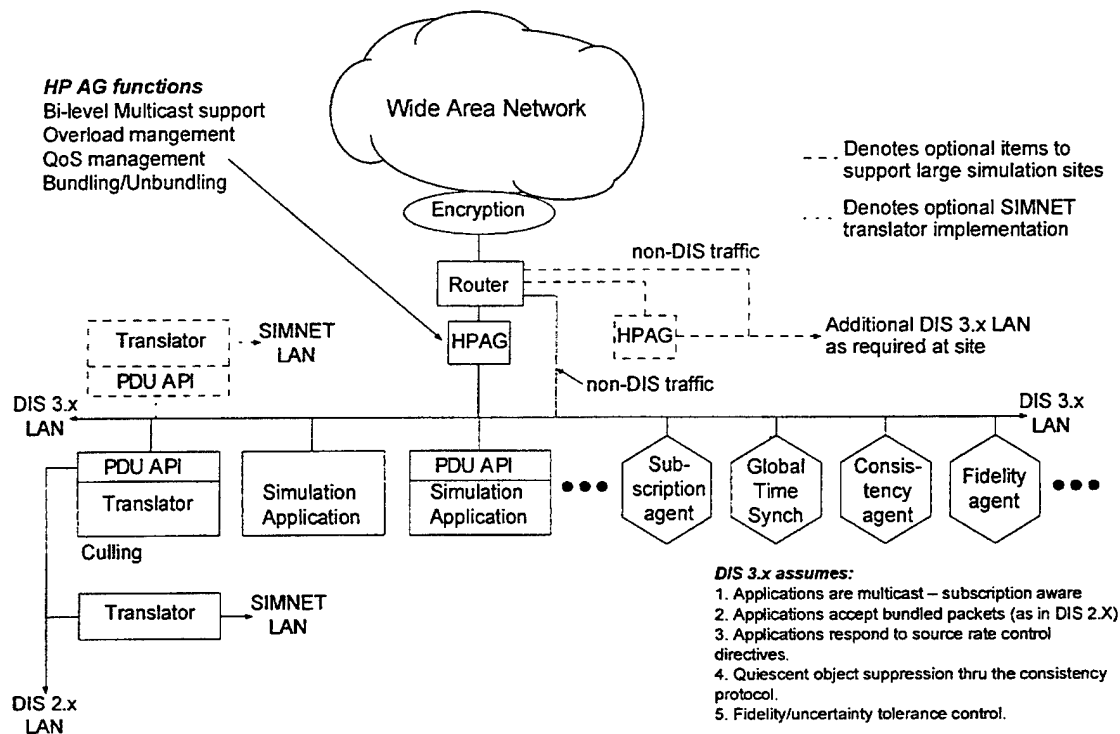
Figure 2. The physical description of the RITN system.
