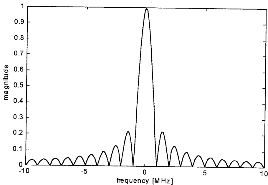
Figure A.8. Frequency profile of the ambiguity diagram of a LFM pulse. (pulse width = 1 microsec)
