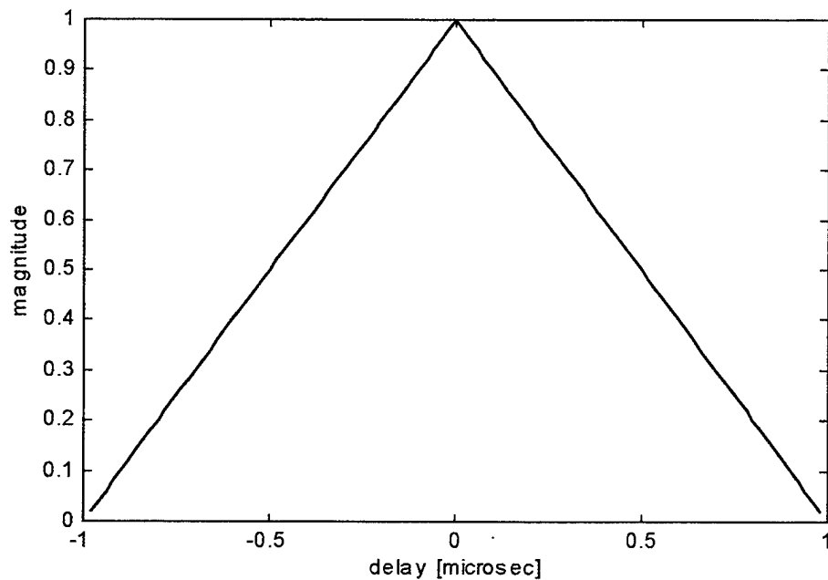
Figure A.3. Time profile of the ambiguity diagram of a single pulse. (pulse width = 1 microsec)
