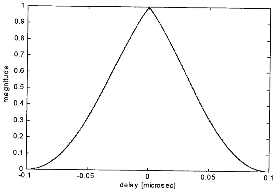
Figure 31. Time profile (cut at zero delay) of the central peak of the step frequency waveform. (N=10, pulse width = 0.1 microsec, PRI = 5 microsec, \Delta f=1\text{MHz} )
