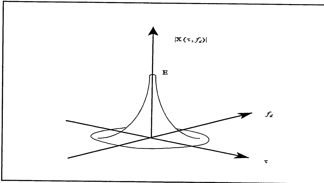
Figure 9. An approximation to the ideal ambiguity diagram "After Ref. [1]."
