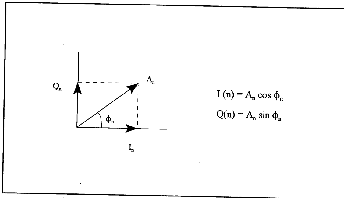
Figure 4. Vector Representation of the Signal Components.
