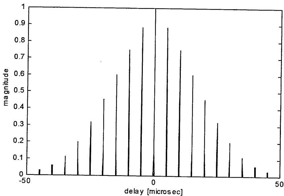
Figure 28. Time profile (cut at zero frequency) of the ambiguity diagram of a step frequency waveform. (N=10, pulse width=0.1 microsec, PRI=5 microsec, \Delta f=1 MHz)
