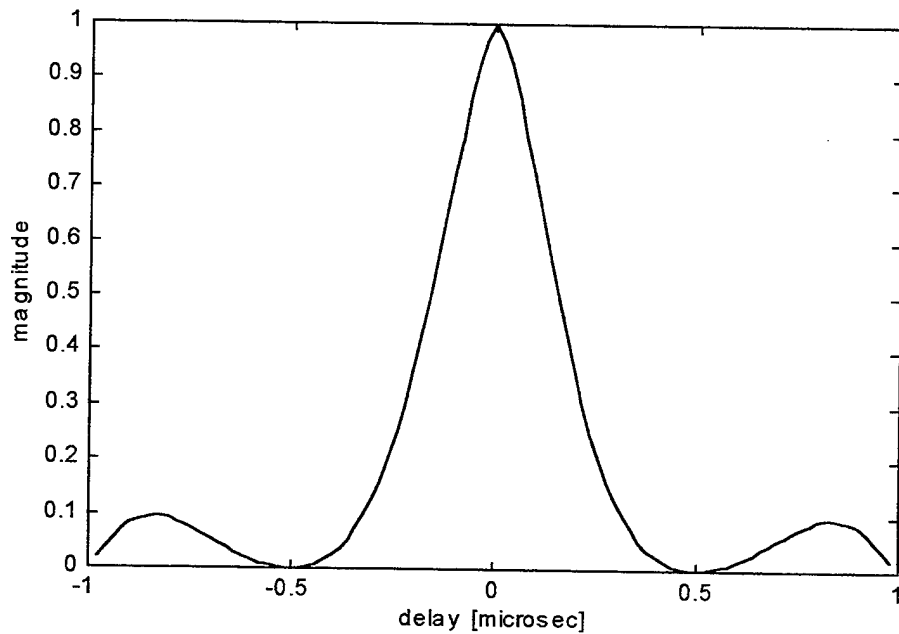
Figure A.7. Time profile of the ambiguity diagram of a LFM pulse. (pulse width = 1 microsec)
