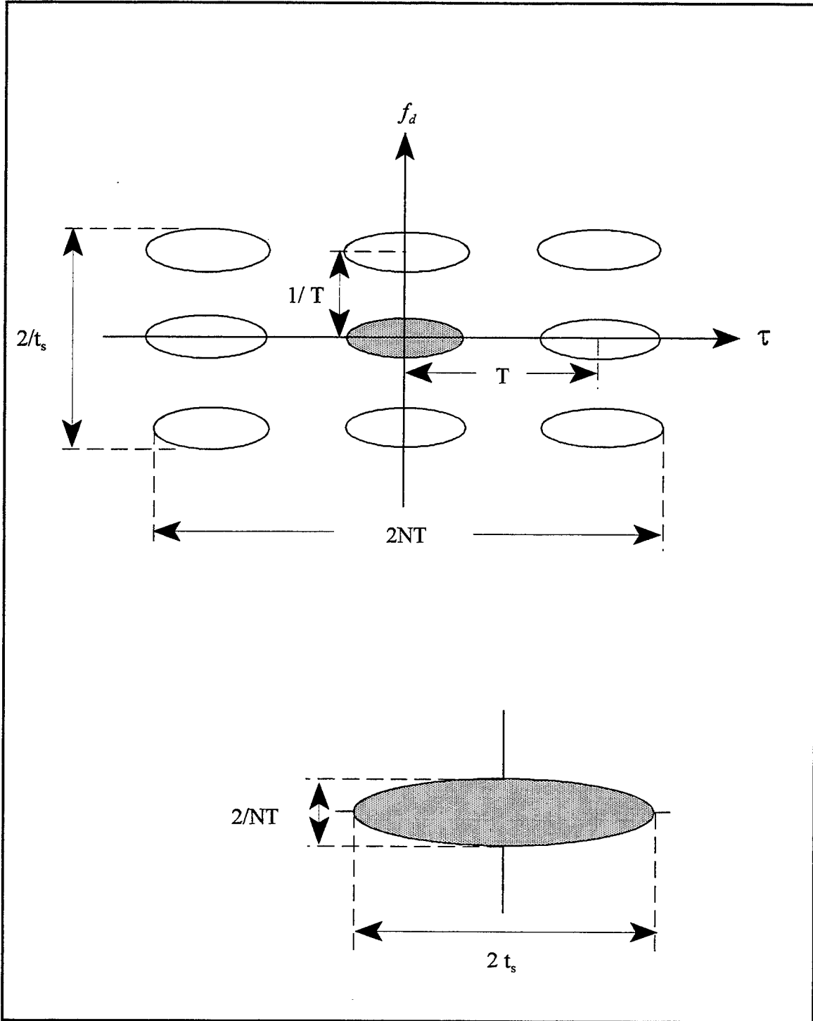
Figure 11. Level contour of the ambiguity surface of a constant frequency pulse train.
