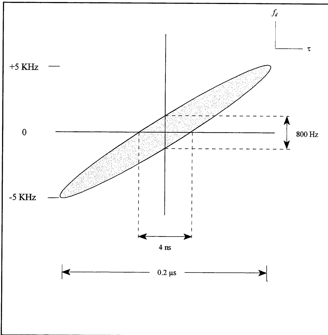
Figure 36. Dimensions of the central peak for the case N=500 , pulse width = 0.1 \mu\text{s} , PRI = 5 \mu\text{s} , \Delta f = 1 \text{ MHz} . (Values indicated are null-to-null; generally 3dB values are given which are a little less than half of the indicated.)
