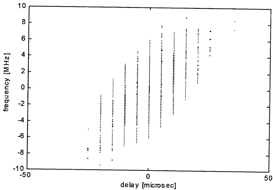
Figure 27. Contour plot of the ambiguity diagram of a step frequency waveform. (N=10, pulse width=0.1 microsec, PRI=5 microsec, \Delta f=1 MHz)
