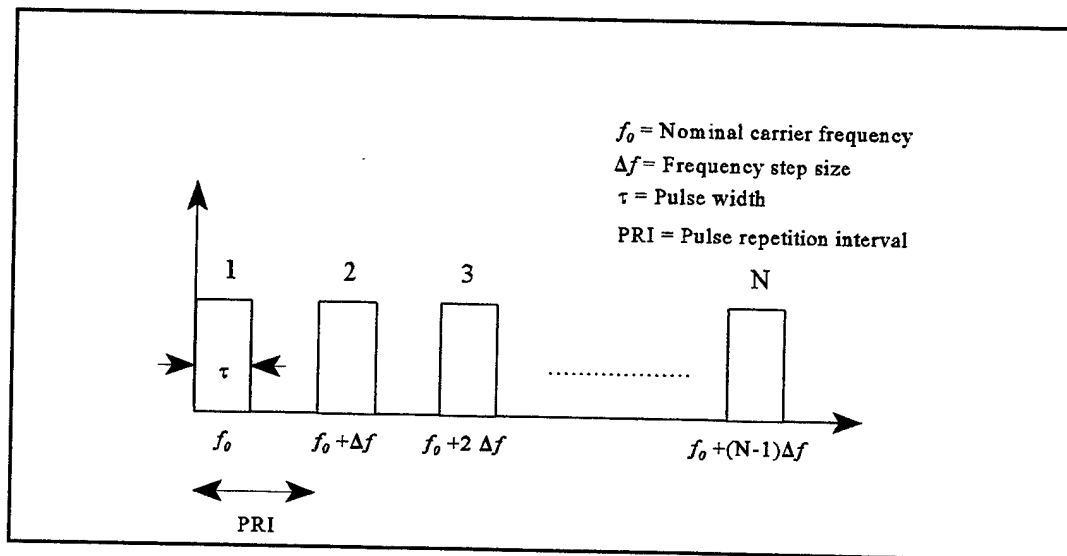
Figure 1. Step Frequency Waveform.
