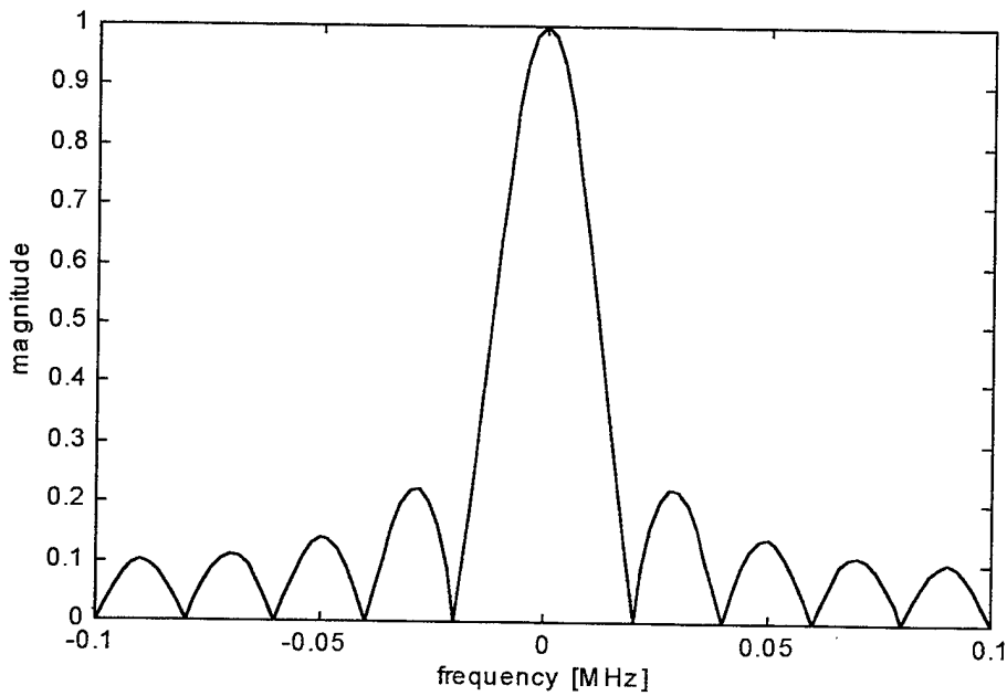
Figure 32. Frequency profile (cut at zero delay) of the central peak of a step frequency waveform. (N=10, pulse width=0.1 microsec, PRI=5 microsec, \Delta f=1\text{ MHz} )
