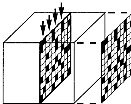
Figure 2-7: A page of bits can be retrieved from a 3D two-photon memory by illuminating it with a plane of light.
