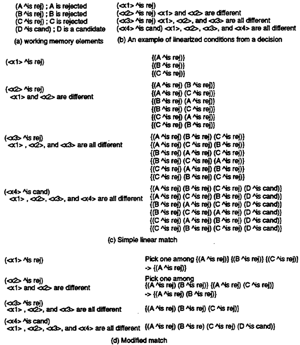
Figure 7: Tokens with linear and nonlinear match.
