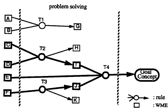
Figure 1: An example of Soar/EBL process.
