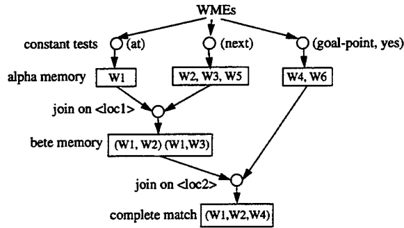
Figure 2: Rete network of a rule.
