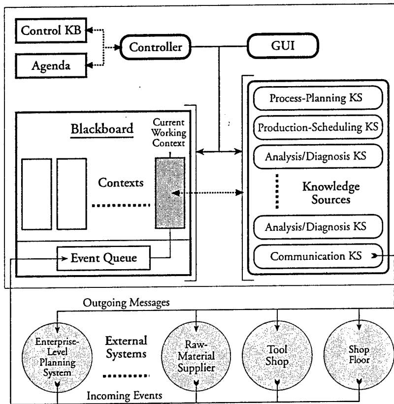
Figure 1: Overview of the IP3S Blackboard Architecture
