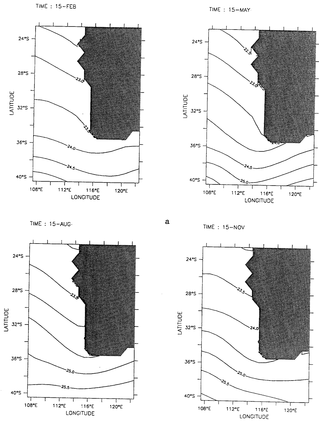
Figure 6. Seasonal density ( \sigma_t ) fields with constant (a) and variable (b) salinity at 10 m depth in February, May, August, and November. The contour interval is 0.5
