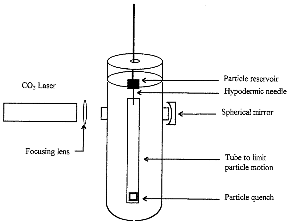
Figure 6. Schematic of the windowed combustion bomb.
