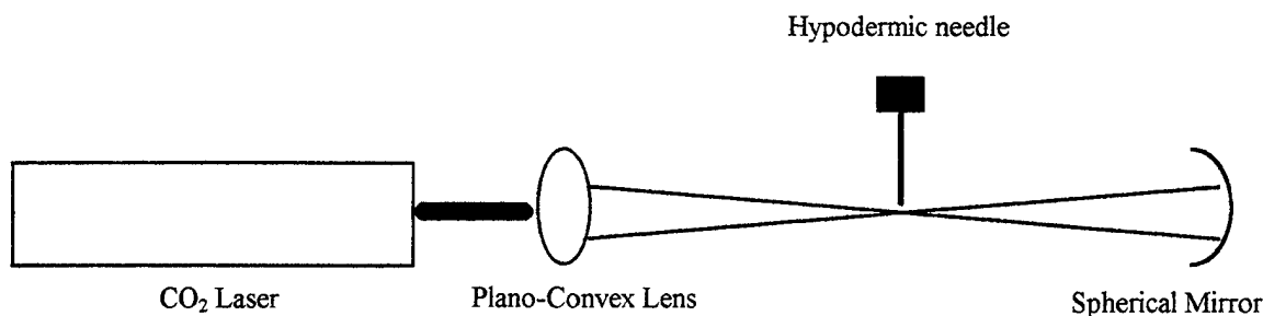
Figure 7. CO 2 Laser and optics diagram.
