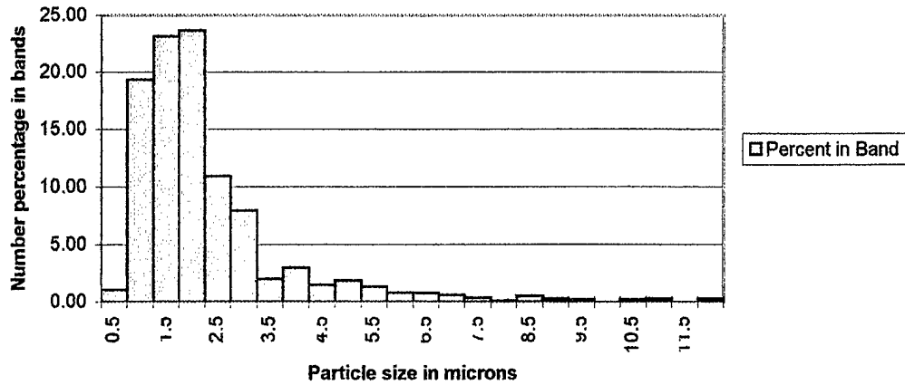
Figure 13. Smoke particle number distribution in 0.5 micron bands.
