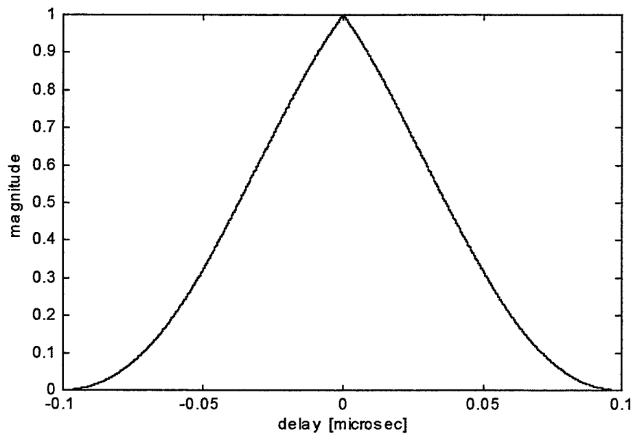
Figure 23. Time profile (cut at zero delay) of the central peak of the step frequency waveform. ( N=10 , pulse width = 0.1 microsec, PRI = 5 microsec, \Delta f=1\text{MHz} )
