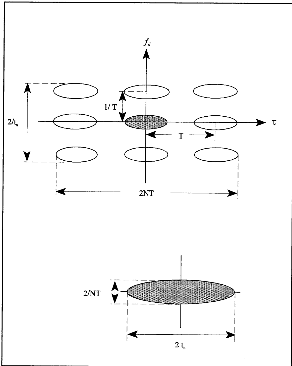
Figure A.11. Level contour of the ambiguity surface of a constant frequency pulse train.
