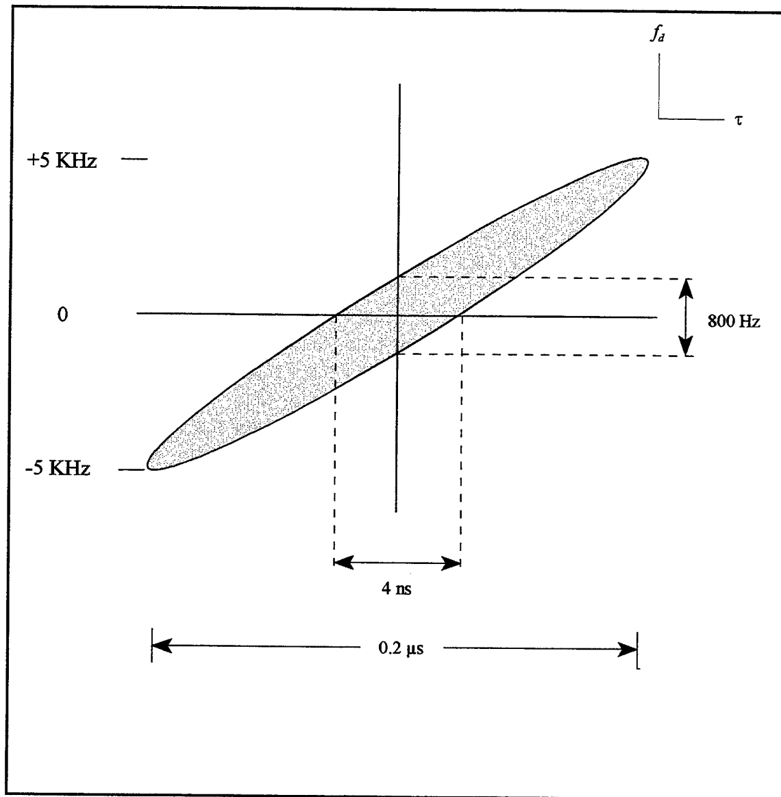
Figure 28. Dimensions of the central peak for the case N=500 , pulse width = 0.1 \mu s , PRI = 5 \mu s , \Delta f = 1 \text{ MHz} . (Values indicated are null-to-null; generally 3dB values are given which are a little less than half of the indicated.)
