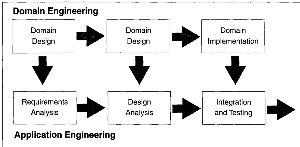
Figure 19: Domain Engineering and Application Engineering
