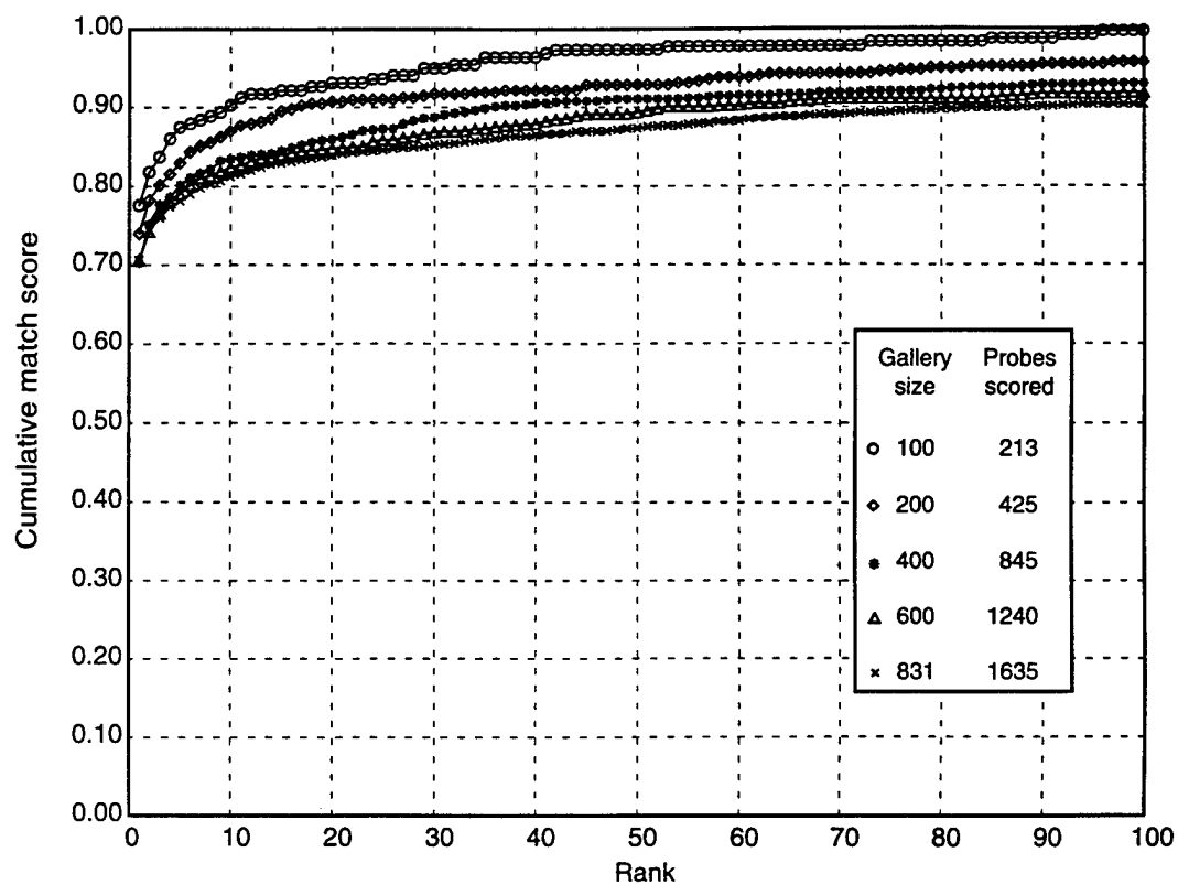
Figure 32. Graduated gallery study: overall scores (March 1995).
