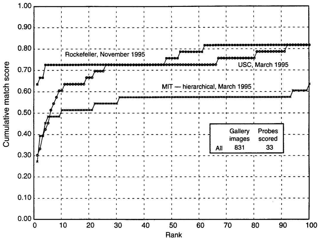
Figure 39. Large gallery tests: quarter rotation scores (November 1995).
