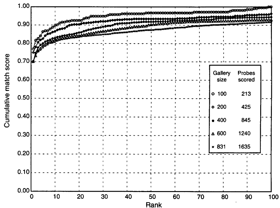
Figure 29. Graduated gallery study: overall scores (March 1995).
