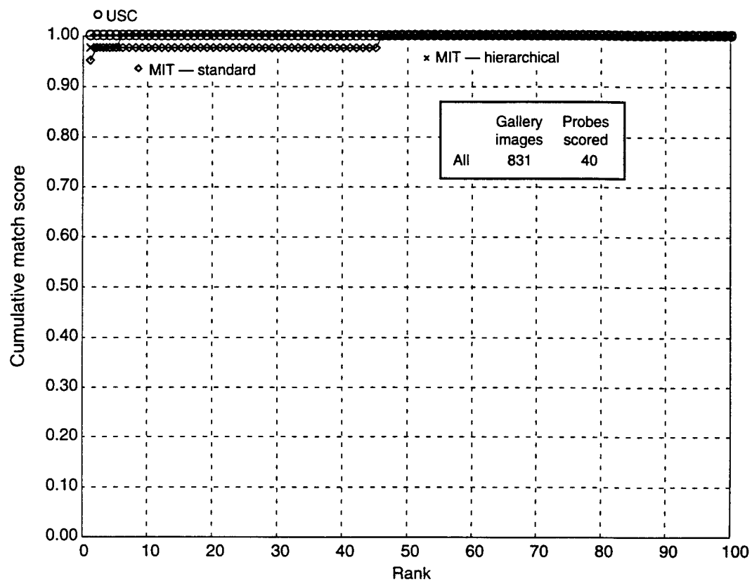
Figure 26. Large gallery test: 20% reduced image size (March 1995).
