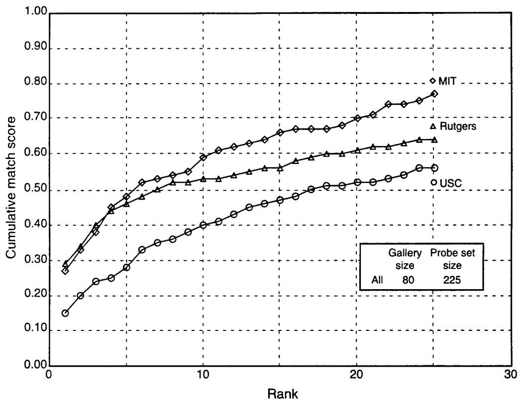
Figure 17. Rotation test: overall scores (August 1994).
