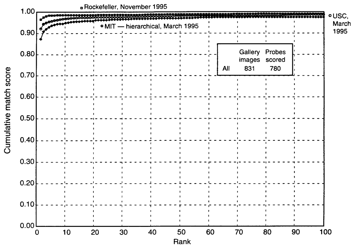
Figure 37. Large gallery tests: FA versus FB scores (November 1995).
