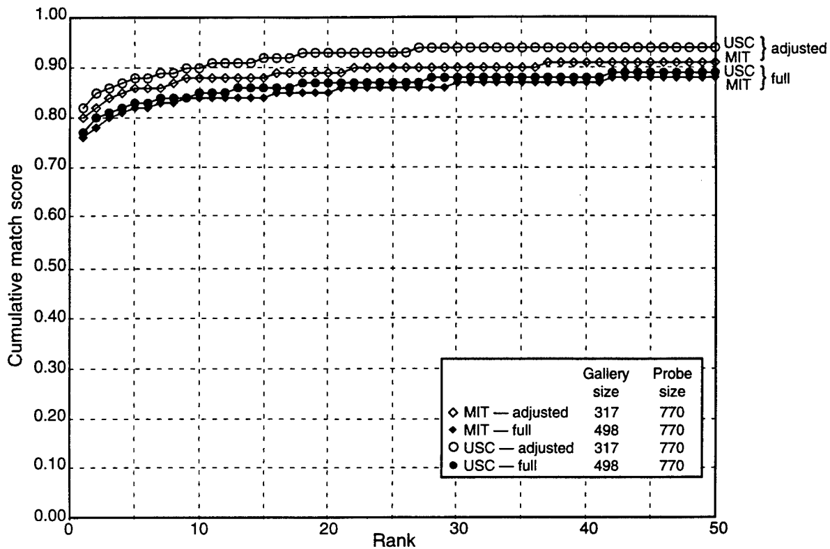
Figure 5. Large gallery test: overall scores: full set versus corrected set (August 1994).
