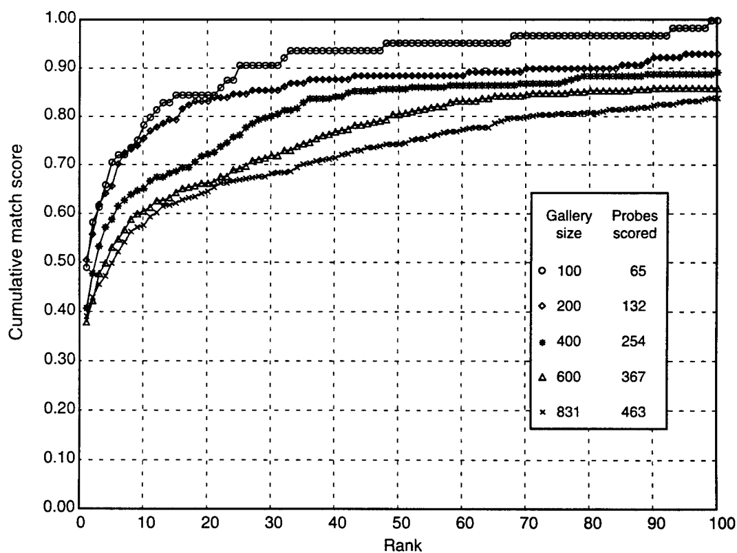
Figure 31. Graduated gallery study: duplicate scores (March 1995).
