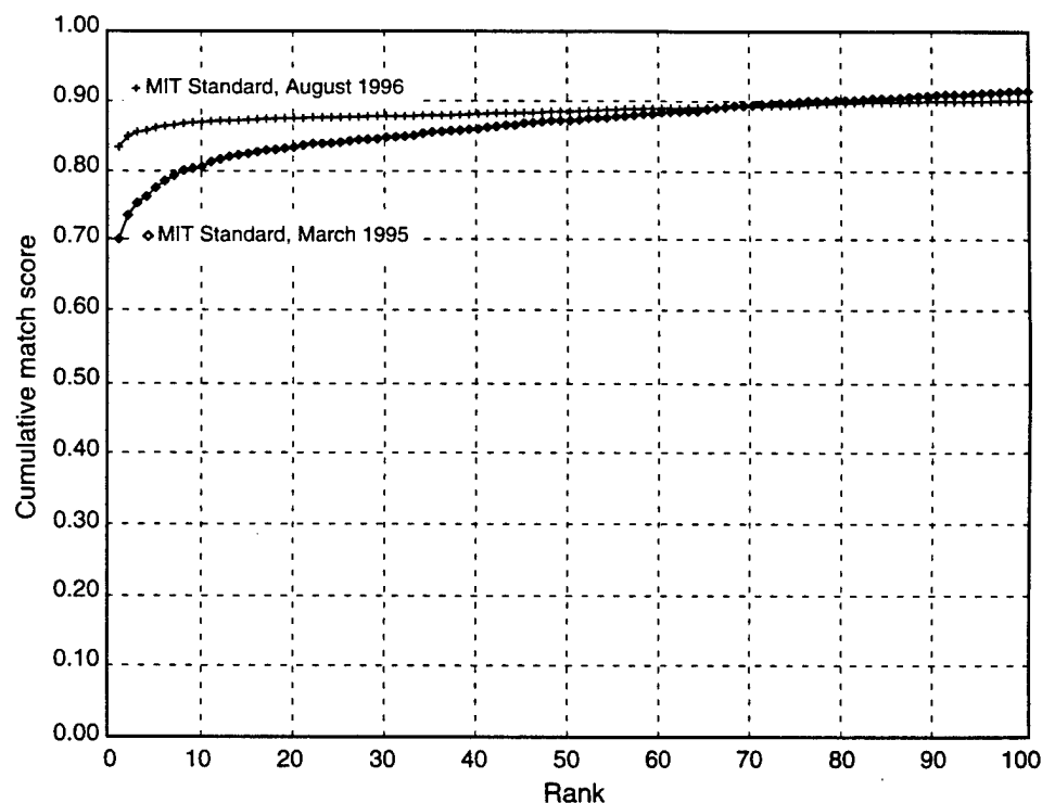
Figure A-1. Comparison of overall scores for March 1995 and August 1996 algorithms.
