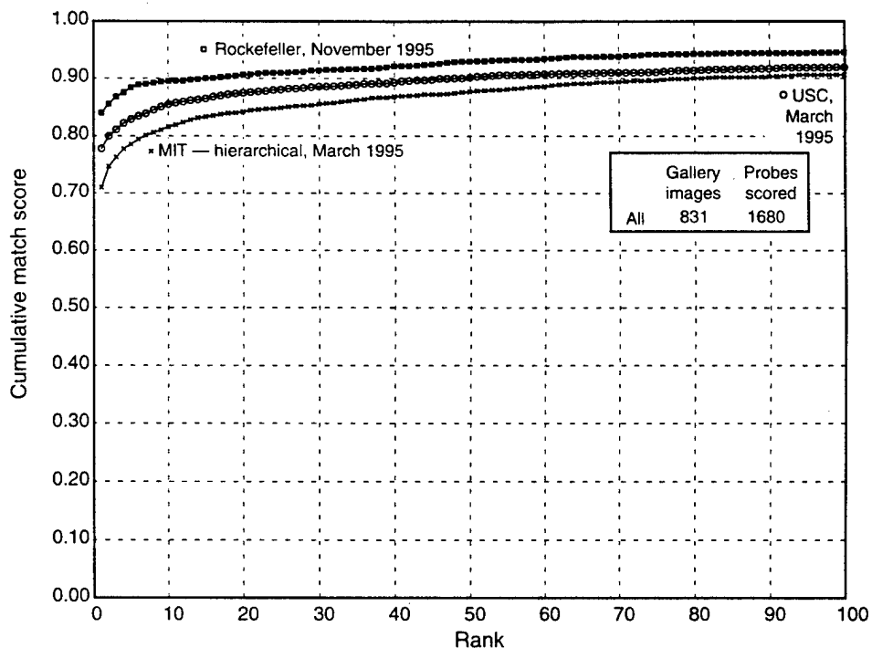
Figure 36. Large gallery tests: overall scores (November 1995).
