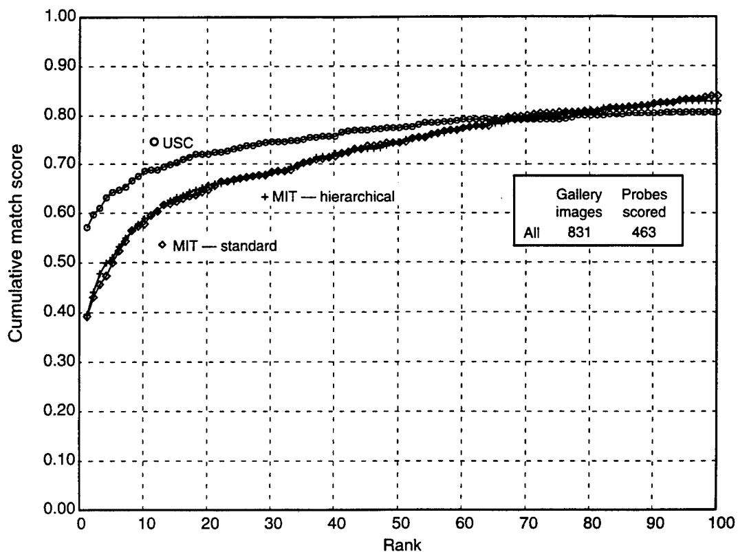
Figure 20. Large gallery test: duplicate scores (March 1995).
