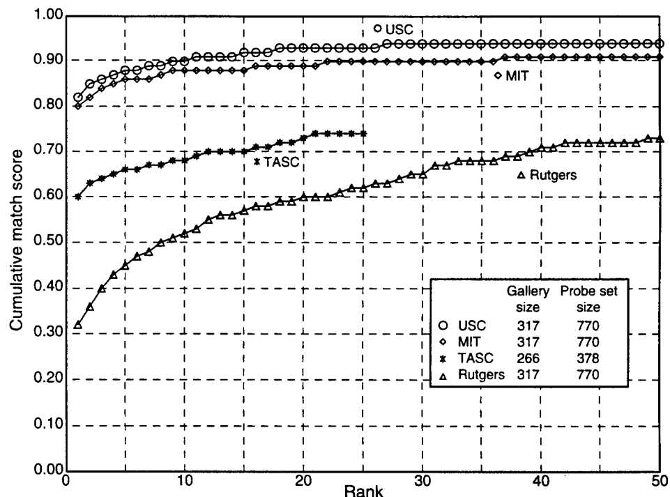
Figure 4. Large gallery test: overall scores, adjusted (August 1994).
