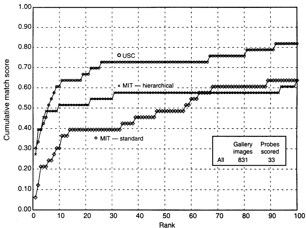
Figure 21. Large gallery test: quarter rotation (March 1995).
