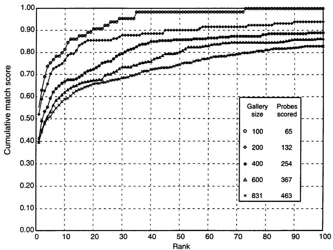
Figure 34. Graduated gallery study: duplicate scores (March 1995).
