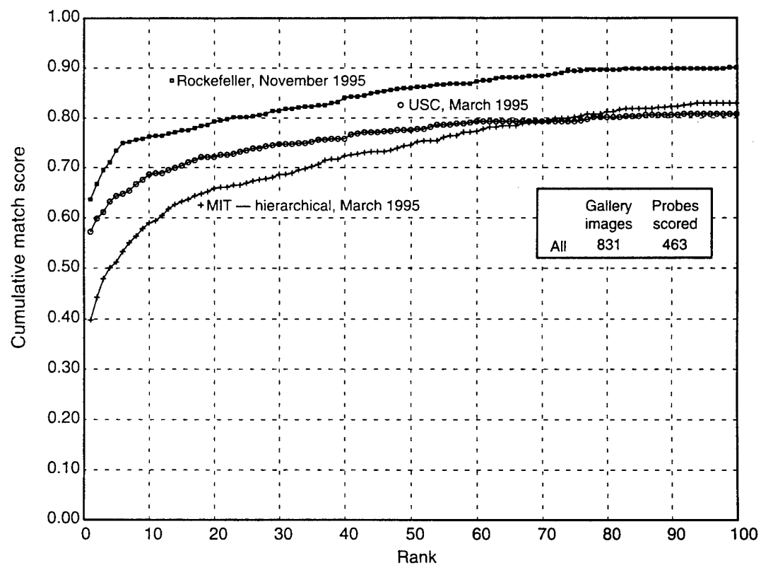
Figure 38. Large gallery tests: duplicate scores (November 1995).
