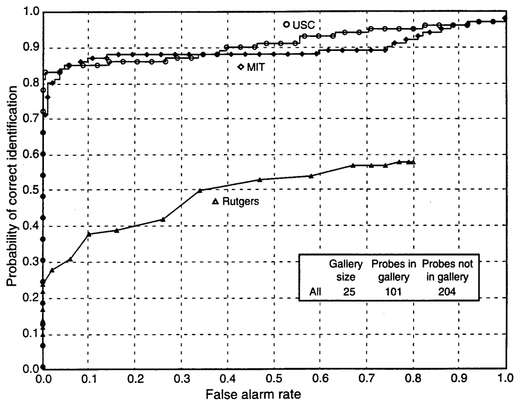
Figure 16. False-alarm test: ROC (August 1994).
