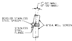
DETAIL
