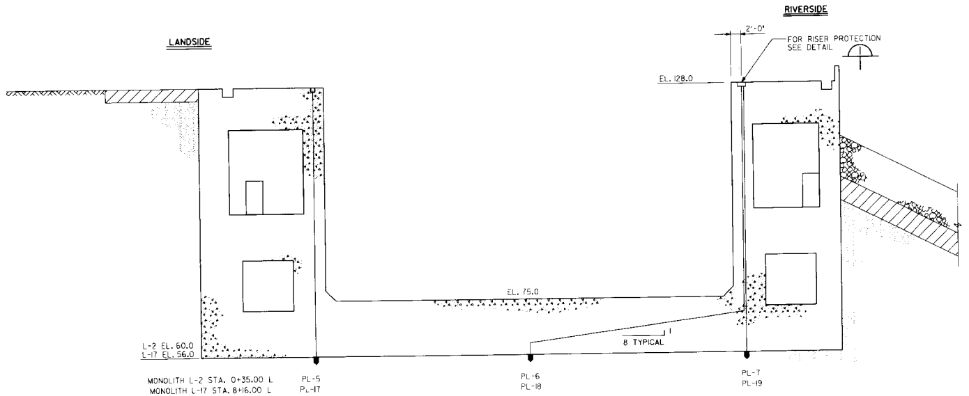
GATE MONOLITH PIEZOMETERS
