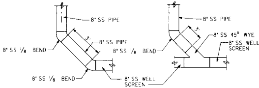
CLEANOUT PIPE DETAILS
