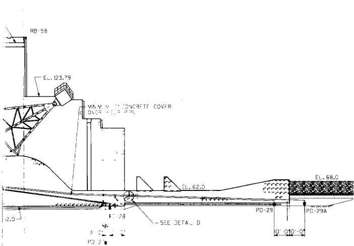
SECTION A
