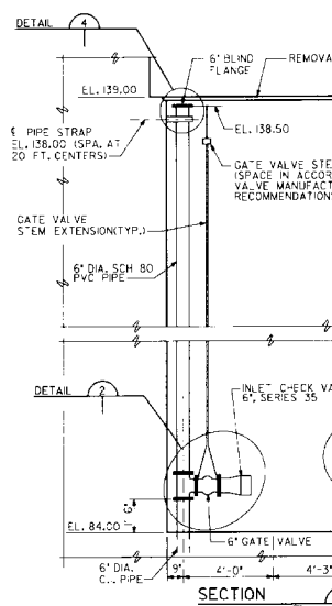
SECTION
