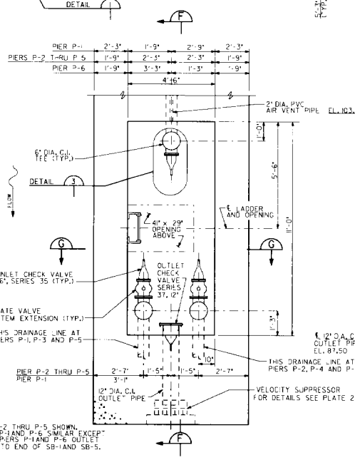
MANHOLE SECTIONAL PLAN
