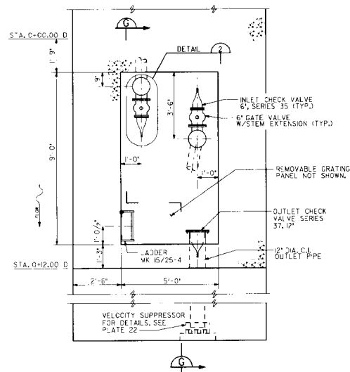
SECTIONAL PLAN - MANHOLE AT PIER P-7
