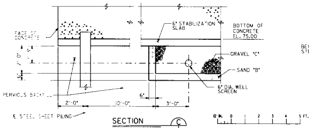
SECTION C
