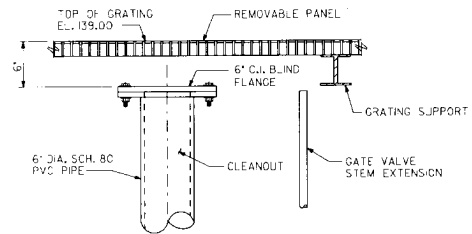
DETAIL 4
