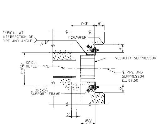
SECTIONAL ELEVATION
