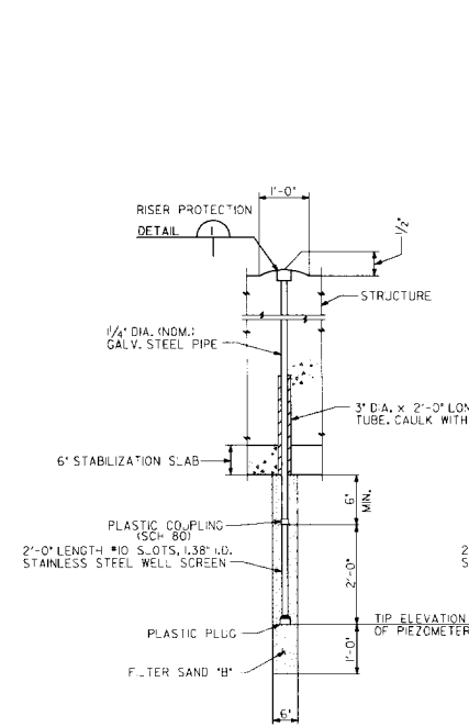
TYPE A PIEZOMETER
