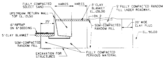
SECTION C
