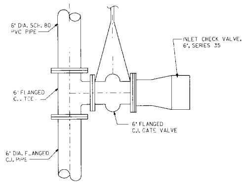
DETAIL 2
