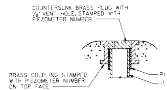
DETAIL
