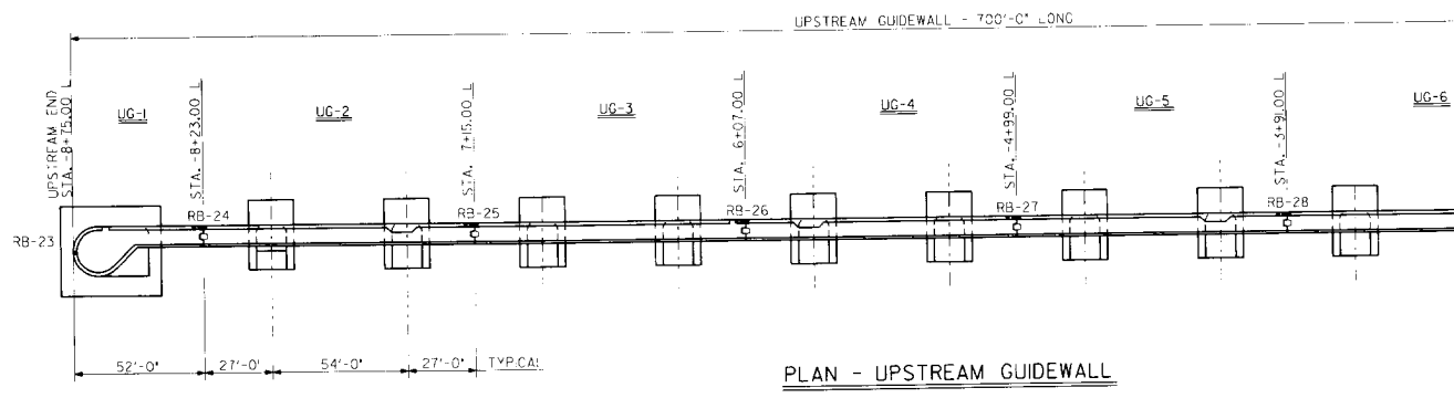
PLAN OF LOCK
