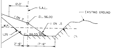
EXISTING CRAIN REVETMENT
