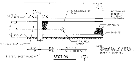
SECTION B
