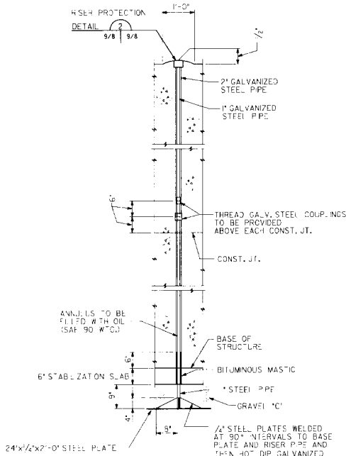
SETTLEMENT PLATE
