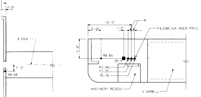
PLAN AT CREST GATE PIER
