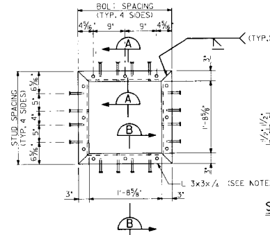
ELEVATION - SUPPORT FRAME
