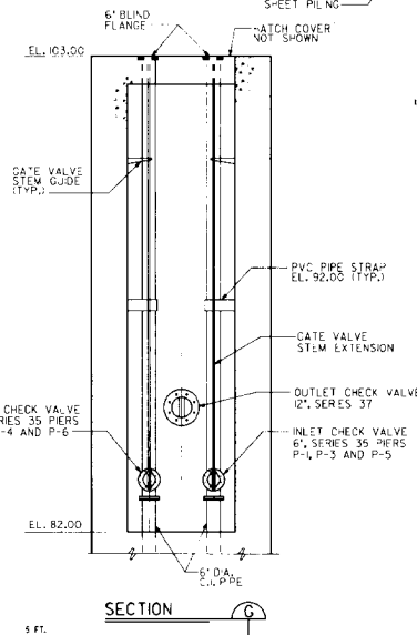
SECTION C
