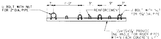
RISER PIPE SPACER DETAIL
