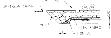
TRANSITION NO. 3A AND 4A TO UPSTREAM CHANNEL
