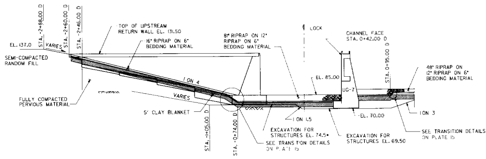
SECTION A
