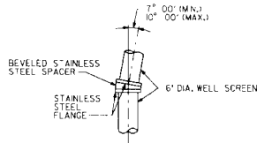
DETAIL 2
