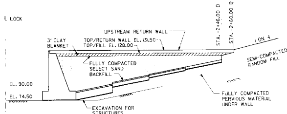
SECTION B
