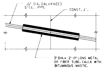
DETAIL D
