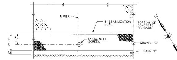
SECTION A NOTE: TYPICAL AT PIERS P-2 THRU P-5.
