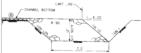
CHANNEL KEY DETAIL
