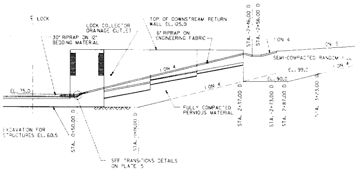
SECTION J
