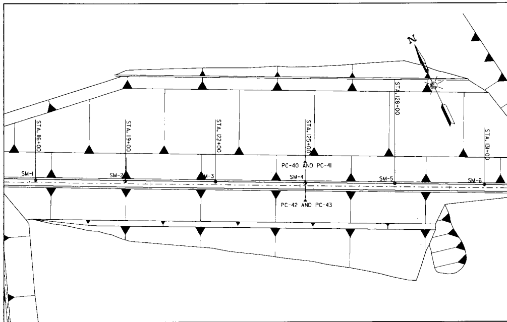
PLAN OF CLOSURE DAM
