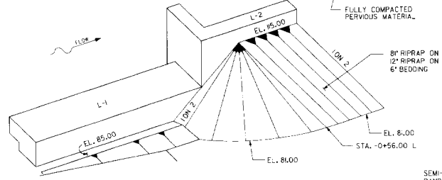
SECTION D
