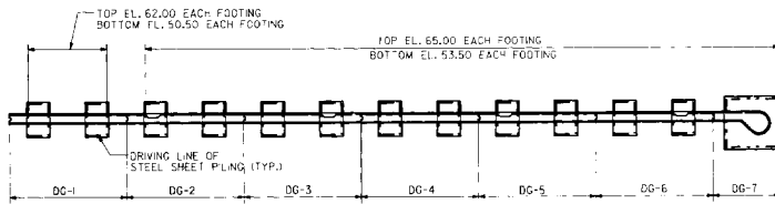
PLAN - DOWNSTREAM GUIDEWALL
