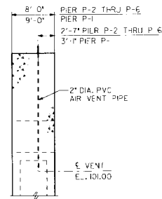
SECTION C
