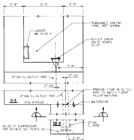
PARTIAL PLAN - MANHOLE AT PIER P-8
