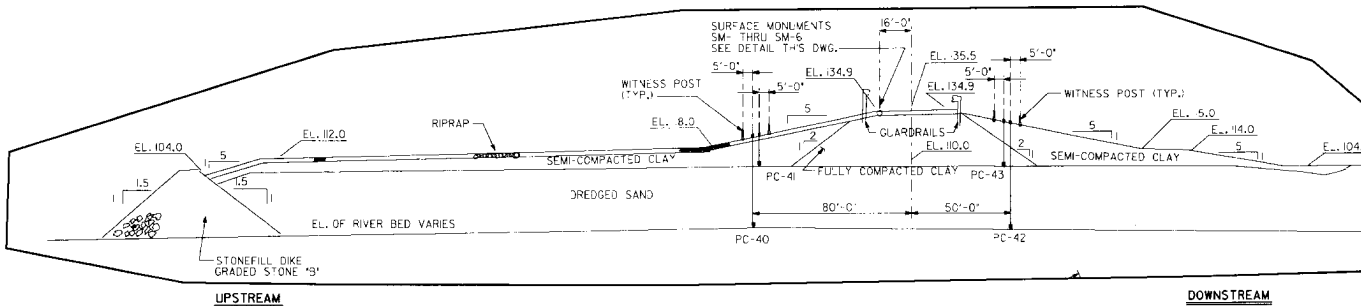
SECTION THRU CLOSURE DAM
