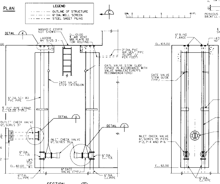
SECTION
