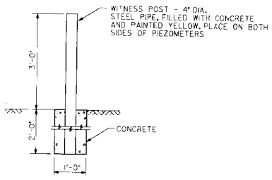
WITNESS POST
