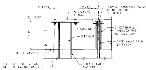
DETAIL 4
