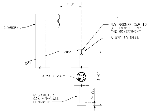
SURFACE MONUMENT DETAIL
