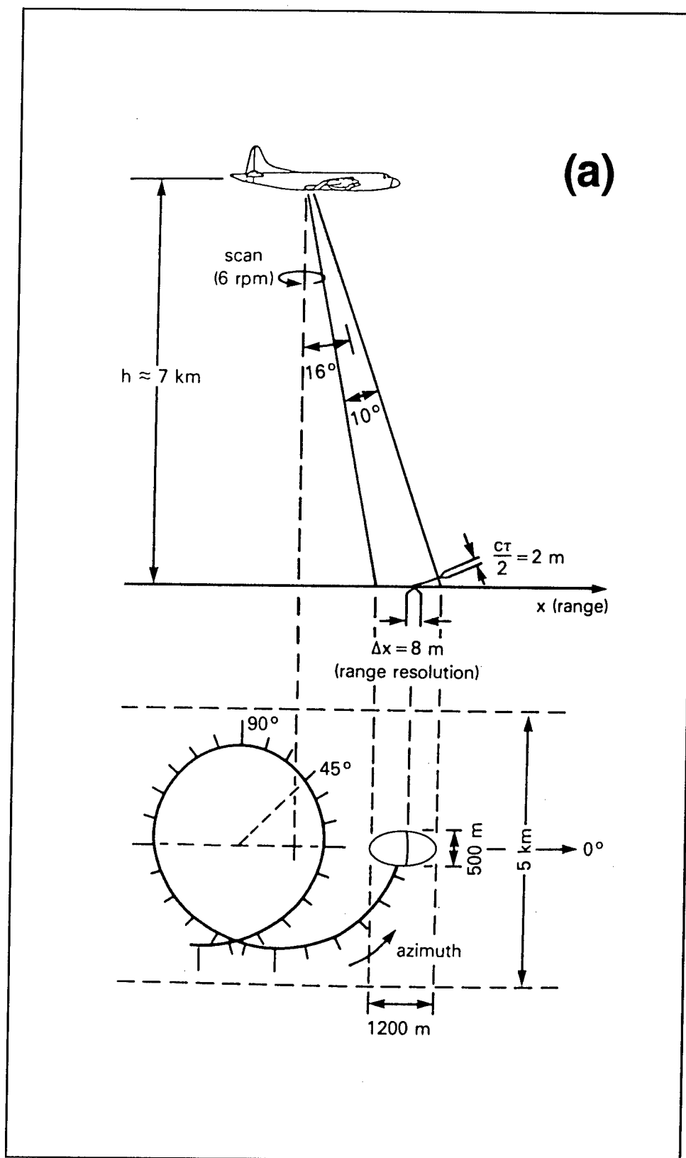
Figure 3. Radar Ocean Wave Spectrometer (ROWS) measurement geometry, (a) spectrometer ('S') mode (Continued)
