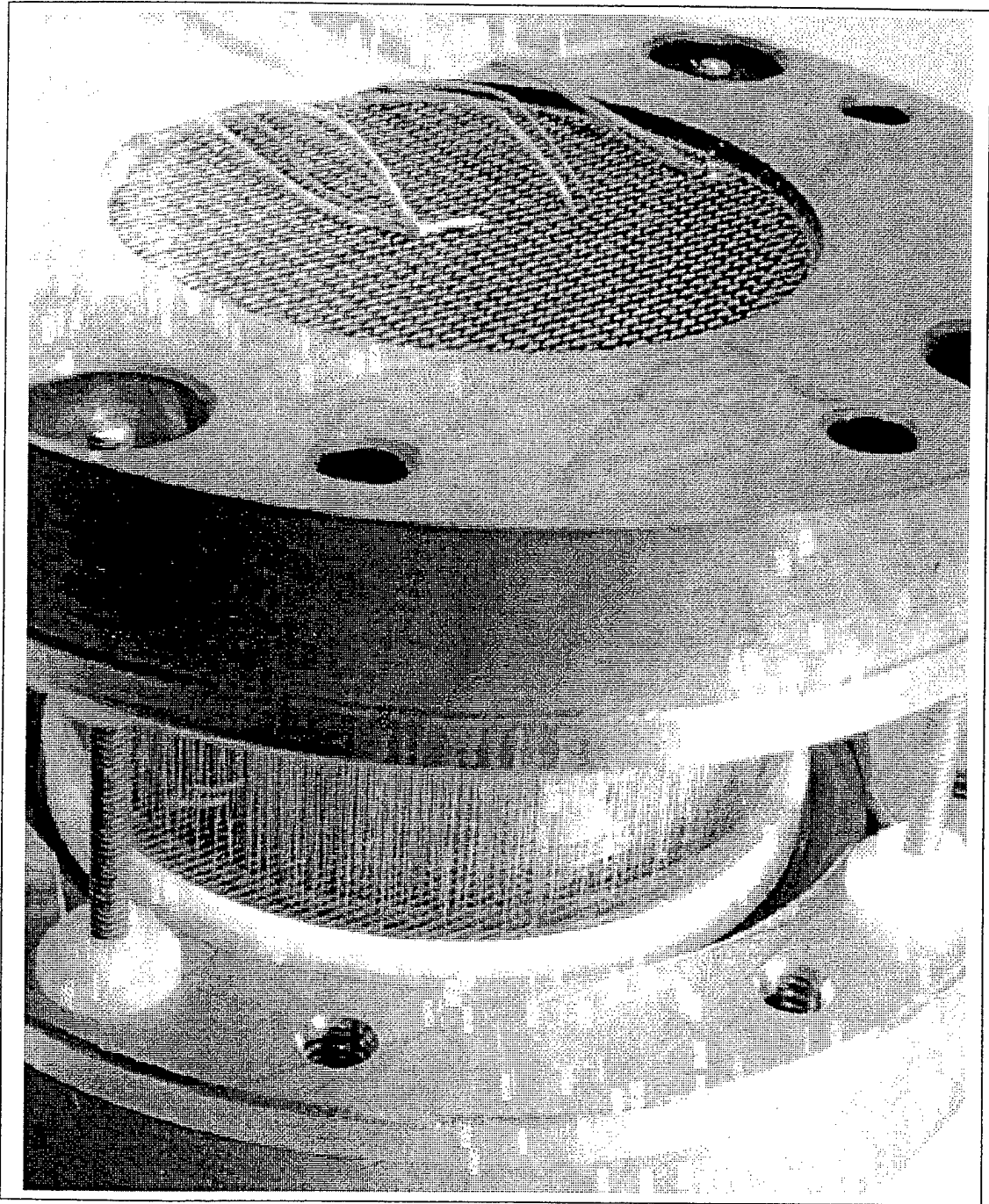
Figure 3. Pin Stack.
