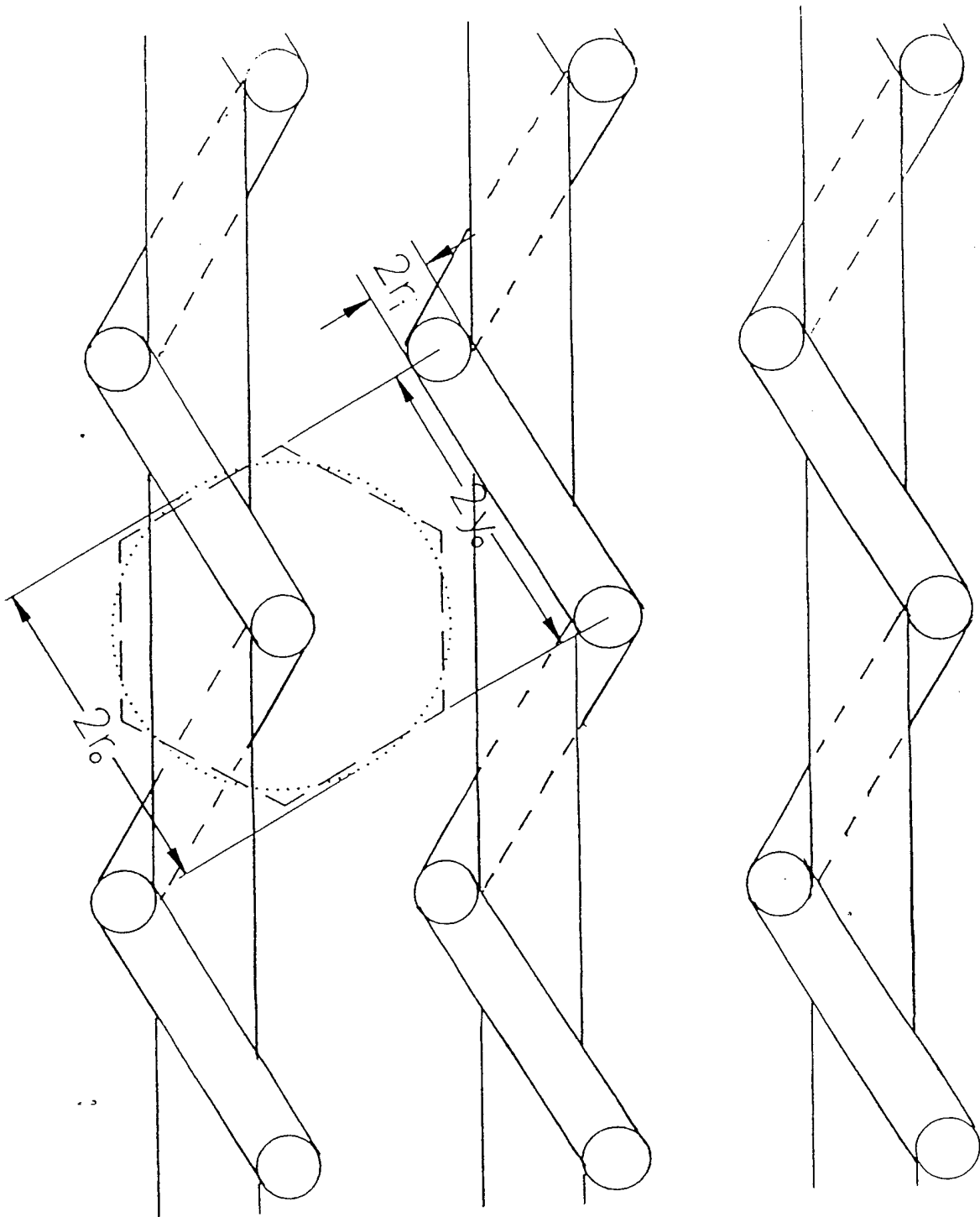
Figure 1. Pin Stack Geometry, from Nessler(1994).
