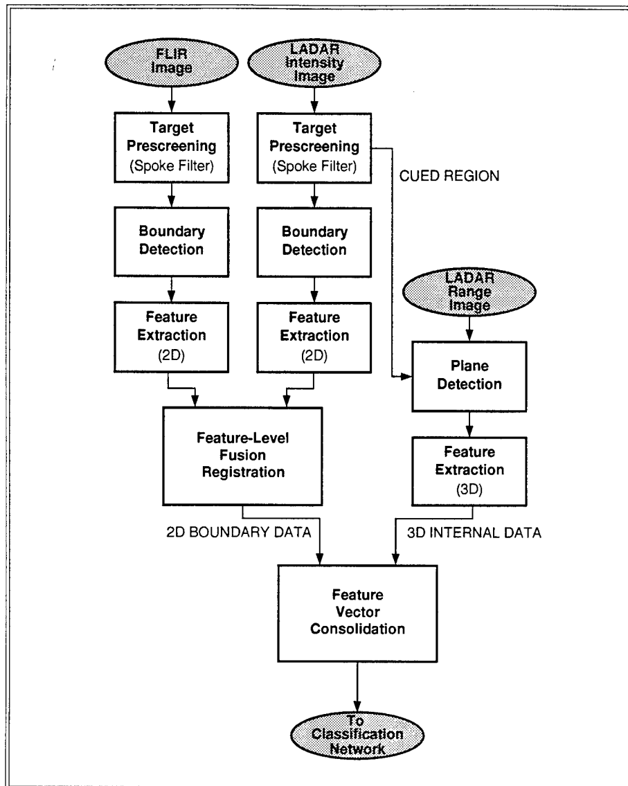
Figure 13. The proposed preprocessing and feature extraction approach for the enhanced, FLIR/LADAR ATD/I system fuses FLIR and LADAR data on a feature level. See Figure 23 for the overall system diagram.
