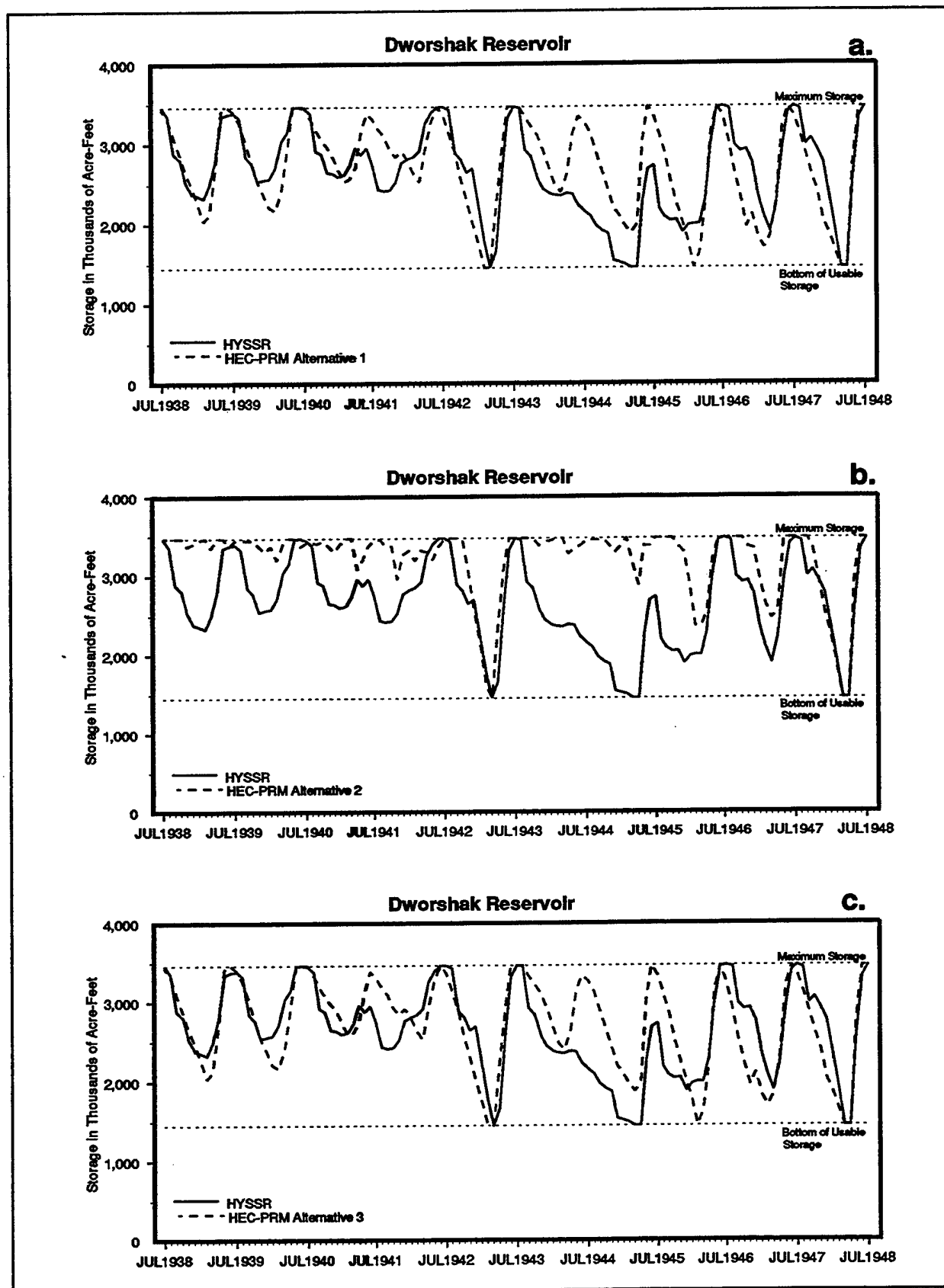
FIGURE F.12 1938 - 1948 Storage at Dworshak: HYSSR & Alternatives
