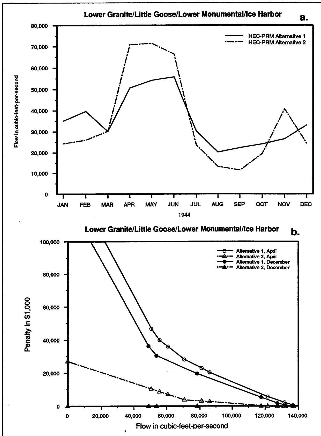
FIGURE 4.7 Penalty Function at Granite: Alternatives 1 & 2
