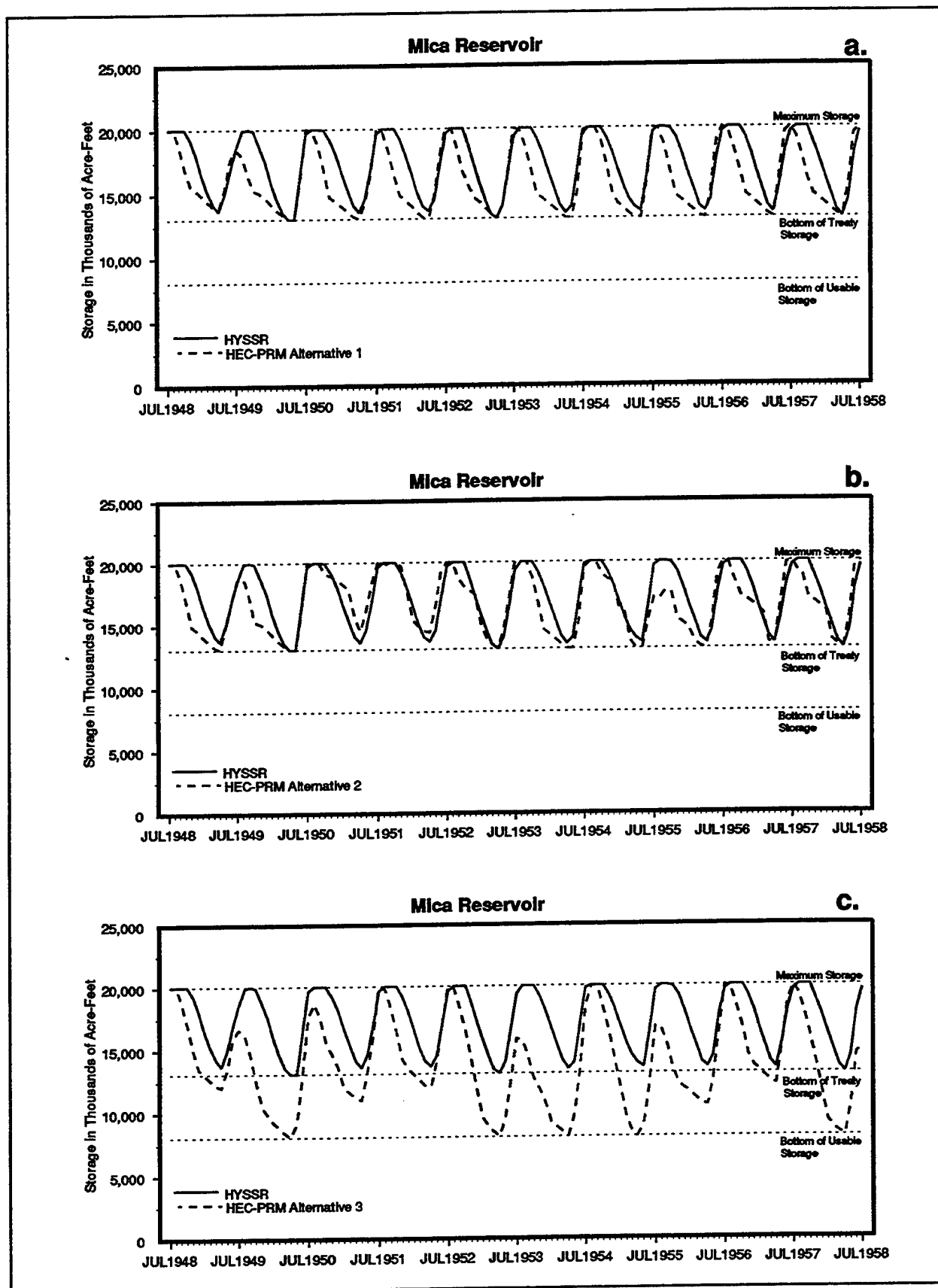
FIGURE F.3 1948 - 1958 Storage at Mica: HYSSR & Alternatives
