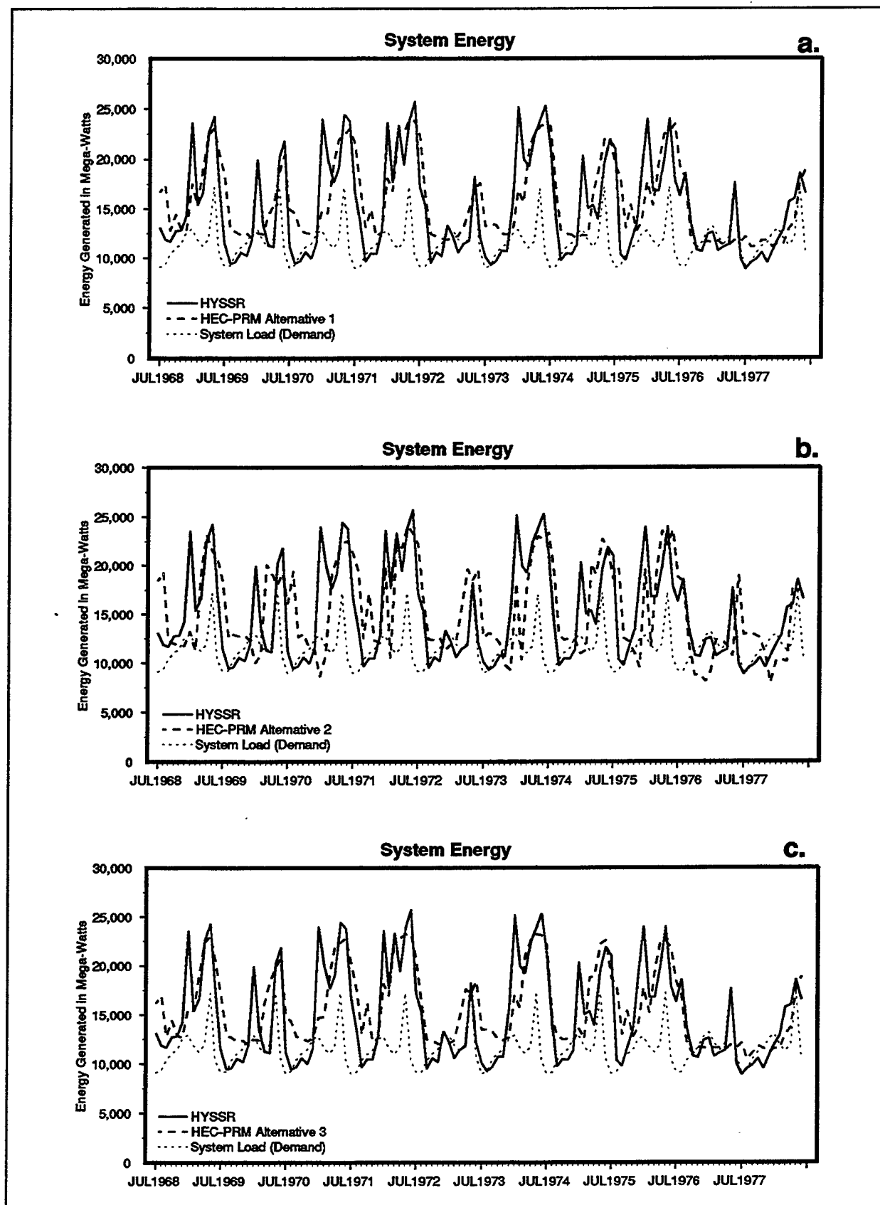
FIGURE G.5 1968 - 1978 System Generated Energy: HYSSR & Alternatives
