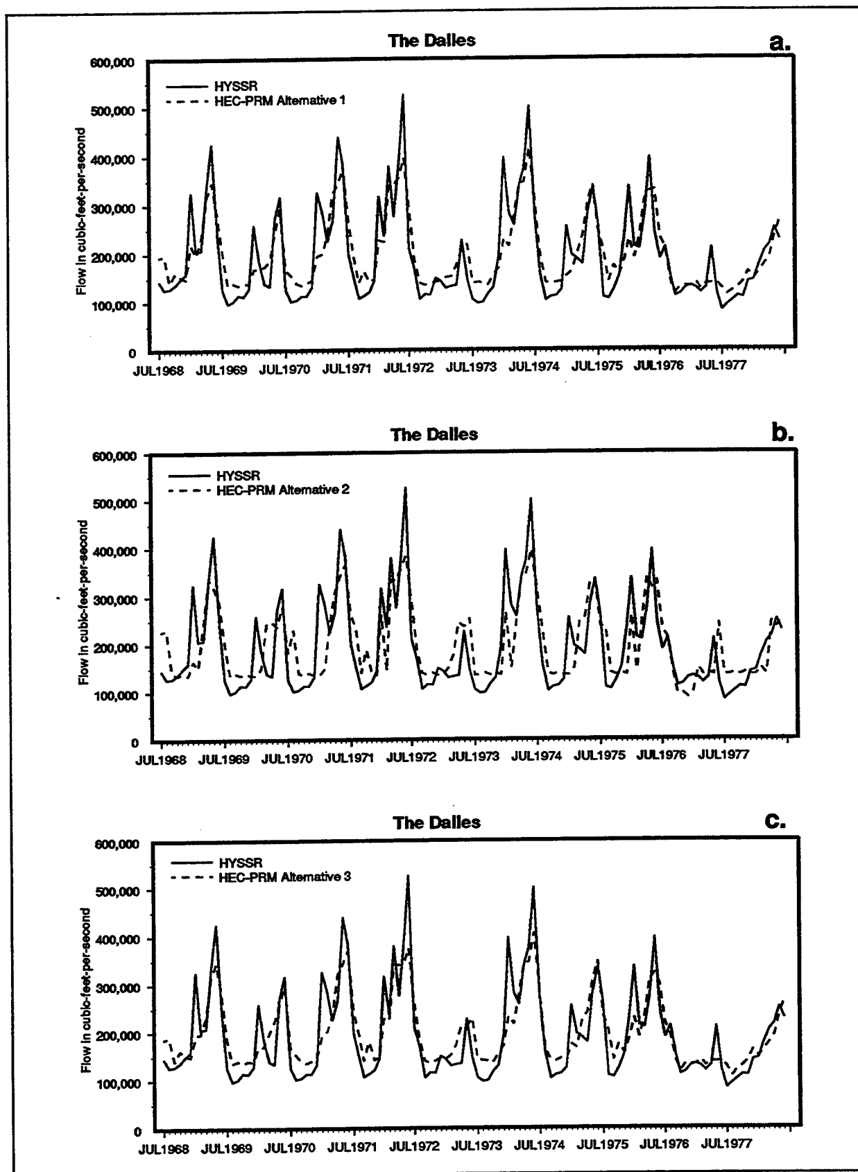
FIGURE F.20 1968 - 1978 Flow at The Dalles: HYSSR & Alternatives
