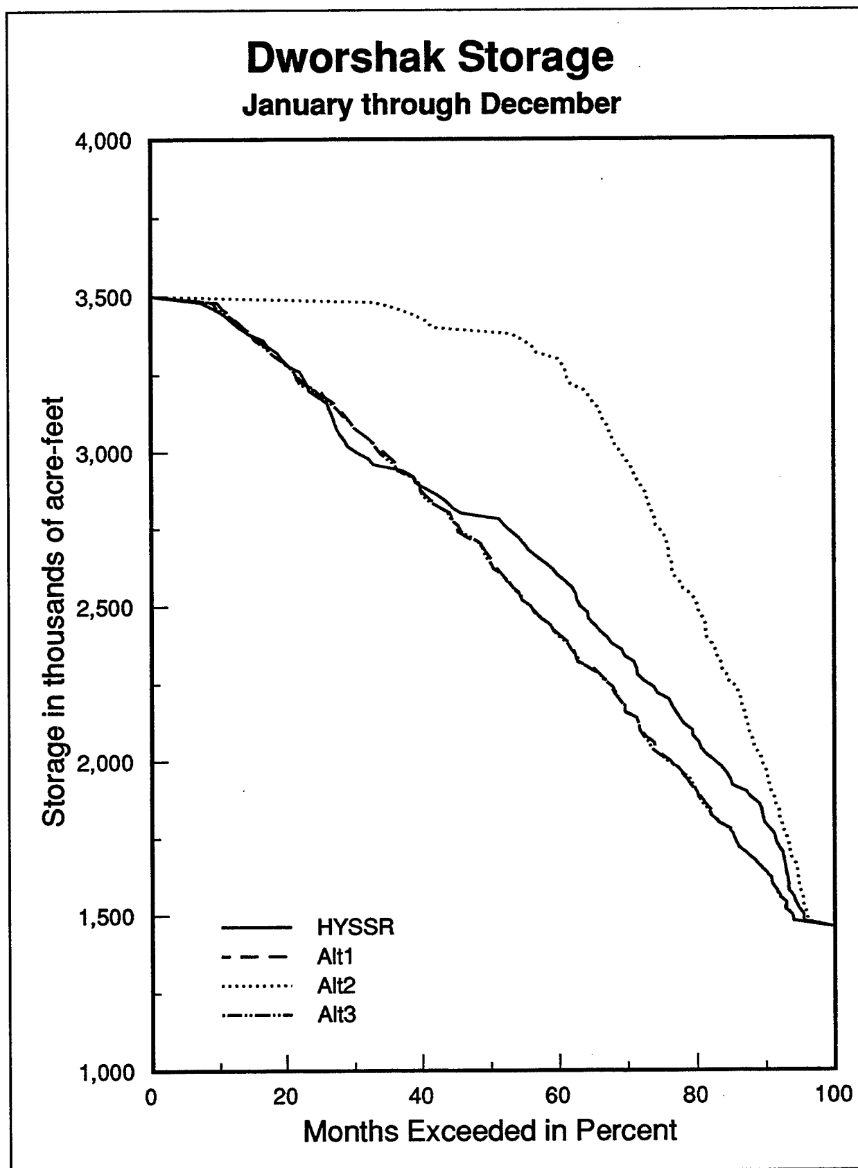
FIGURE 4.8 Exceedance Frequency for Dworshak Storage (January - December)
