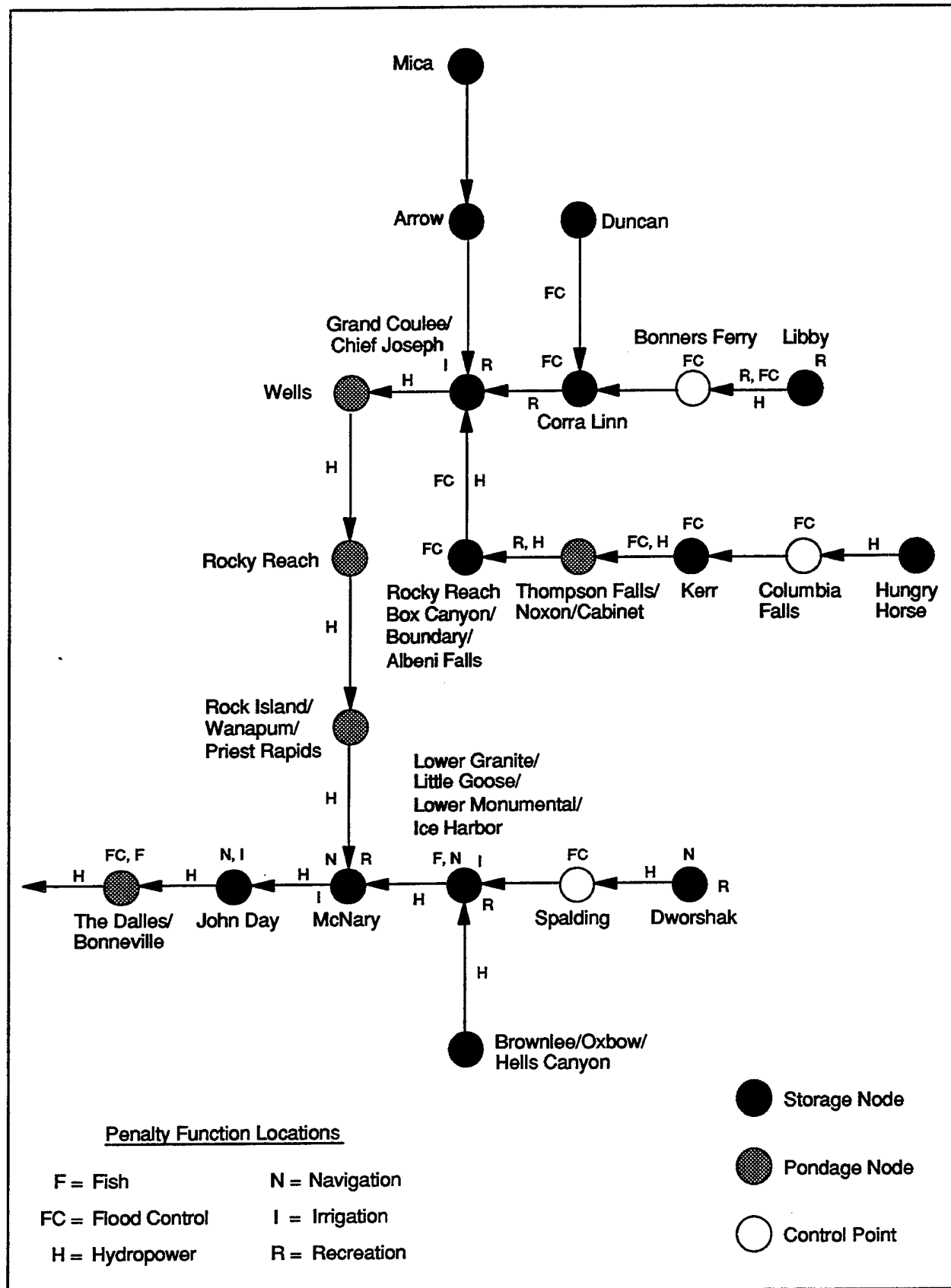
FIGURE 3.1 Single-period Network Model of Columbia River System
