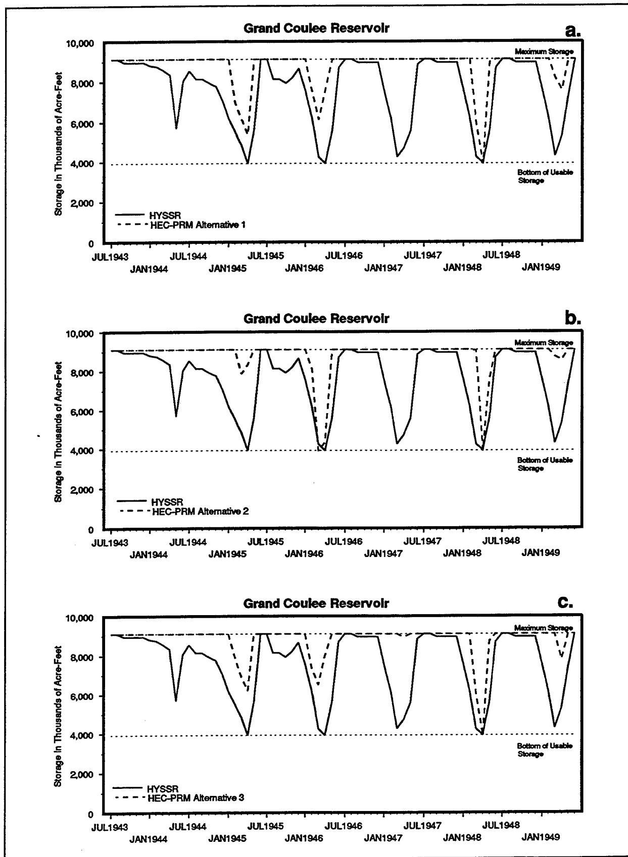
FIGURE 4.3 1943 - 1949 Storage at Grand Coulee: HYSSR & Alternatives
