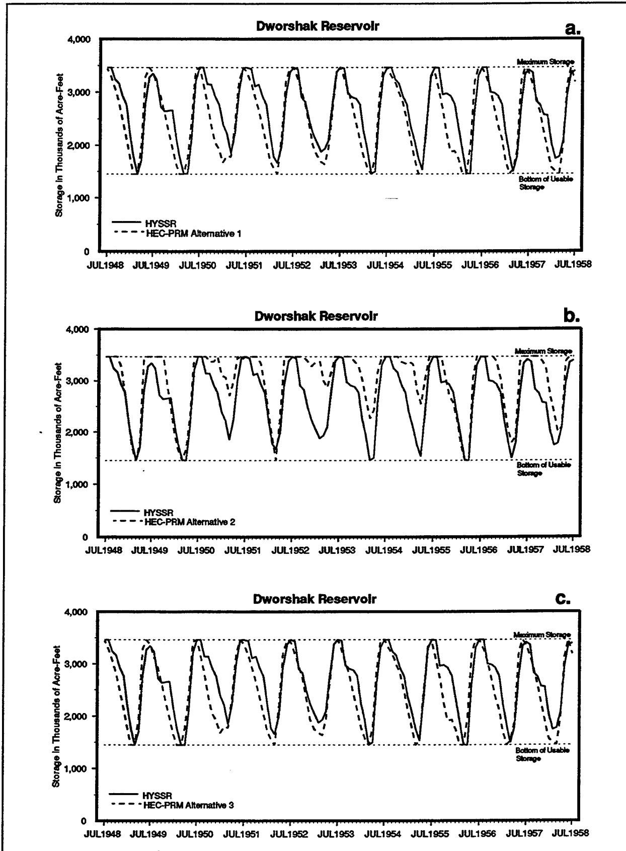
FIGURE F.13 1948 - 1958 Storage at Dworshak: HYSSR & Alternatives
