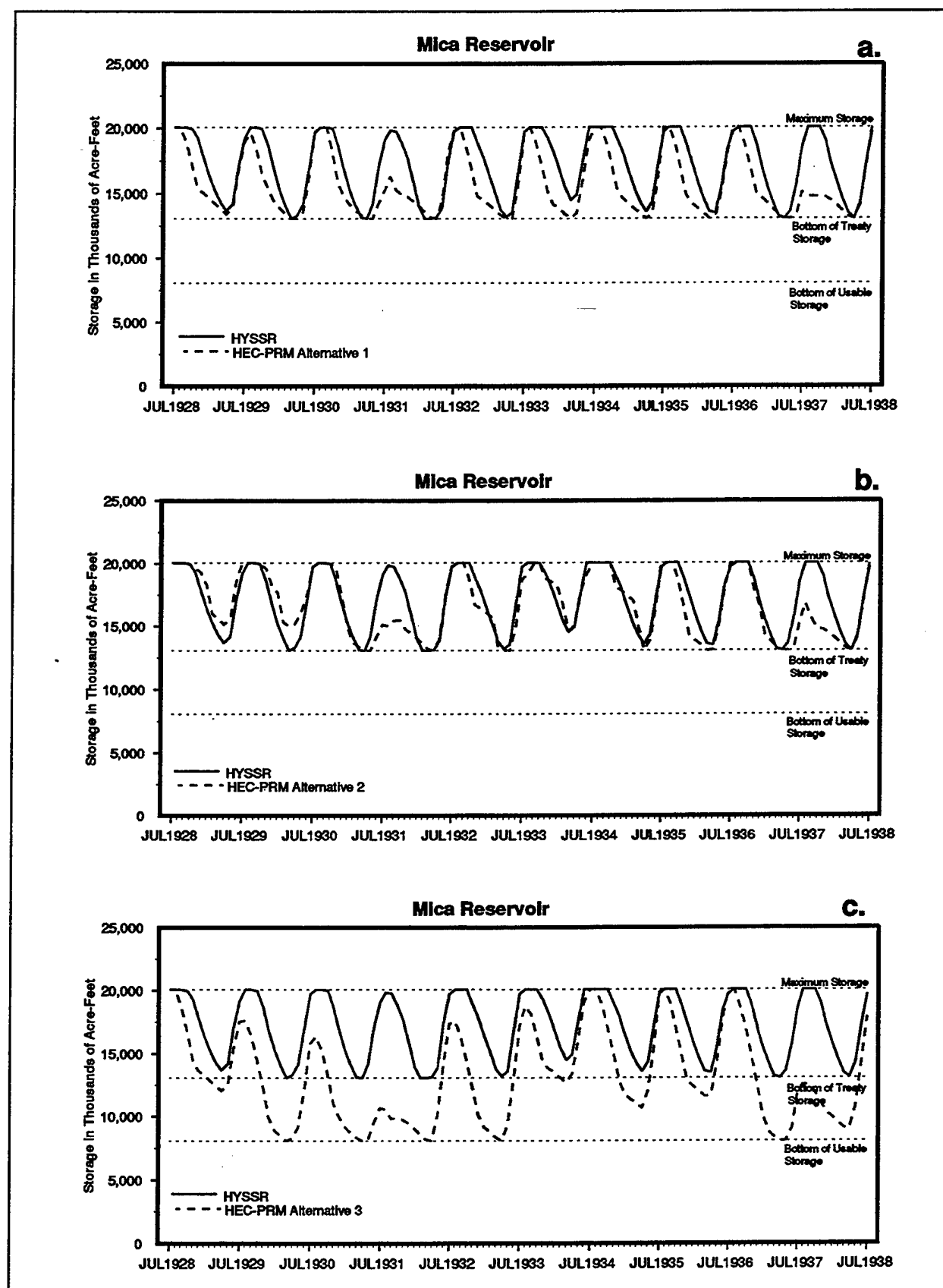
FIGURE F.1 1928 - 1938 Storage at Mica: HYSSR & Alternatives
