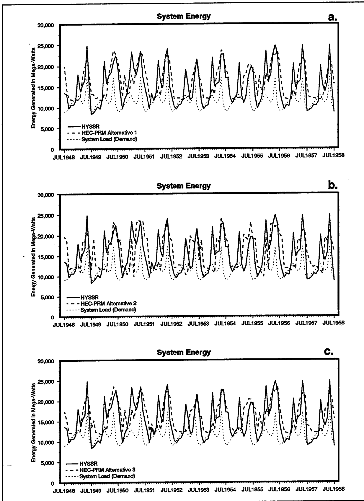
FIGURE G.3 1948 - 1958 System Generated Energy: HYSSR & Alternatives
