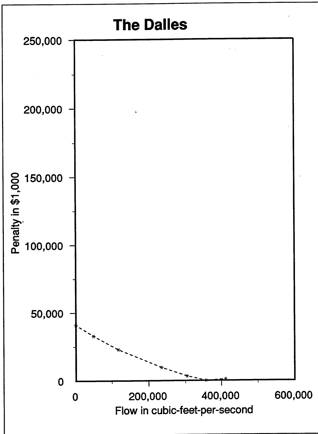
FIGURE E.10 The Dalles Hydropower Penalty Function
