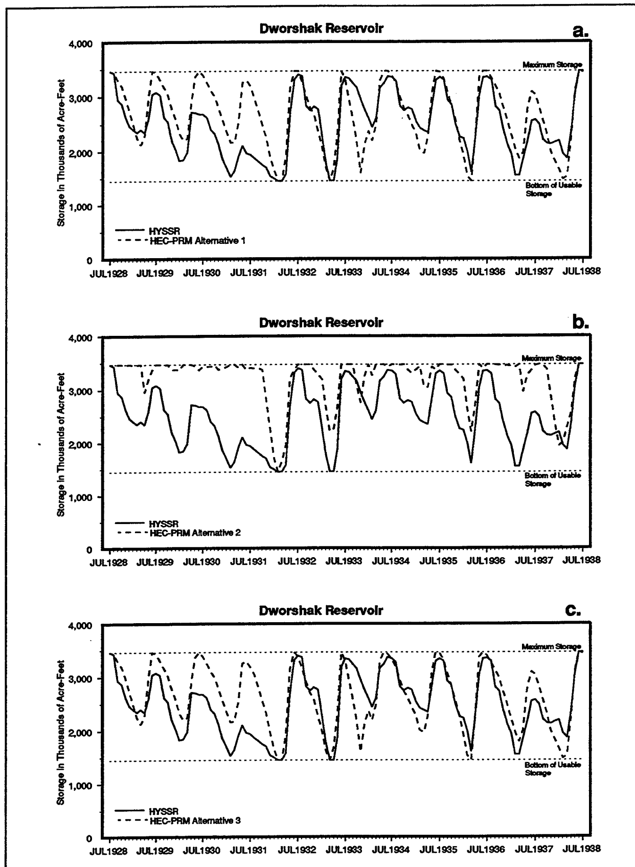
FIGURE F.11 1928 - 1938 Storage at Dworshak: HYSSR & Alternatives
