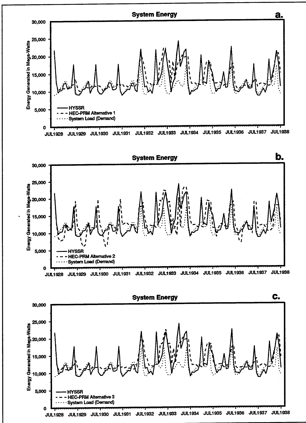
FIGURE G.1 1928 - 1938 System Generated Energy: HYSSR & Alternatives
