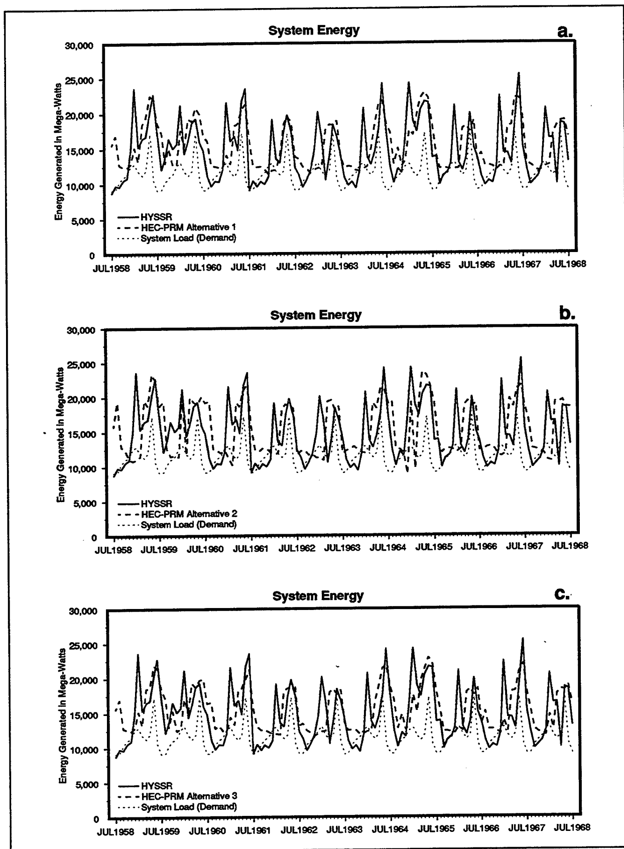
FIGURE G.4 1958 - 1968 System Generated Energy: HYSSR & Alternatives
