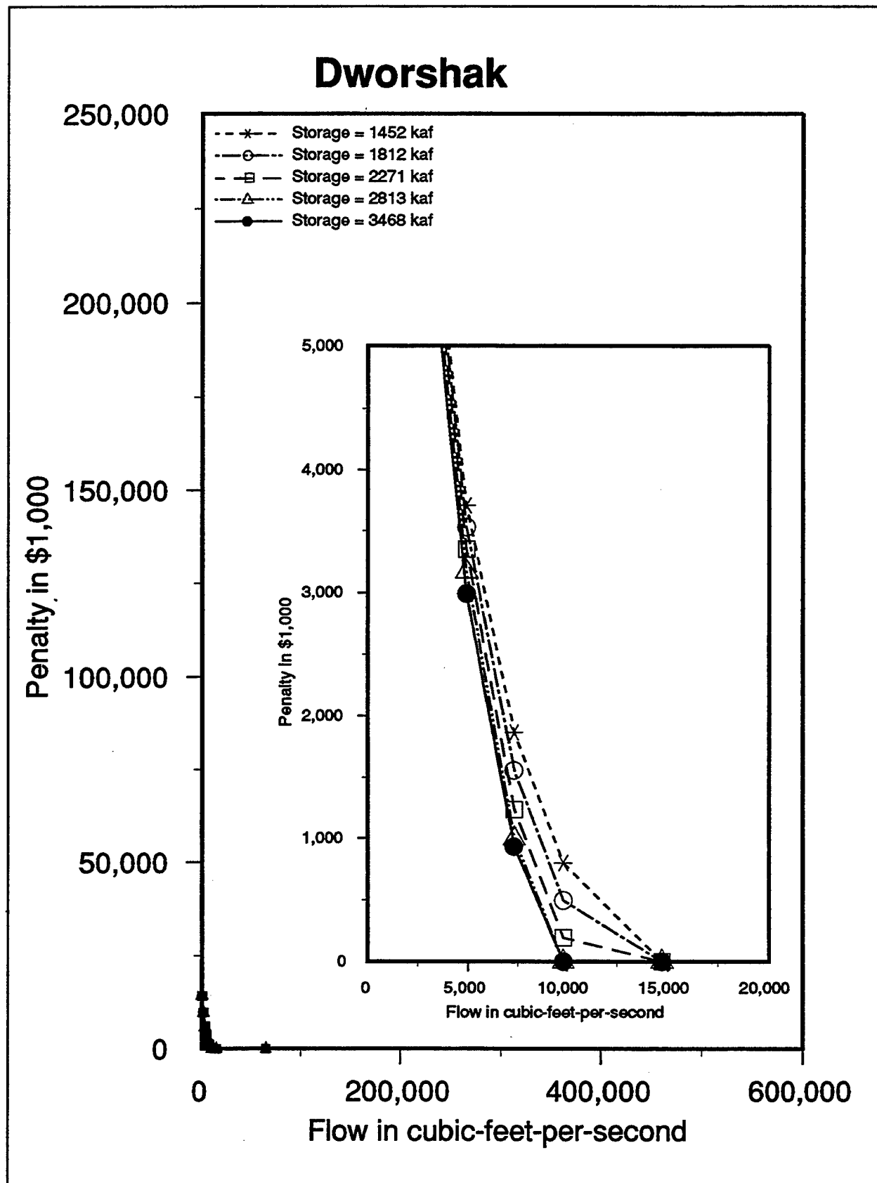
FIGURE E.8 Dworshak Hydropower Penalty Functions
