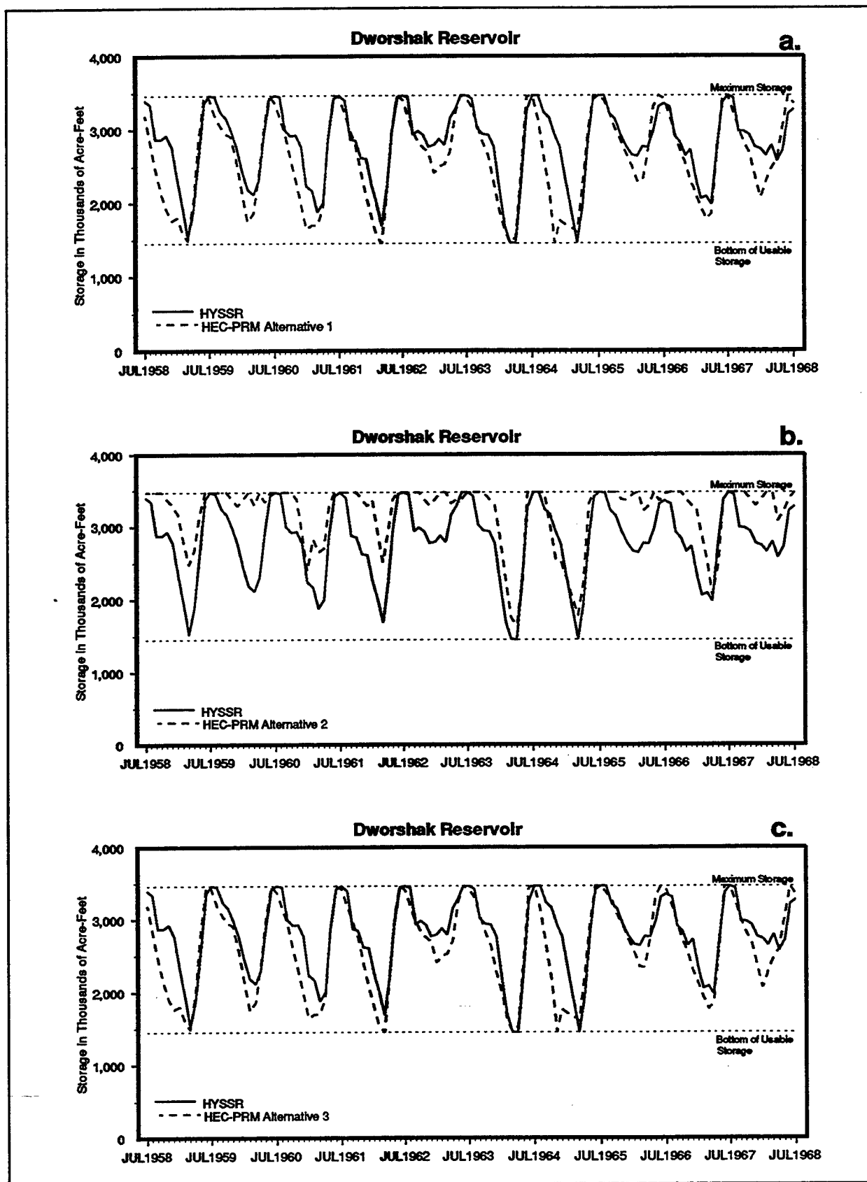
FIGURE F.14 1958 - 1968 Storage at Dworshak: HYSSR & Alternatives
