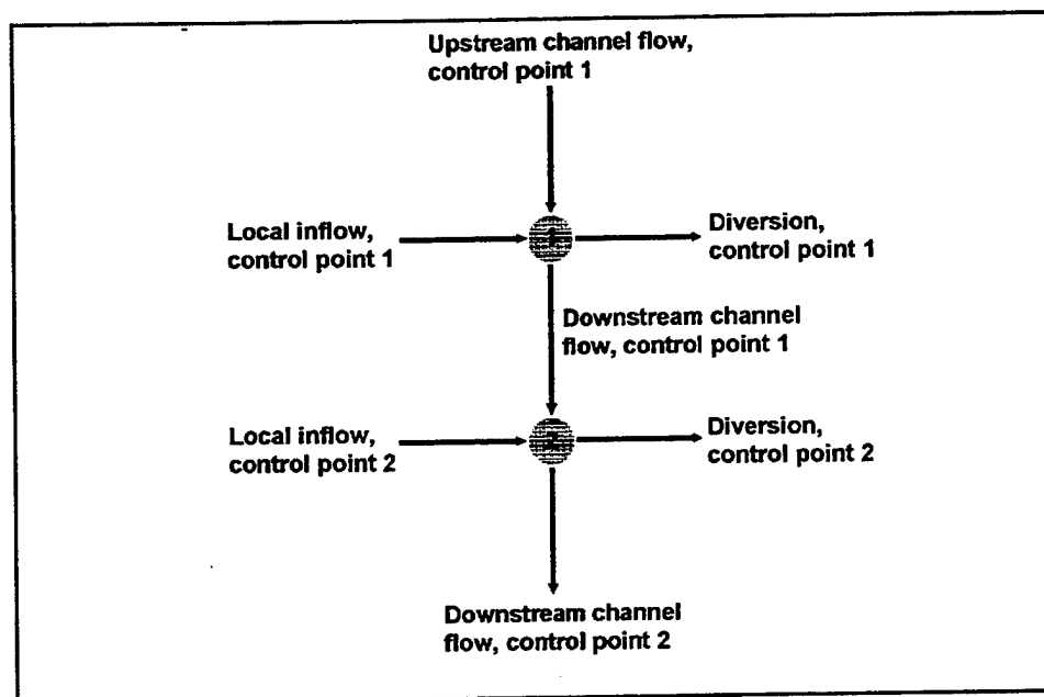
FIGURE A.4 Multiple Control-point Channel Mass Continuity Representation
