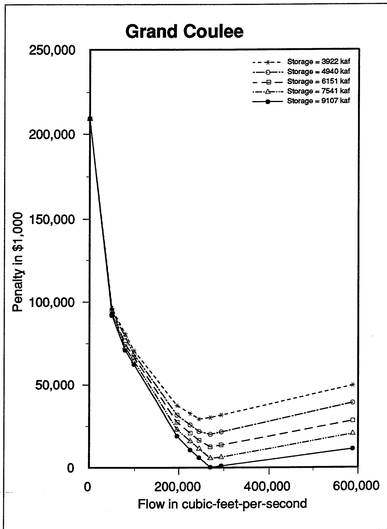
FIGURE E.7 Grand Coulee Hydropower Penalty Functions
