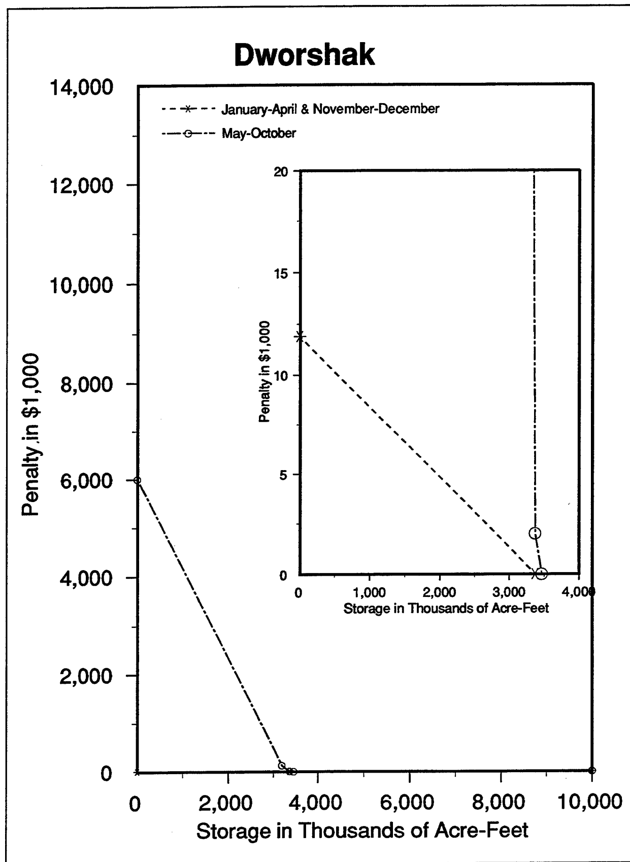
FIGURE E.3 Dworshak Storage Penalty Functions
