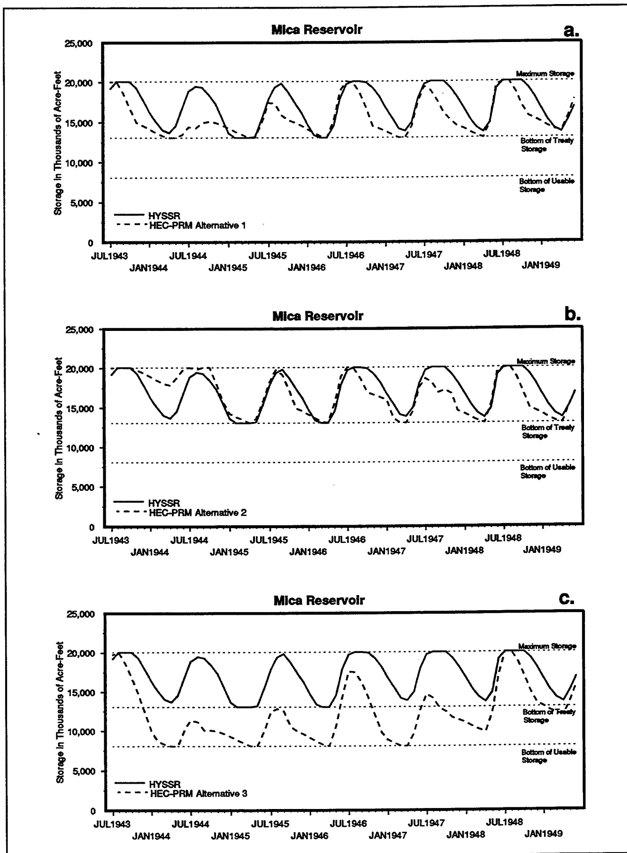
FIGURE 4.2 1943 - 1949 Storage at Mica: HYSSR & Alternatives
