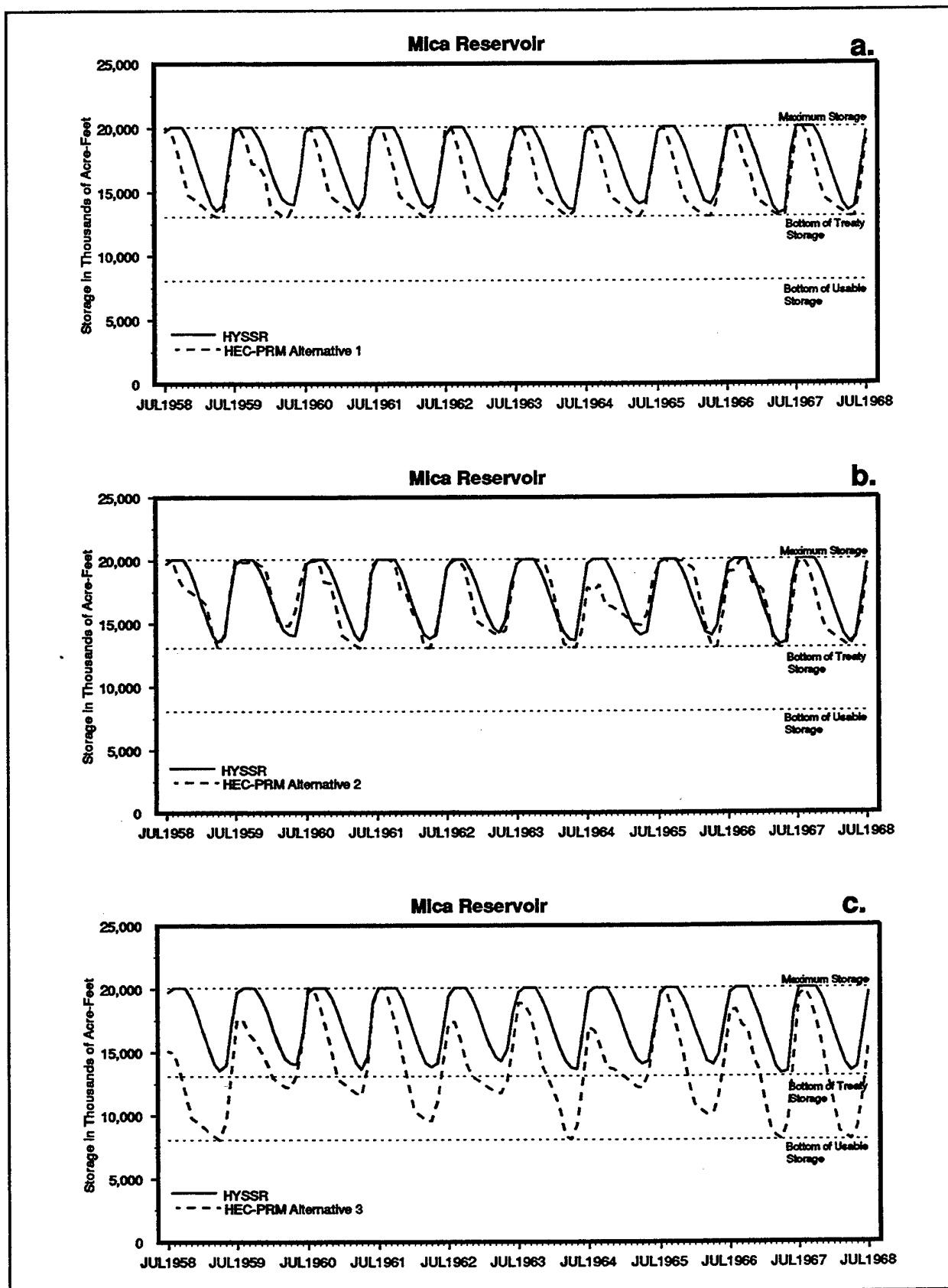
FIGURE F.4 1958 - 1968 Storage at Mica: HYSSR & Alternatives
