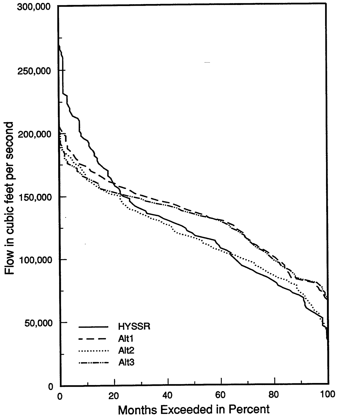
FIGURE 4.6 Exceedance Frequency for Grand Coulee Releases, Fish-flow Season (April - July)
