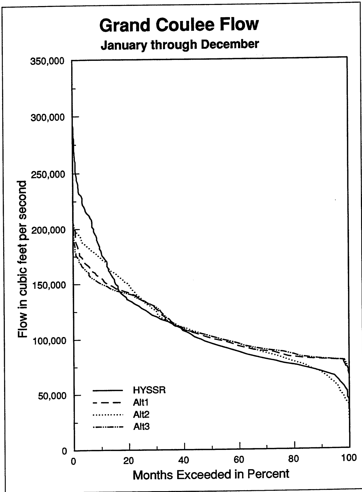
FIGURE 4.5 Exceedance Frequency for Grand Coulee Releases (January - December)
