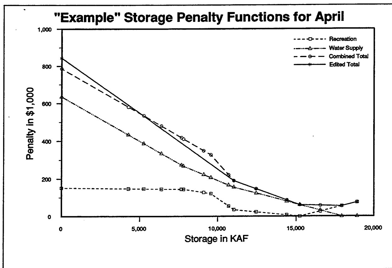
FIGURE 3.2 How Penalty Functions are Combined and Approximated
