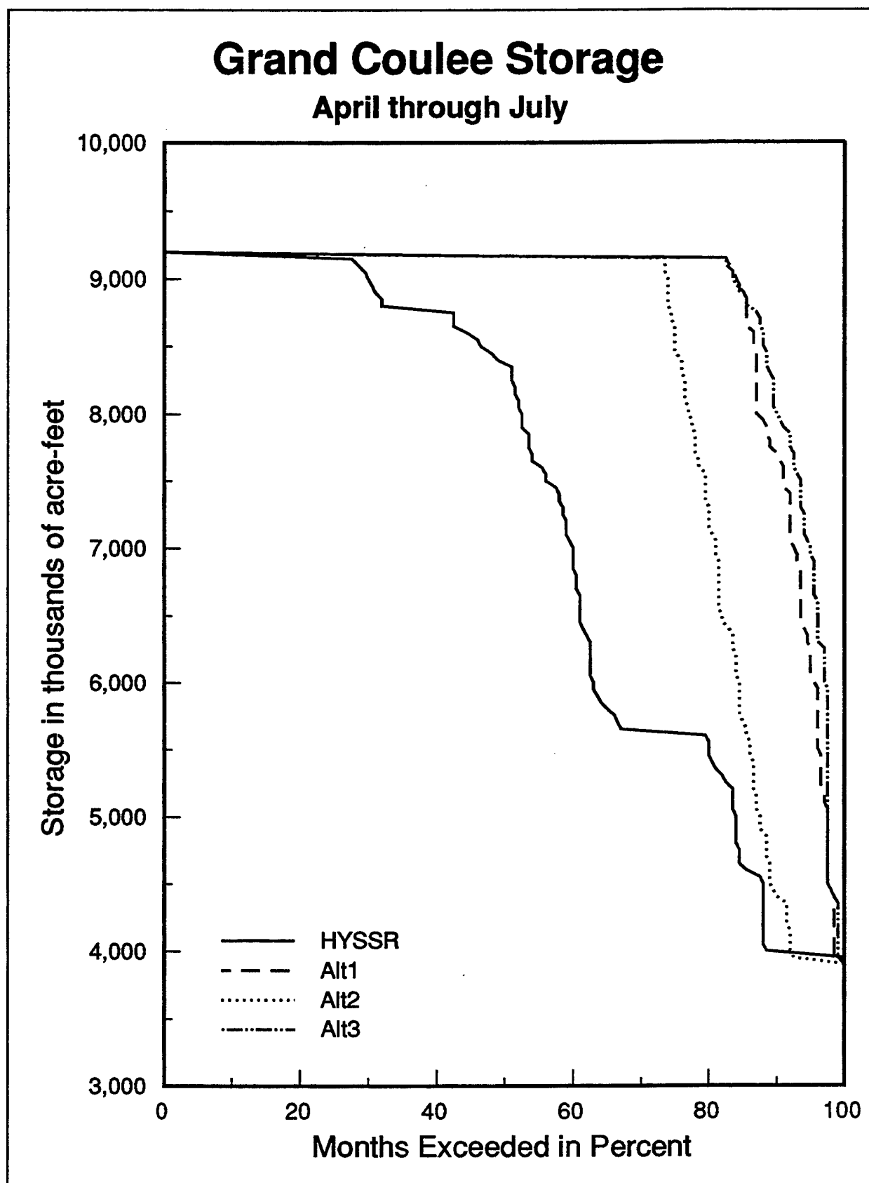
FIGURE 4.4 Percent Time Exceedance for Grand Coulee Storage (April - July)
