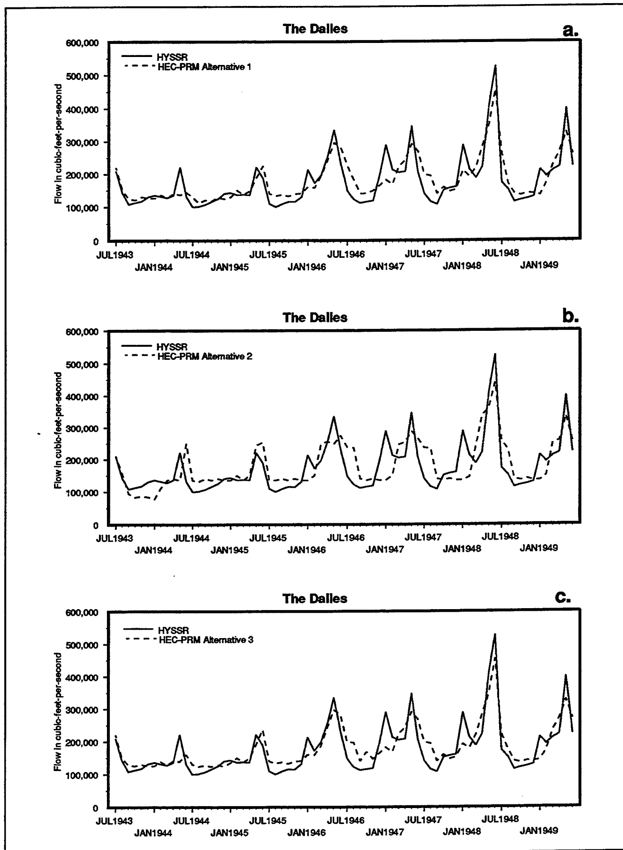
FIGURE 4.10 1943 - 1949 Flow at The Dalles: HYSSR & Alternatives
