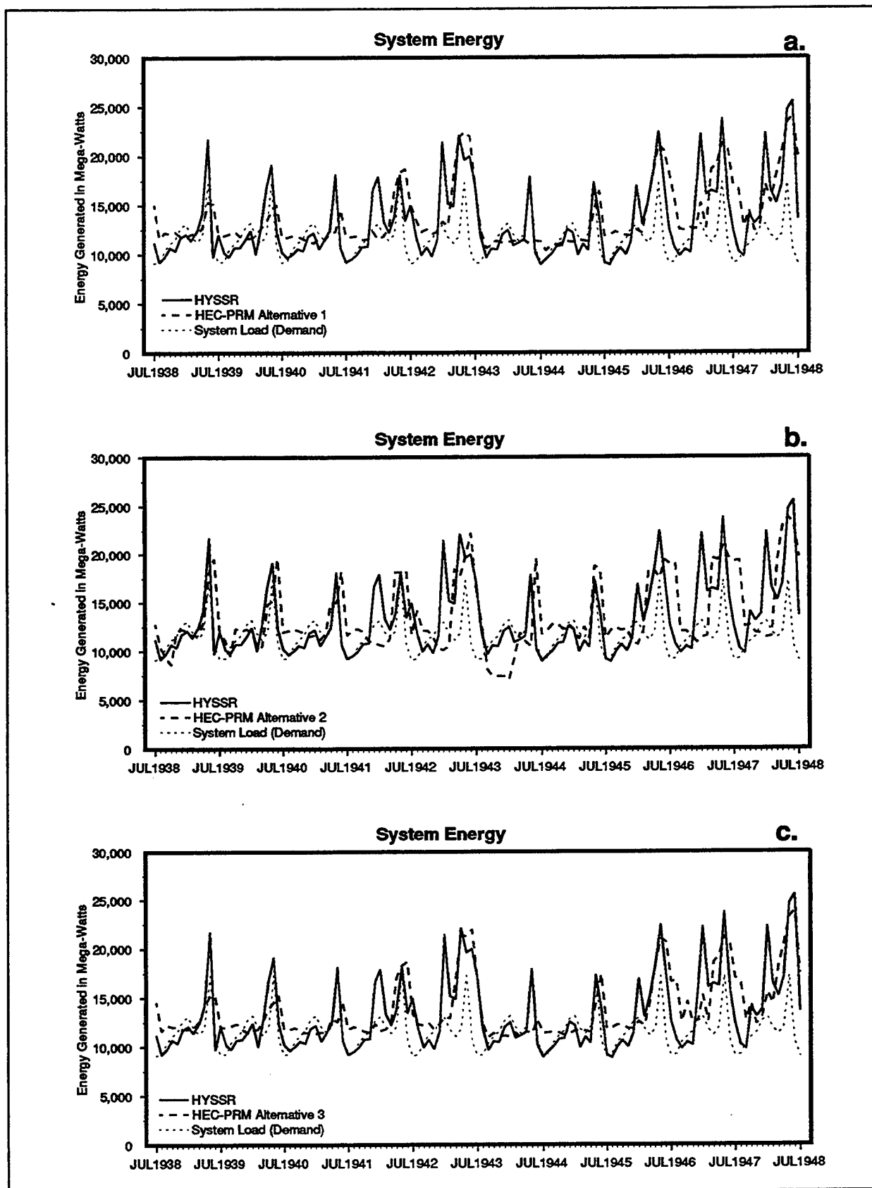
FIGURE G.2 1938 - 1948 System Generated Energy: HYSSR & Alternatives
