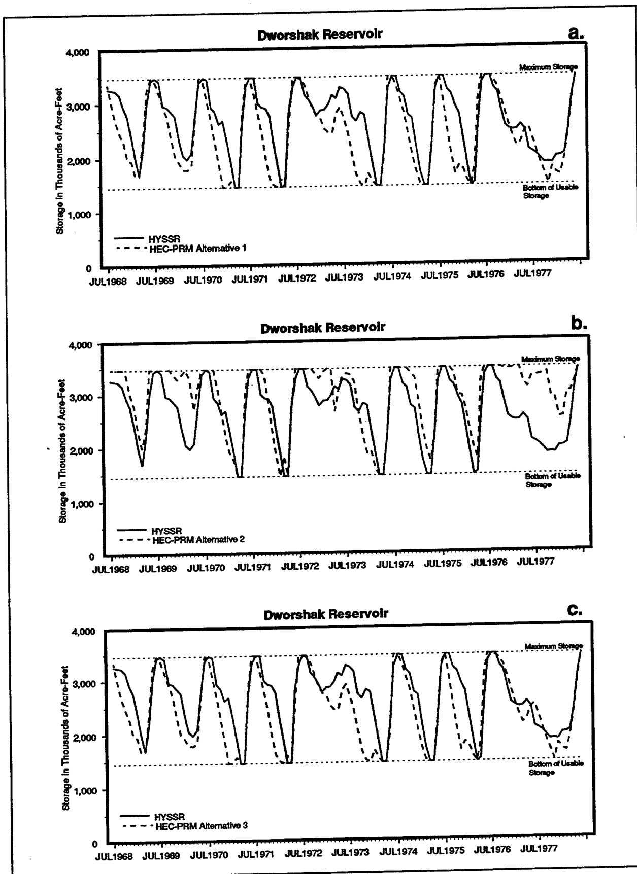
FIGURE F.15 1968 - 1978 Storage at Dworshak: HYSSR & Alternatives
