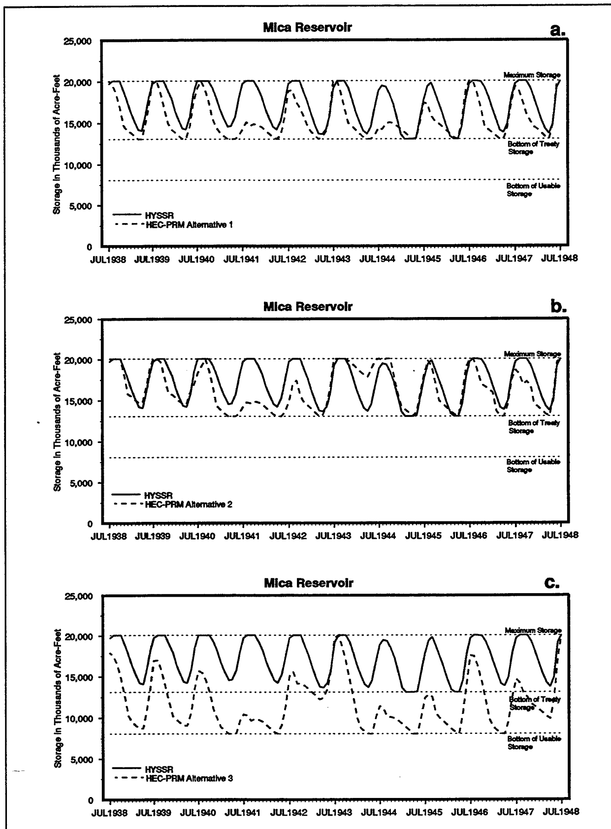
FIGURE F.2 1938 - 1948 Storage at Mica: HYSSR & Alternatives
