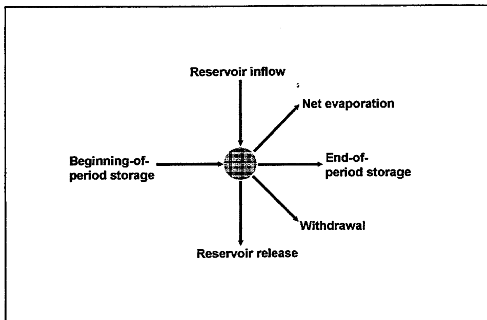
FIGURE A.1 Single-period Reservoir Mass Continuity Representation
