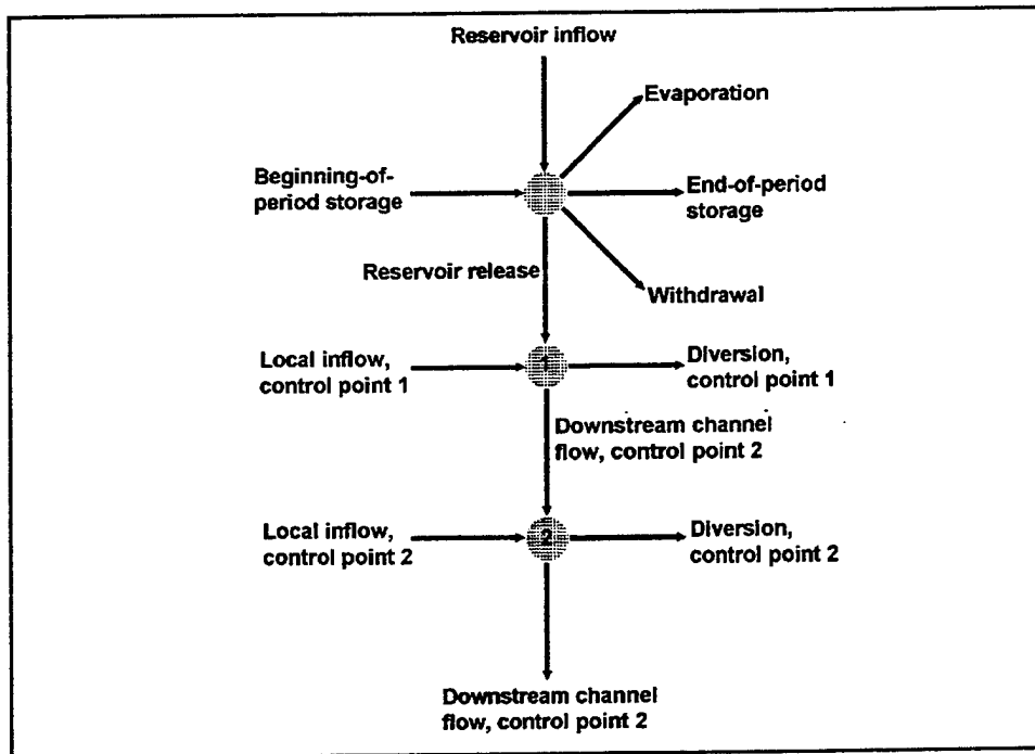
FIGURE A.5 Reservoir System Representation for Single Period
