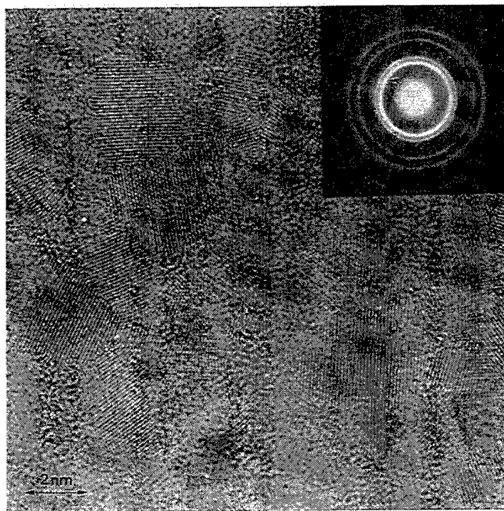
Fig. 2. The typical microstructure of a high flux Au-Pd film deposited on a carbon substrate: the quasi-continuous, polycrystalline nature of the film as opposed to discrete 3D islands in Fig. 1 is apparent; a twinned particle is arrowed and denoted by "T". The inset diffraction pattern shows sharp rings of polycrystalline Au-Pd domains; note also the stronger intensity of the Au-Pd(111) ring (arrowed).
