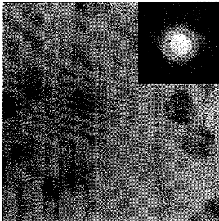
Fig. 1. The typical microstructure of a low flux Au-Pd film deposited on a carbon substrate: three-dimensional (3D) islands comprising of single crystals and multiply twinned particles; "T" arrows show twins in the latter. The inset diffraction pattern of the region in the image shows diffuse rings corresponding to the small sizes of these particles; the (111) ring of Au-Pd is arrowed for reference.
