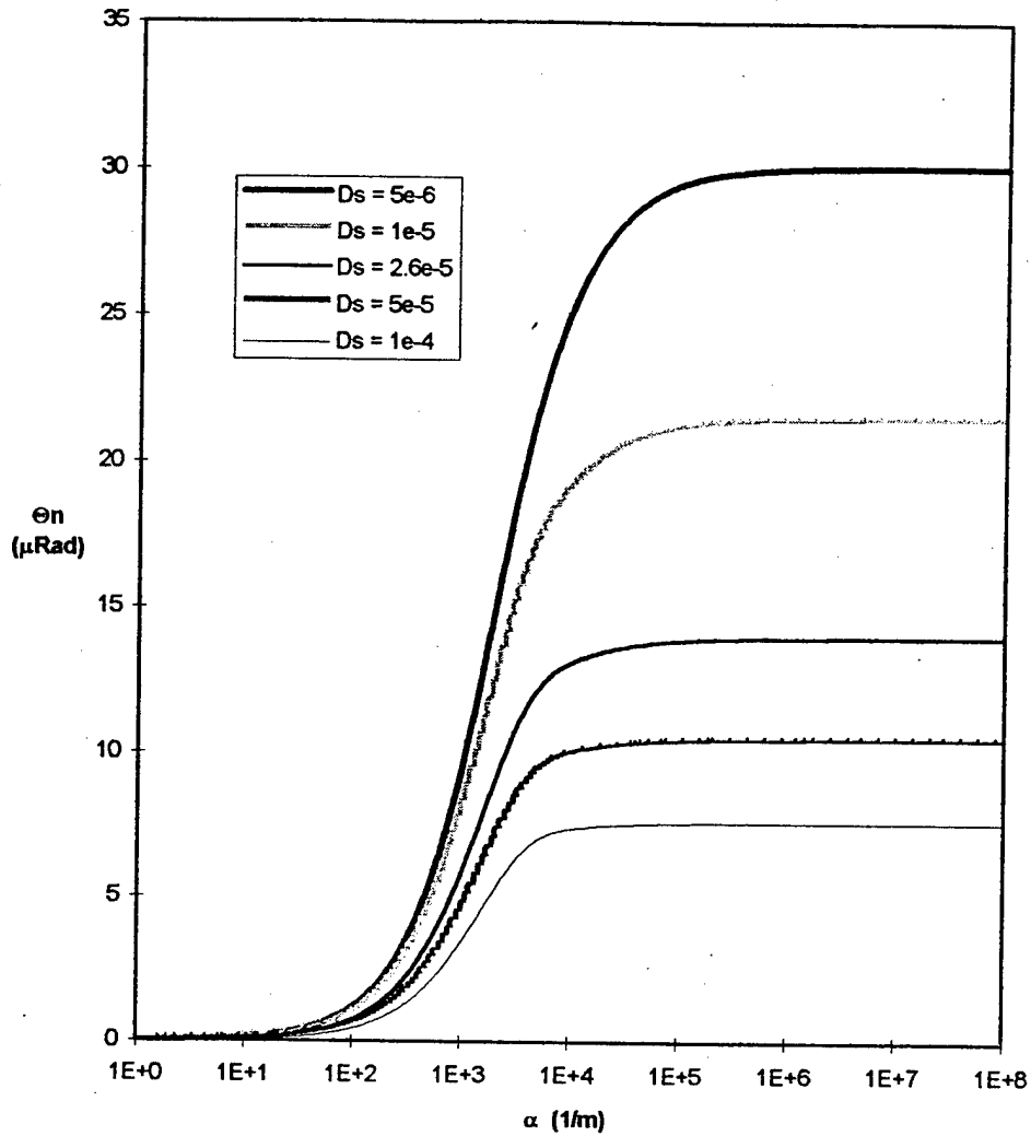
Fig. 6 Normal deflection versus the absorption coefficient with different values for the sample thermal diffusion constant and CCl 4 as the fluid.
