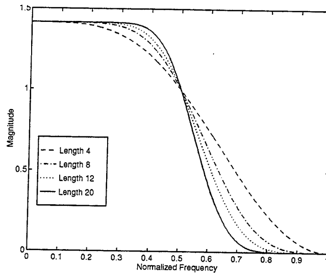
FIGURE 28. Frequency Response Plots for Filters of Length 4, 8, 12, and 20
