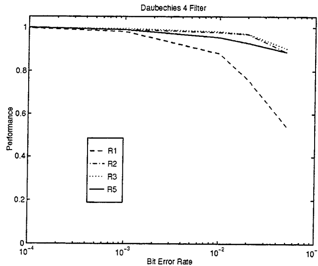
FIGURE 25. Performance with Length 4 Daubechies Filter on Binary Image
