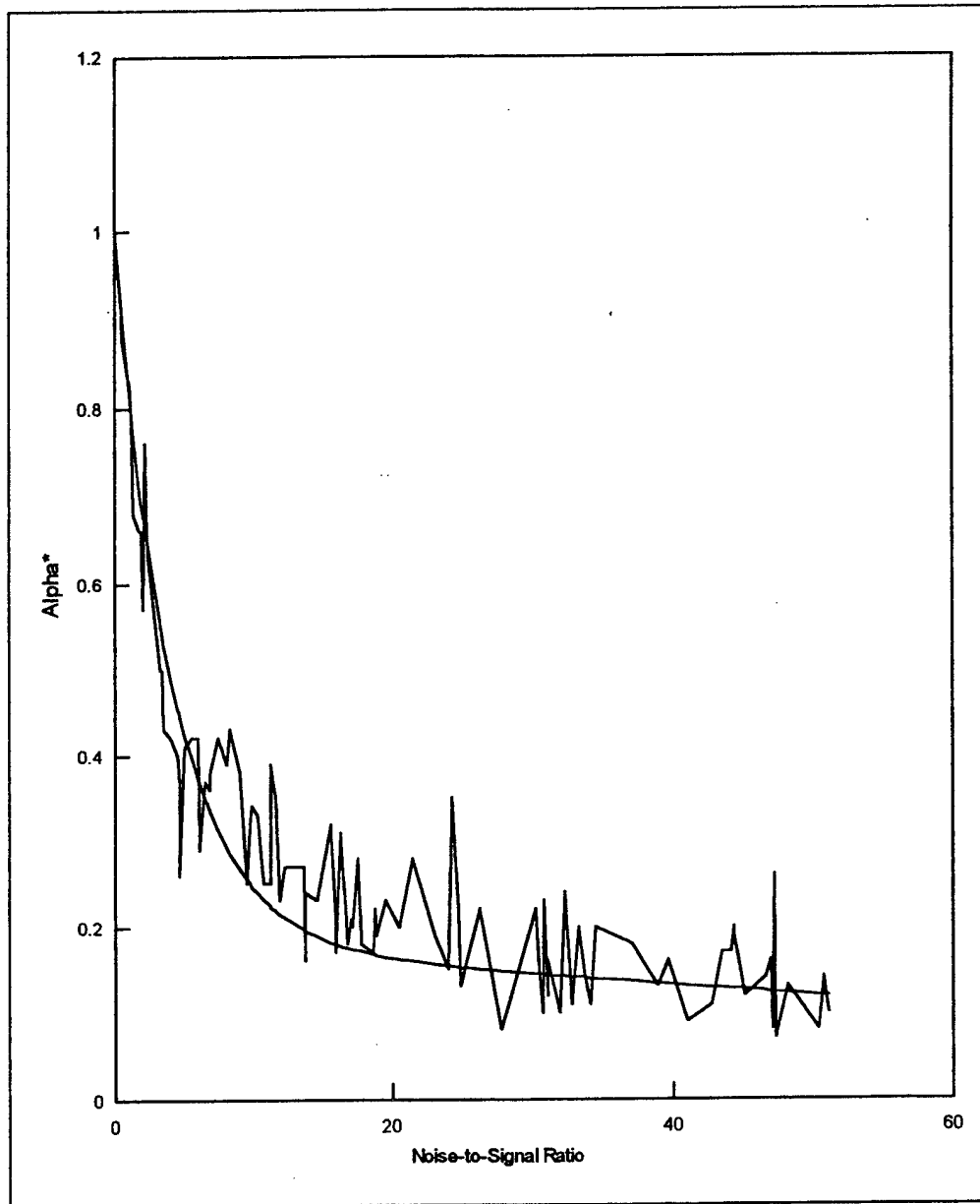
Equation to Estimate Alpha* Given the Noise-to-Signal Ratio
