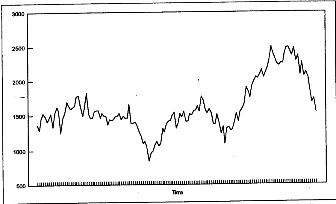
No Trend or Seasonality
