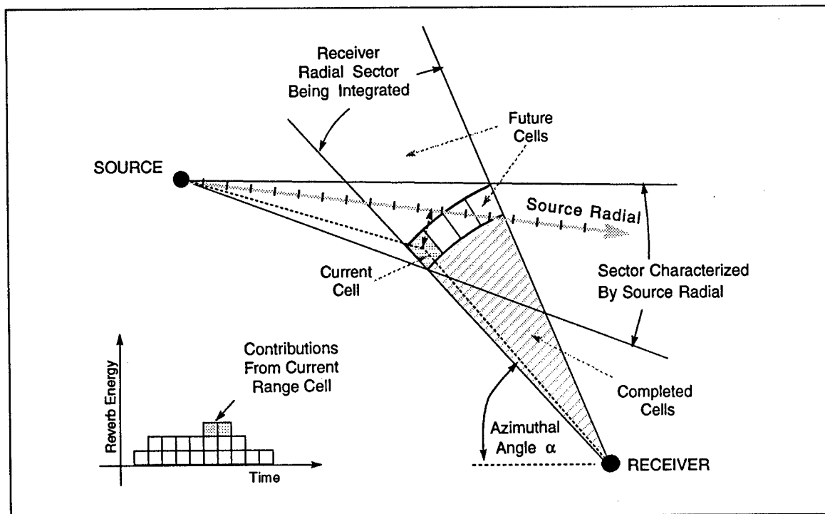
Fig. 13 – Integration procedure for calculating reverberation due to scattering along an angular sector. The angle \alpha measures the direction of arrival of the reverberation relative to an arbitrary coordinate reference.
