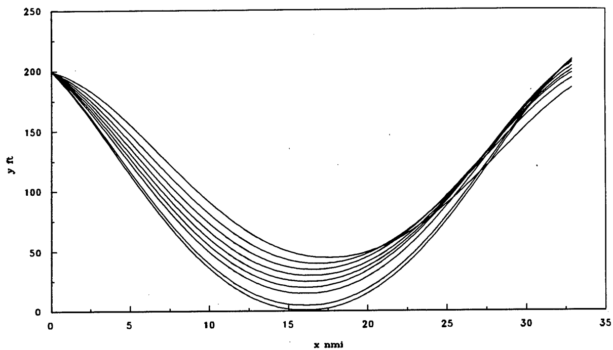
Figure 3. Interior Mirage Rays
