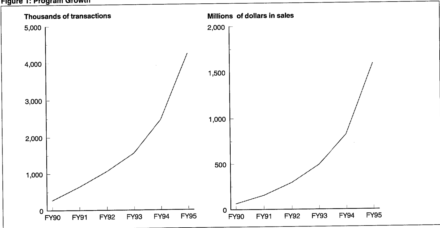
Figure 1: Program Growth
