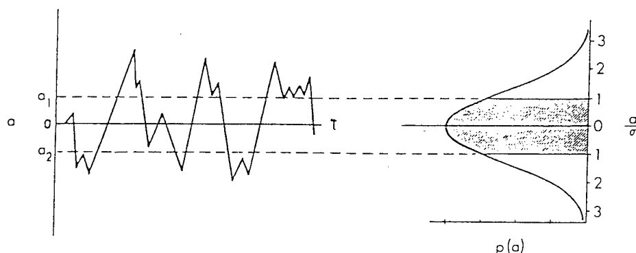
Figure 3.8. Gaussian Distribution of Random Vibration. From Ref. [6].
