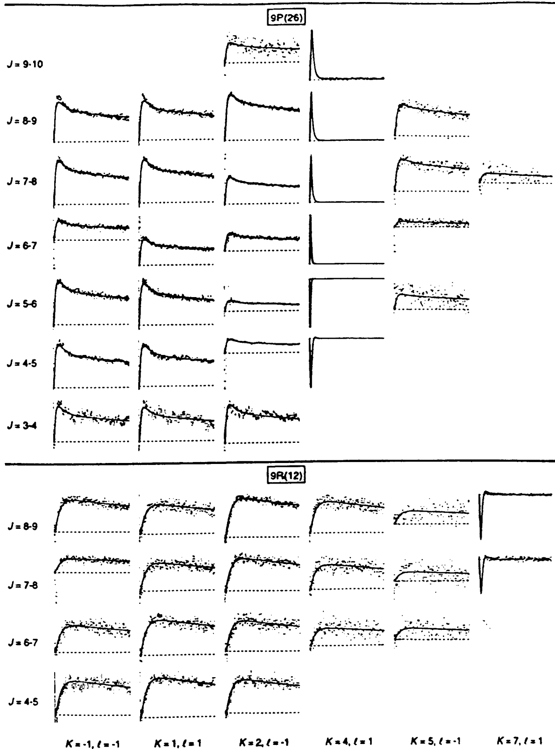
Figure III.B.2. Time resolved mm/submm probe responses for J,K transitions of the same symmetry species as the pumped transition in \text{CH}_3^{35}\text{Cl} . The 9P26 laser pumps the J = 6, K = 4, l = 1 energy level; The 9R12 laser pumps the J = 12, K = 7, l = 1 energy level.
