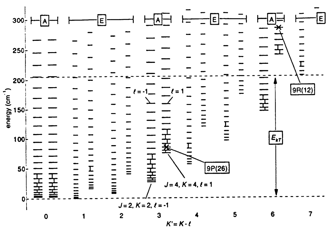
Figure III.B.1. Energy levels and symmetry species of \nu_6 vibrational state of \text{CH}_3\text{Cl} . The states pumped by the \text{CO}_2 laser are indicated in the figure.
