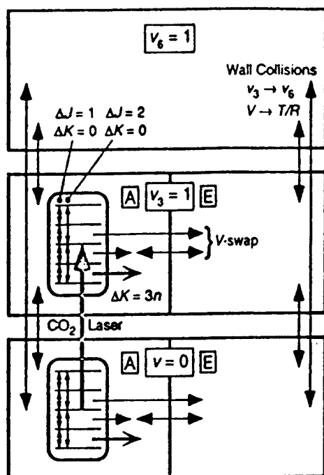
Figure III.B.3. Energy transfer model for methyl halides.
