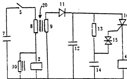
Figure 3.. Igniting circuit
